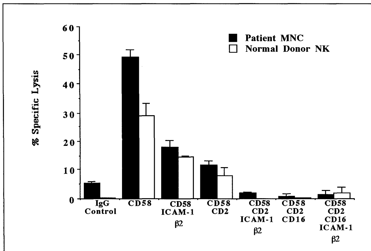
Figure 7. CD58 mediated ADCC decreases by blocking ICAM-1/β2 integrins, CD2 and CD16. Mononuclear cells from a patient receiving IL-2 therapy (E:T 20:1) or normal donor purified NK cells (E:T 10:1), without further IL-2 activation, were tested against the BT-20 breast cancer target in the presence or absence of various antibodies. CD58 significantly increased lytic activity compared to IgG control. In the presence of CD58 antibody, addition of antibodies to block ICAM-1, β2 integrin, CD2, and CD16 resulted in suppression of CD58 mediated ADCC.
