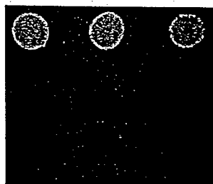
Terbinafine 1 µg/mL
