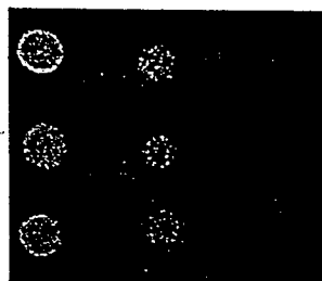
Clotrimazole 1.0 µg/mL
