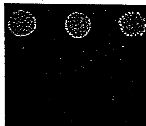
Fluphenazine 50 µg/mL
