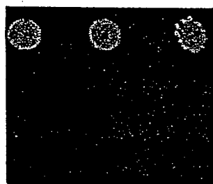
Tridemorph 0.03 µg/mL
