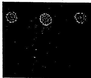
Cerulenin 1 µg/mL
