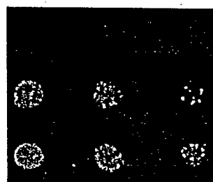
Nystatin 10 µg/mL
