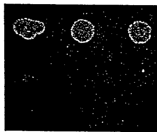
Cycloheximide 50 µg/mL
