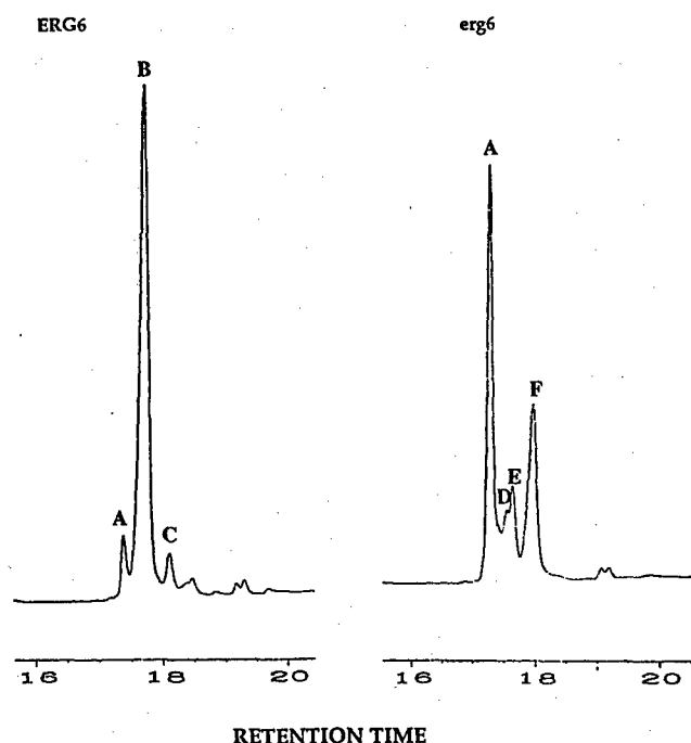
FIG. 5. GC of the sterols of the wild type and an erg6 strain of C. albicans . Peak A, zymosterol; peak B, ergosterol; peak C, fecosterol; peak D, cholesta-5,7,24-trien-3 \beta -ol; peak E, cholesta-7,24-dien-3 \beta -ol; peak F, cholesta-5,7,22,24-tetraen-3 \beta -ol.
