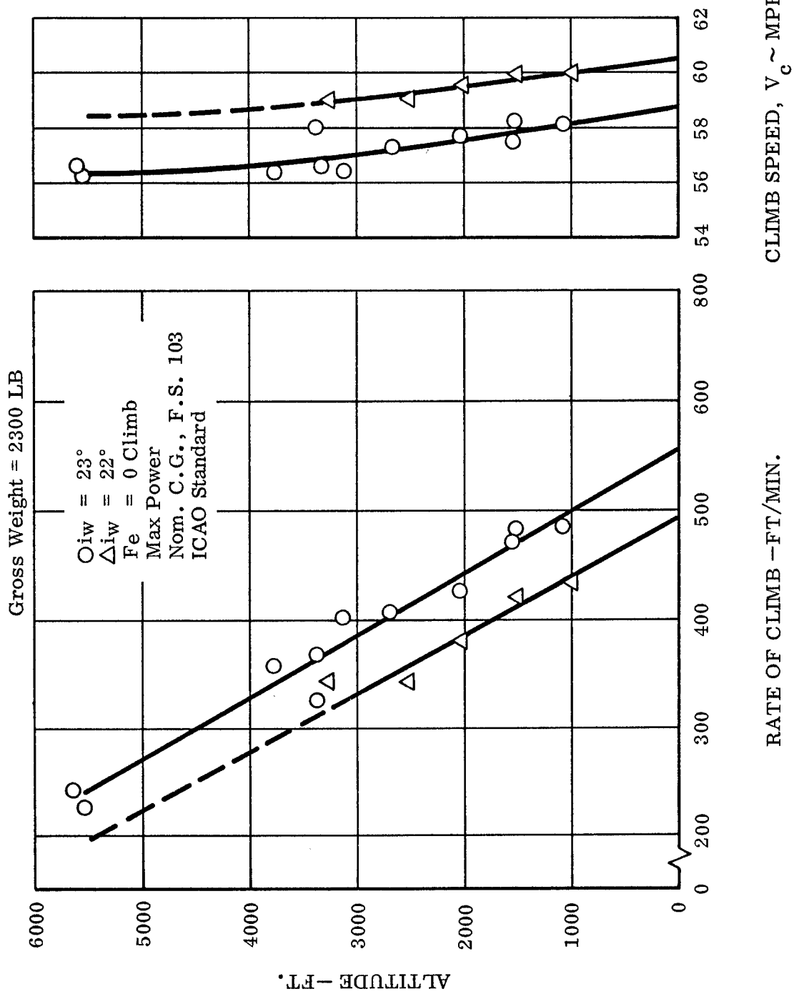
Figure 12. Rate of Climb Summary - 2300 Pound Gross Weight
