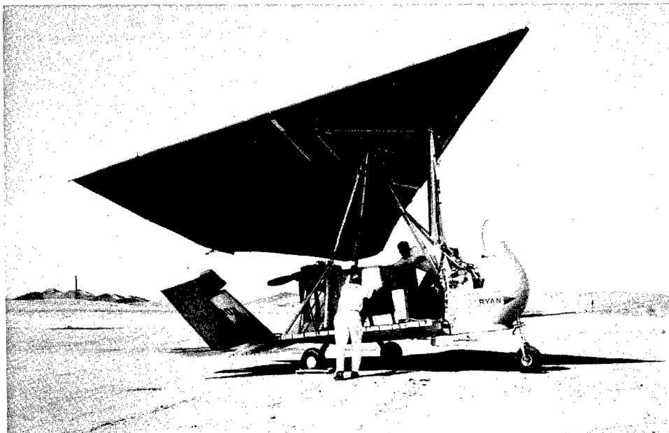
Figure 27. Maximum Height Propeller Blockage Configuration
