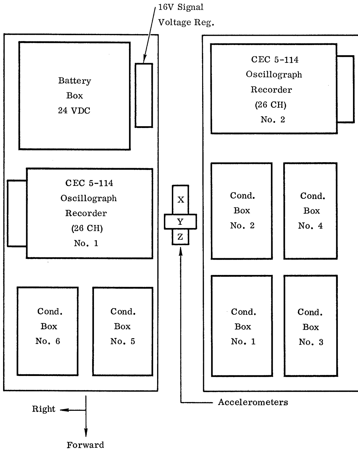
Figure 2. Recording Equipment
