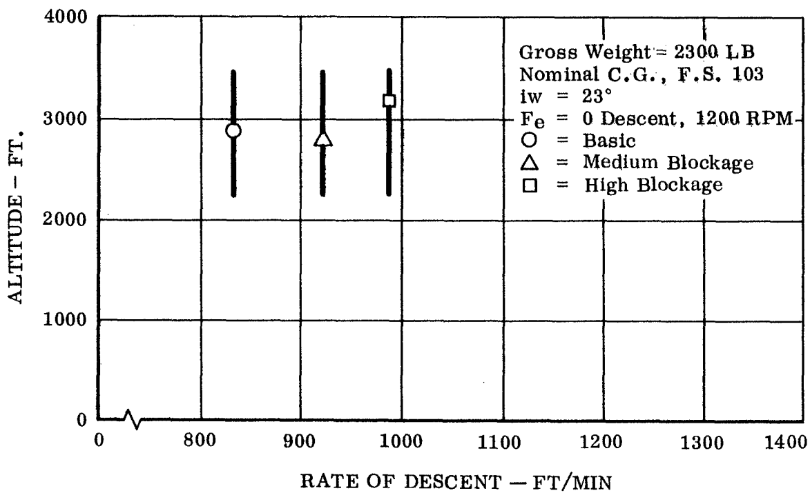
Figure 30. Propeller Blockage Effect on Rate of Descent
