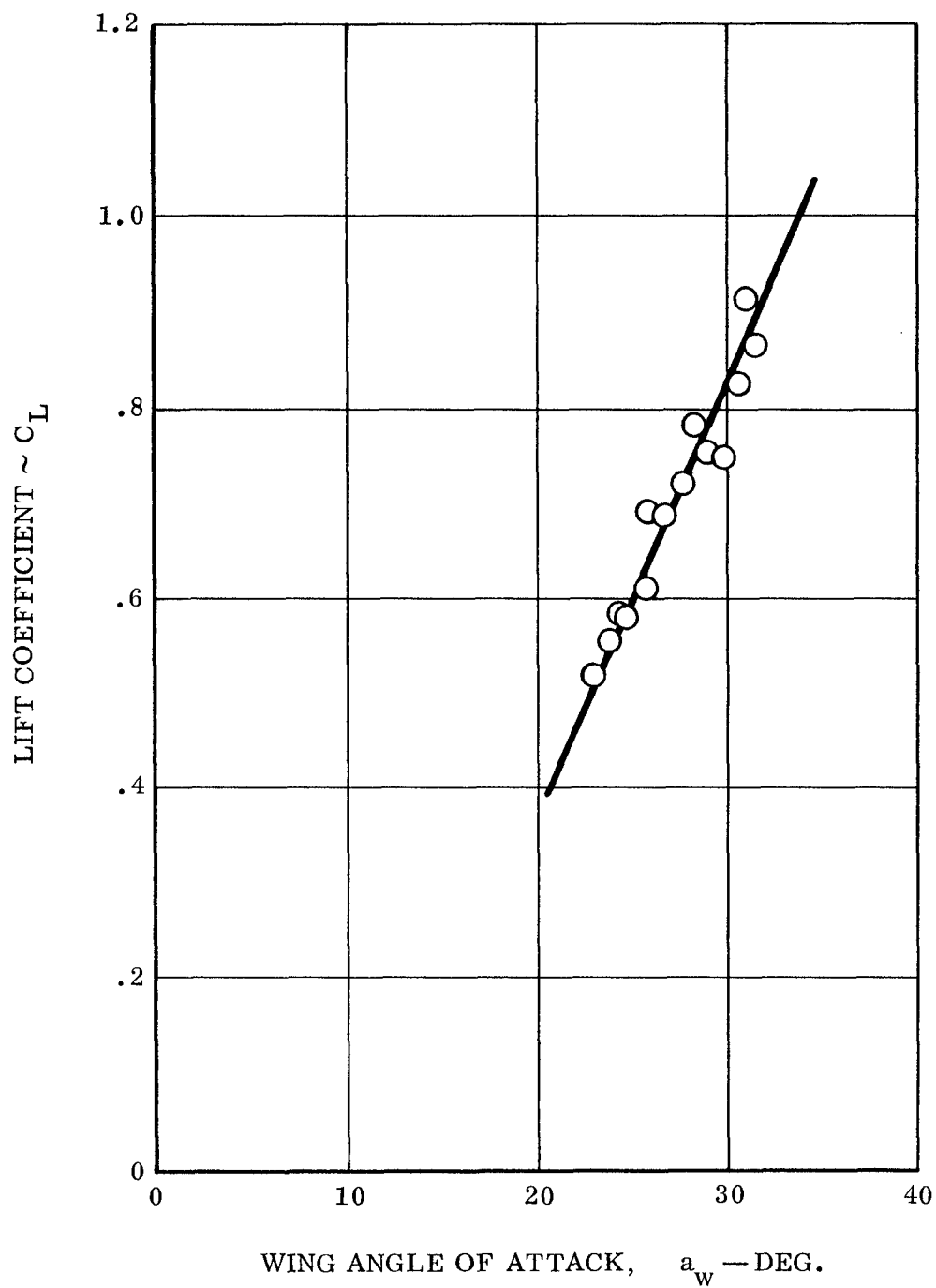
Figure 20. Lift Coefficient vs. Wing Angle of Attack
