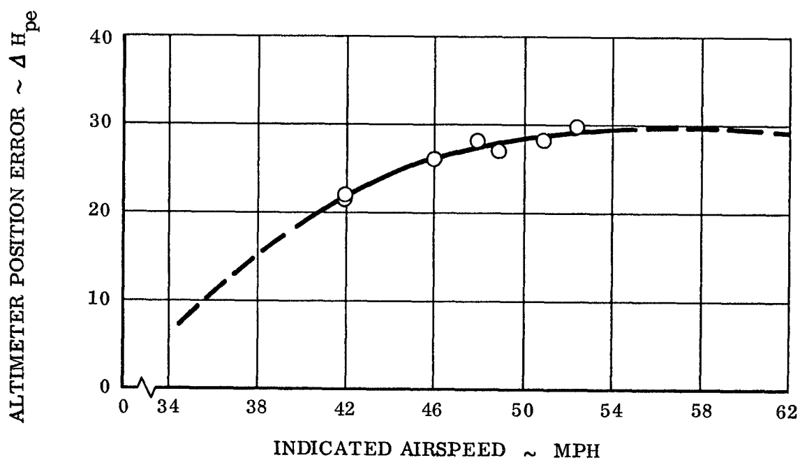
Figure 5. Altimeter Position Error Correction
