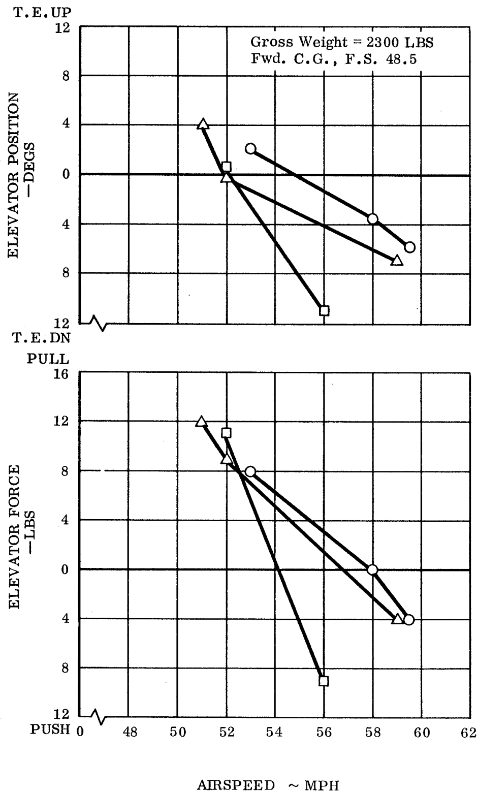
Figure 35. Static Longitudinal Stability - Fwd. C.G.
