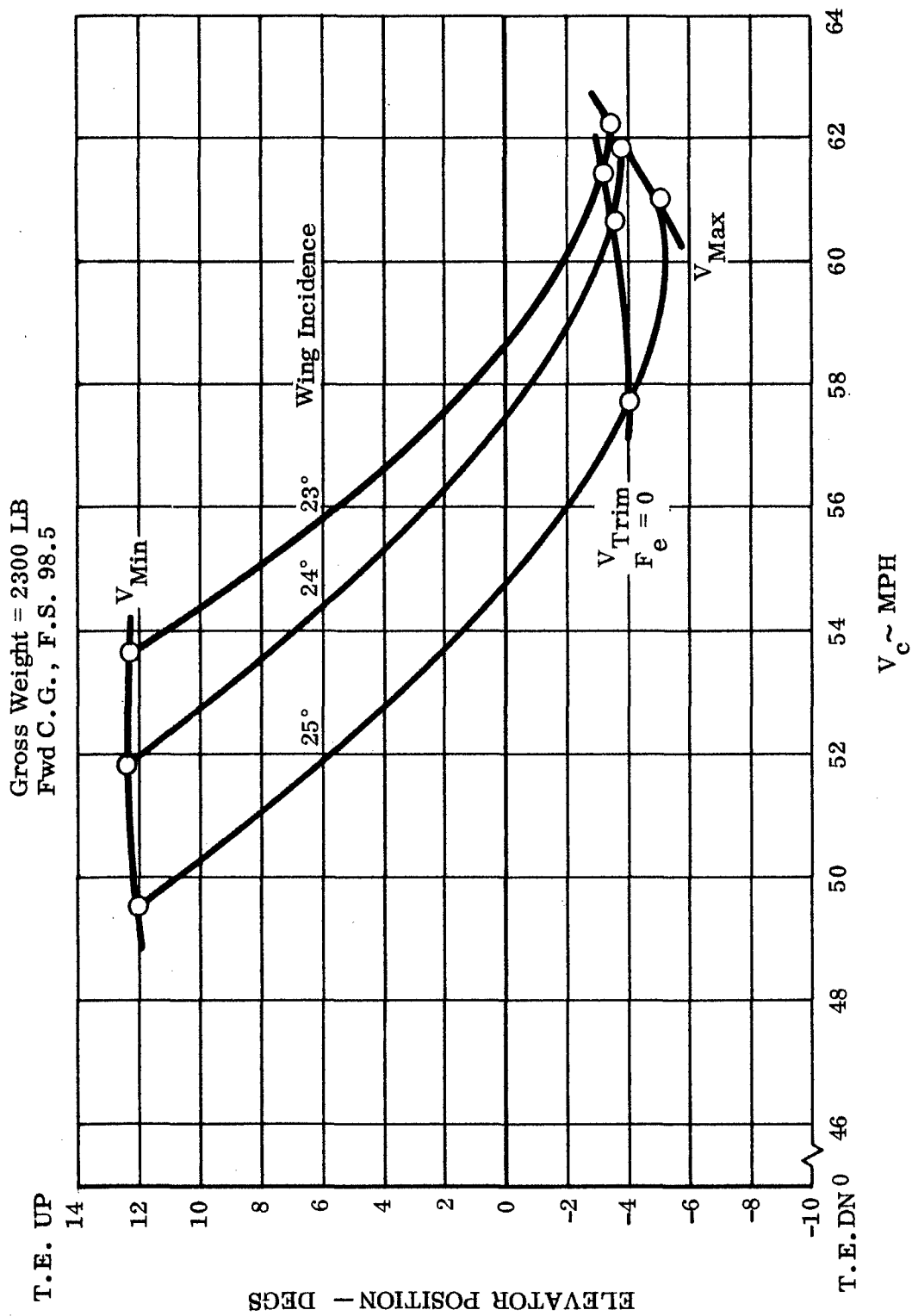
Figure 31. Elevator Angle vs. Velocity - Fwd. C.G. 2300 lb.
