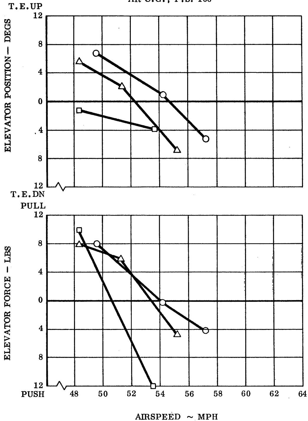
Figure 36. Static Longitudinal Stability - Aft. C.G.
