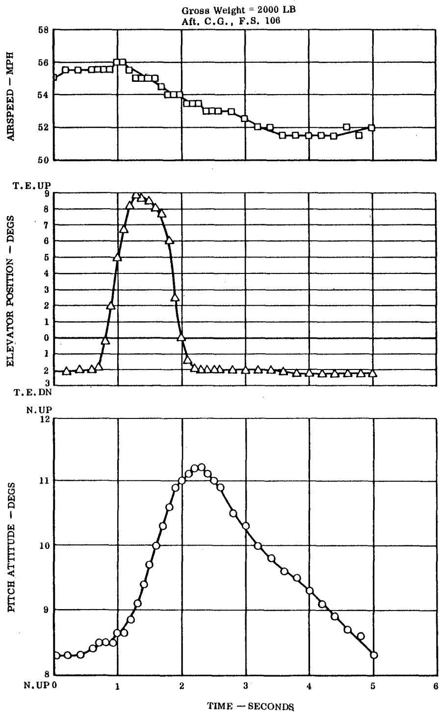
Figure 39. Short Period Dynamic Longitudinal Stability
