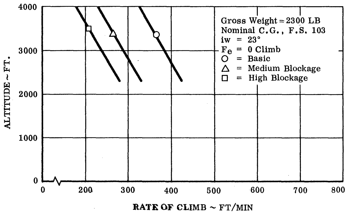
Figure 29. Propeller Blockage Effect on Rate of Climb
