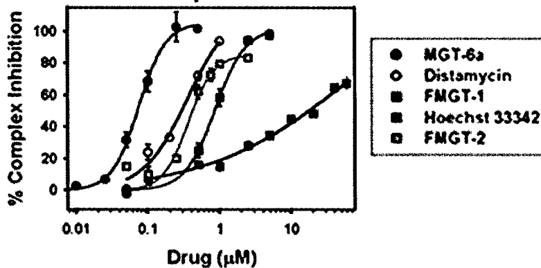
Figure 3: Effects of MGTs on TF/DNA complex formation in EMSAs.
