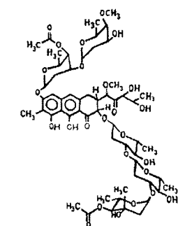
Chromomycin Binds G/C rich regions in the minor groove.
