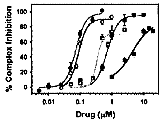
Figure 3: Effects of MGTs on TF/DNA complex formation in EMSAs.
