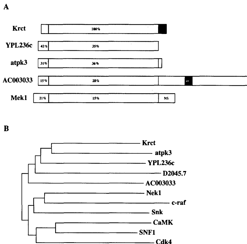
Figure 3. Krcr defines a novel subfamily of serine/threonine kinases. (A) Schematic representation of amino acid homology between Krcr , YPL236c , atpk3 and AC003033 . Results of the pairwise analysis using the ClustalW alignment program of the N-terminus, catalytic domain and C-terminus of Krcr , YPL236c , atpk3 , AC003033 and Mek1 are listed. The percentage identity to Krcr within each of these domains is indicated for each kinase. N-terminal, catalytic and C-terminal domains are indicated by open boxes, shaded boxes and black boxes, respectively. NS, not significant. (B) Phylogenetic tree illustrating the relationship of Krcr with other serine/threonine kinases in the GenBank database. Analysis and depiction of results was performed using the ClustalX multisequence alignment program and DendroMaker 4.0.
