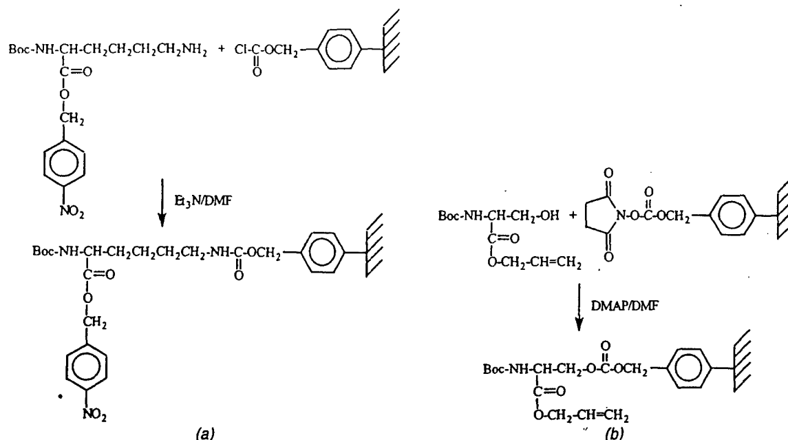
FIGURE 16.8. The p -nitrobenzyl and allyl esters can be used for carboxyl protection when attaching lysine (a) or serine (b) to resin supports.
