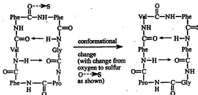
FIGURE 16.15. Conformational change accompanies thionation of a more sterically accessible Phe-Phe amide to form the Phe \psi [CSNH]Phe-containing pseudopeptide. This leads to a new hydrogen bonded structure with thioamide participation as a donor. Nevertheless all structures displayed significant conformational heterogeneity.
