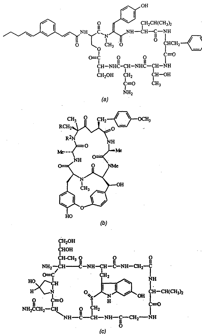
FIGURE 16.1. Examples of naturally occurring cyclic peptides with amide and nonamide groups in the ring. (a) Tachykinin antagonist from Streptomyces violaceonigen ; (b) structure of Bouvardins; (c) structure of the mushroom-derived toxin \alpha -amanitin.
