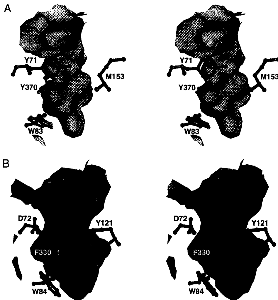
Fig. 3. Stereoviews of the active-site gorges of DmACHE and TcACHE . The accessible surfaces are rendered semi-transparent using the program DINO (Philippsen, 2000). Residues that significantly influence the trajectory and volume (see text) are shown as ball and stick. A: The active-site gorge of DmACHE . B: The active-site gorge of TcACHE . Residue Phe330 is on the far side of the surface.
