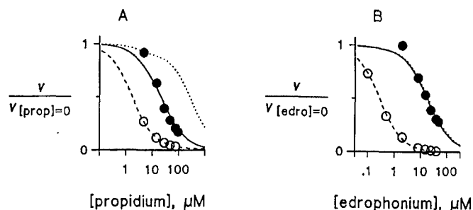
Fig. 7. Determination of the relative affinity of huprine X in the propidium-AChE complex (A) or the edrophonium-AChE complex (B) by inhibition of substrate hydrolysis. AChE ( \circ , 25 pM; \bullet , 1200 pM) was incubated without ( \circ ) or with ( \bullet ) huprine X (4 nM) and the indicated concentration of propidium or edrophonium for 6 h at 23°C, and a 2.9-ml aliquot was mixed with 100 \mu\text{l} of DTNB and 12 \mu\text{l} of acetylthiocholine to give final concentrations of 0.33 mM DTNB and 20 \mu\text{M} acetylthiocholine. Points represent v observed over a 2- to 5-min interval normalized by the corresponding v obtained at the same [huprine X] in the absence of propidium ( v_{[\text{prop}]=0} ) or edrophonium ( v_{[\text{edro}]=0} ). Lines correspond to normalized v obtained by fitting the experimental data to a complete nonequilibrium reaction scheme with the program SCOP, with kinetic rate constants previously determined for acetylthiocholine and propidium or edrophonium (Eastman et al., 1995; Szegeletes et al., 1999) and those in Table 1 for huprine X. The dashed lines correspond to the absence of huprine X and the solid lines, to 4 nM huprine X. The dotted lines correspond to the curves calculated when no ternary complex forms ( 1/K_{112} = 0 ). Based on data with 4 nM huprine X as well as with 1 and 2 nM huprine X (data not shown) with both propidium and edrophonium, the procedure in A gave K_{12} = 1.4 \mu\text{M} for propidium, K_{11} = 20 \text{ pM} for huprine X, and K_{112}/K_{11} = 17 \pm 3 . The procedure in B gave K_{12} = 0.2 \mu\text{M} for edrophonium, K_{11} = 29 \text{ pM} for huprine X, and K_{112}/K_{11} > 1000 . Lines also were fitted with the much simpler analysis scheme in eq. 3, which required the approximations that v reflects the true second-order rate constant, that the free huprine X concentration remains unchanged through the entire range of propidium or edrophonium concentrations, and that no slow reequilibration occurs in the presence of substrate. Although these approximations held only approximately at best, ratios of K_{112}/K_{11} of 12 \pm 2 with propidium and >200 with edrophonium were in reasonable agreement with those from the SCOP program.
