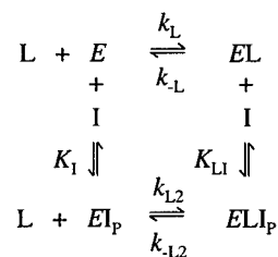
SCHEME 3
