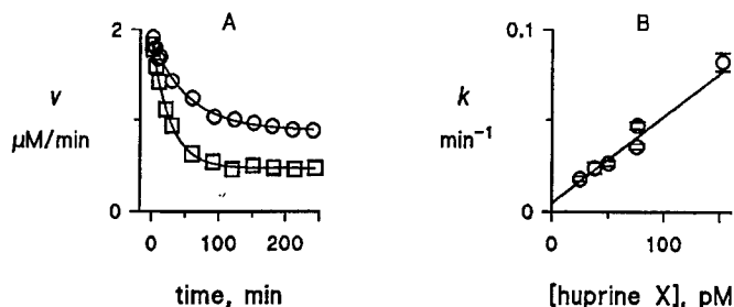
Fig. 5. Association and dissociation rate constants for hupeirine X and AChE. A, progressive inhibition of AChE (6 pM) with time as hupeirine X binding approached equilibrium was measured by removing 1-ml aliquots of the reaction mixture and immediately adding DTNB and the substrate acetylthiocholine for assay as outlined in Experimental Procedures . Hydrolysis rates v obtained with 25 (○) and 75 (□) pM hupeirine X were fitted to eq. 4 to obtain a value of k for each curve. B, values of k obtained at several concentrations of hupeirine X as in A were plotted against [\text{hupeirine X}] . Although the plot was nearly linear, the concentration of hupeirine X in some cases was not sufficiently in excess of the concentration of AChE to justify analysis with eq. 5. The SCoP fitting program was applied directly to all the association rate data (Szegeletes et al., 1998) to obtain k_i = 440 \pm 30 \mu\text{M}^{-1} \text{min}^{-1} and k_{-1} = 0.009 \pm 0.003 \text{ min}^{-1} .
