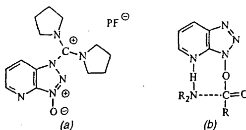
FIGURE 16.12. Structure of the condensing agent HAPyU as the guanidinium N-oxide in the solid state (a) as contrasted to the postulated reactive intermediate in solution during coupling where the adjacent 7-azabenzotriazole additive (b) can assist in amide bond formation via intramolecular base catalysis.
