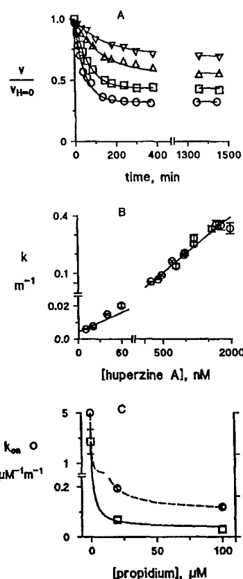
FIGURE 6: Determination of association and dissociation rate constants for huperzine A with both AChE and the AChE-propidium complex. Ligand binding was assumed to occur according to Scheme 3. Part A: Association reactions were initiated by mixing AChE (150 pM) with huperzine A (○) 60 nM, (□) 40 nM, (Δ) 20 nM, (▽) 10 nM and 20 \mu M propidium, and aliquots were assayed at the indicated times as outlined in the Experimental Procedures. Assay points v were normalized to a control 150 pM AChE activity with 20 \mu M propidium but without huperzine A ( v_{H=0} ) and fitted to eq 2 to obtain a value of k for each curve. Part B: Values of k obtained from both part A and additional measurements at 20 \mu M propidium were plotted against the huperzine A concentration according to eq 3 to obtain k_{on} = 0.195 \pm 0.007 \mu\text{M}^{-1}\text{m}^{-1} and k_{off} = 0.0043 \pm 0.0006 \text{ m}^{-1} . In the absence of propidium, k_{on} = k_L and k_{off} = k_{-L} and a similar analysis was used to obtain the estimates of k_L and k_{-L} in Table 3. Part C: Values of k_{on} and k_{off} were plotted against the propidium concentration according to eqs 4a,b. The above k_L value was fixed in eq 4a, and the k_{on} estimates at 20 \mu M and 100 \mu M propidium were then fitted to this equation to obtain the estimates of k_{L2} and K_I in Table 3. Equation 4b was rearranged to the form k_{off} = (k_{-L} + W[I]/K_I)/(1 + W[I]/K_I k_{-L2}) . The previously obtained k_{-L} , K_I , and W = k_{L2}K_L were then fixed, and this equation was used to fit the k_{-L2} value in Table 3.
