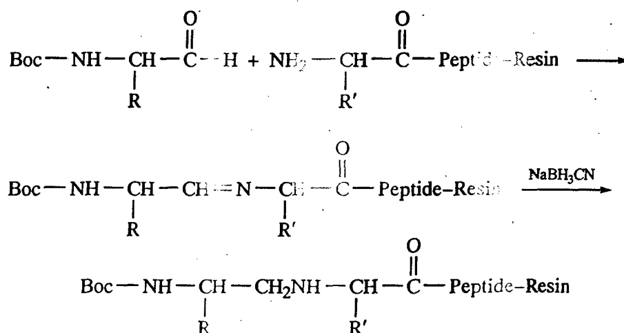
Scheme 5. Solid phase synthesis of a \psi[\text{CH}_2\text{NH}] pseudopeptide.
