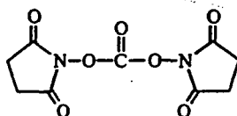
N,N' -disuccinimidyl carbonate (DSC)
