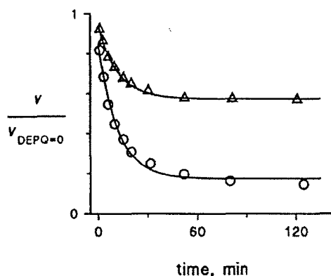
FIG. 4. Inactivation of the residual activity of the fasciculin-AChE complex by DEPQ at two ratios of the DEPQ to AChE concentrations. Erythrocyte AChE at 0.16 nM (○) and 80 nM (△) was incubated for 10 min with fasciculin at 50 nM (○) and 500 nM (△), and inactivation was initiated by the addition of DEPQ to a final concentration of 1.4 nM. Aliquots were assayed at the indicated times as outlined under "Experimental Procedures." Assay points v were normalized to corresponding control residual activities with fasciculin but without DEPQ ( v_{\text{DEPQ}=0} ) and fitted to Equation 7 (lines) to obtain a value of k for each curve.
