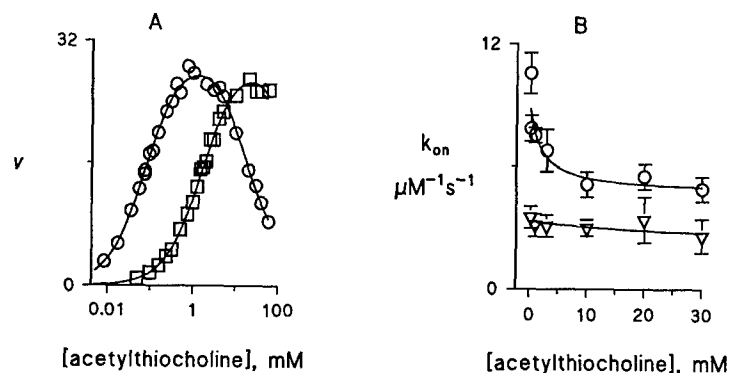
Figure 2. Acetylthiocholine binding to the peripheral site of human AChE (4). Panel A. Substrate inhibition with acetylthiocholine. Initial velocities v ( \mu\text{M}/\text{min} ) were measured with recombinant wild type ( \circ ) or D74G ( \square ) AChE (80 pM). Lines were fitted with the SCoP program. Panel B: Inhibition of fasciculin 3 binding by acetylthiocholine. Association rate constants k_{\text{on}} for fasciculin 3 were measured with recombinant wild type ( \circ ) or D74G ( \nabla ) AChE. Lines were obtained by fixing K_S at the value obtained from substrate inhibition before fitting.
