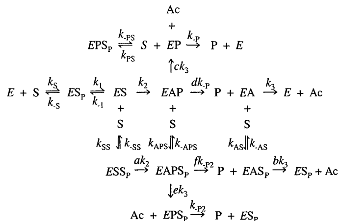
SCHEME 5
