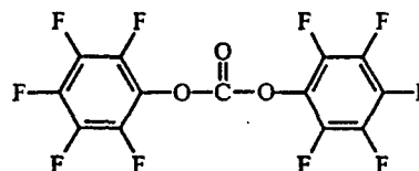
Di-(pentafluorophenyl)carbonate
