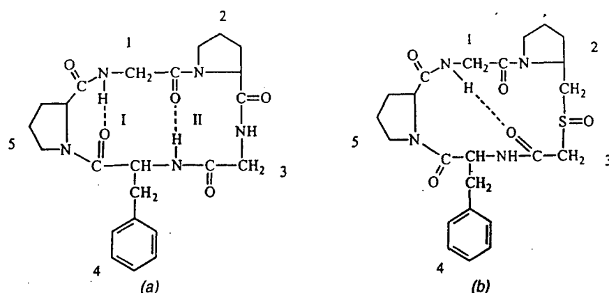
FIGURE 16.14. Structure of a cyclic pentapeptide (a) and a cyclic \psi[\text{CH}_2\text{S}] pseudopentapeptide (b) showing shift of intramolecular \beta -turn.
