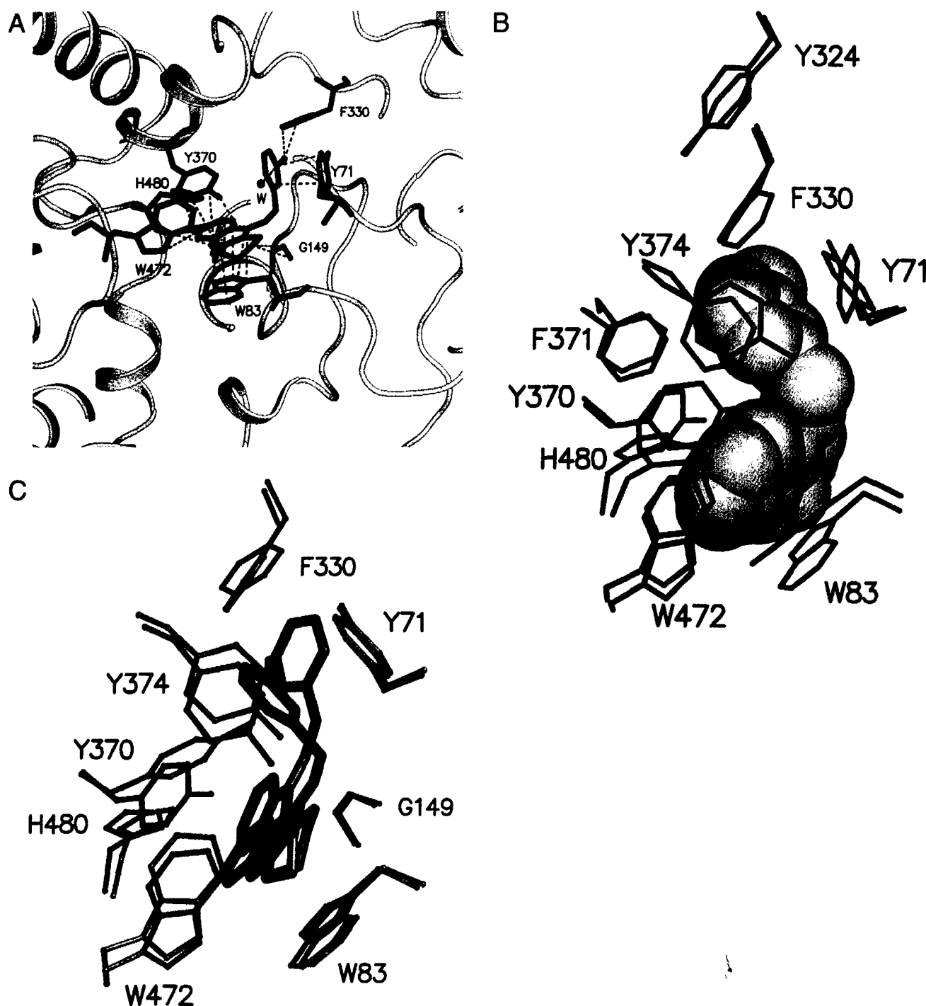
Fig. 7. Representations of interactions of Dm AChE with ZAI and ZA. A: Dm AChE residues (turquoise) interacting with ZAI (red) with distances <3.8 Å. B: Nine aromatic residues in native Dm AChE (black) change their conformation when ZAI (red), shown with its van der Waals surface, binds to Dm AChE. C: Overlap of ZAI complex (red) and ZA complex (turquoise). The inhibitors are shown as thick sticks, and the side chains of the principal residues with which they interact as thin sticks.
