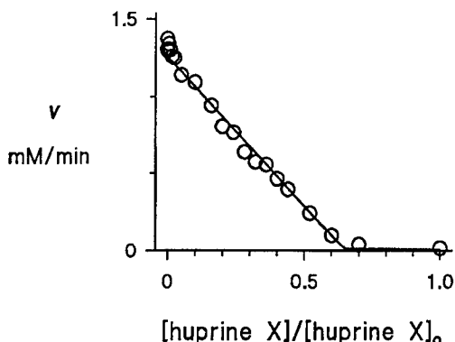
Fig. 3. Titration of recombinant human AChE with huprine X. Each point represents one mixture with a final concentration of 1.21 \mu M AChE and the indicated concentration of huprine X relative to the maximal concentration [huprine X] 0 incubated for 3 h at 23°C. Aliquots (10 \mu l) were then diluted 300- to 15,000-fold into assay solution containing 0.5 mM acetylthiocholine. Points represent observed v (mM/min) normalized to a 300-fold dilution into assay solution. The line was fitted to the points in a nonequilibrium analysis with the program SCoP, assuming that huprine X interacted with AChE according to Scheme 1 with rate constants k_1 = k_{AI} and k_{-1} = k_{-AI} given in Fig. 5. The fitted value of [huprine X] 0 = 1.87 \mu M was used to determine an apparent extinction coefficient for huprine X.
