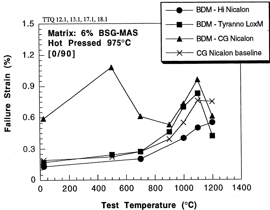
FIGURE 107. FLEXURAL STRENGTH AND FAILURE STRAIN FOR AS PROCESSED FAST FRACTURE TESTED BDM MICA COATED SiC FIBER CMCs
