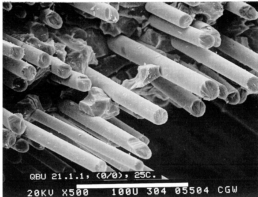
(A) 25°C FRACTURE SURFACE SHOWING FIBER PULLOUT
