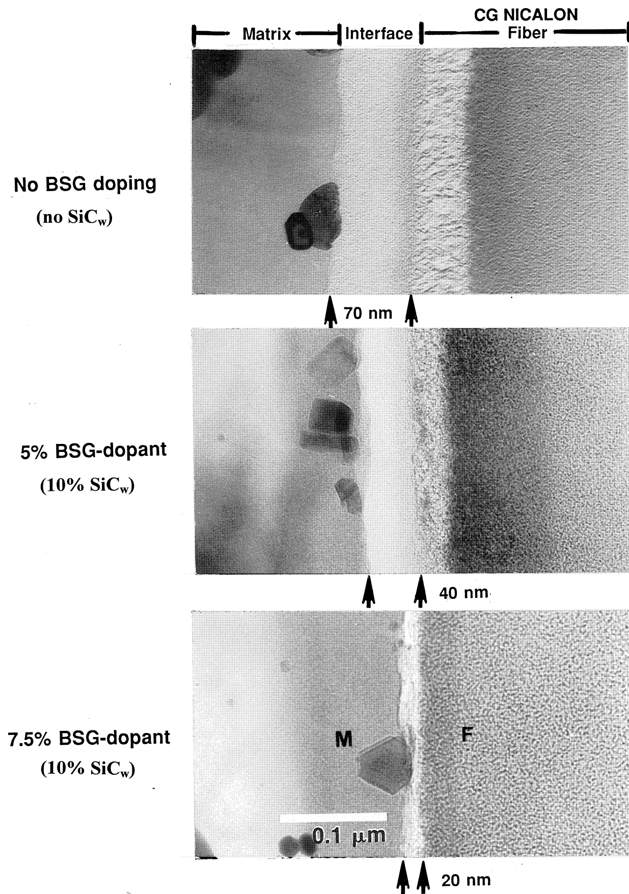
FIGURE 8. TEM THIN FOIL VIEWS OF INTERFACE IN Nicalon/MAS CORDIERITE COMPOSITES WITH VARYING AMOUNTS OF BSG-DOPING
