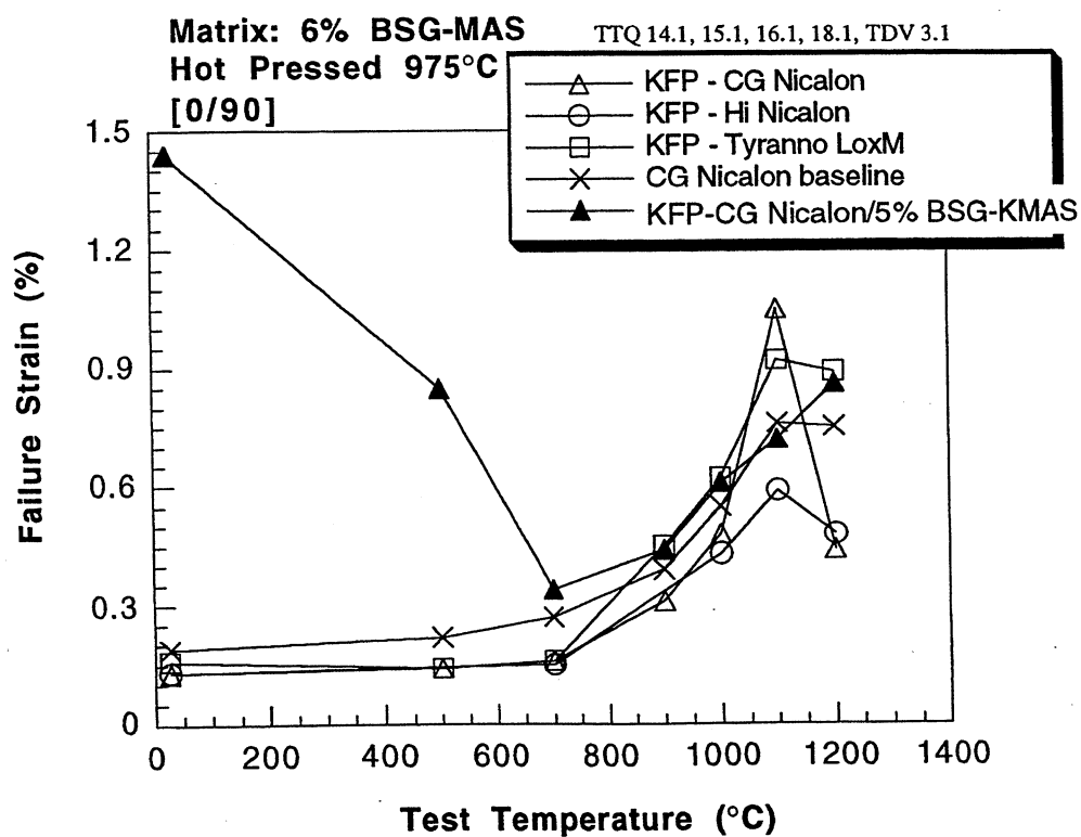
FIGURE 109. FLEXURAL STRENGTH AND FAILURE STRAIN FOR AS PROCESSED, FAST FRACTURE TESTED, KFP MICA COATED SiC FIBER CMCs
