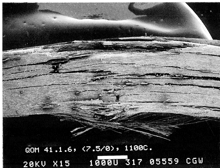
(B) 1100°C EXTENSIVE SHEAR DEFORMATION OF BEAM WITH LITTLE TENSILE PROPAGATION. NOTE COMPRESSIVE FAILURE AND SLIGHT PERMANENT DEFORMATION
