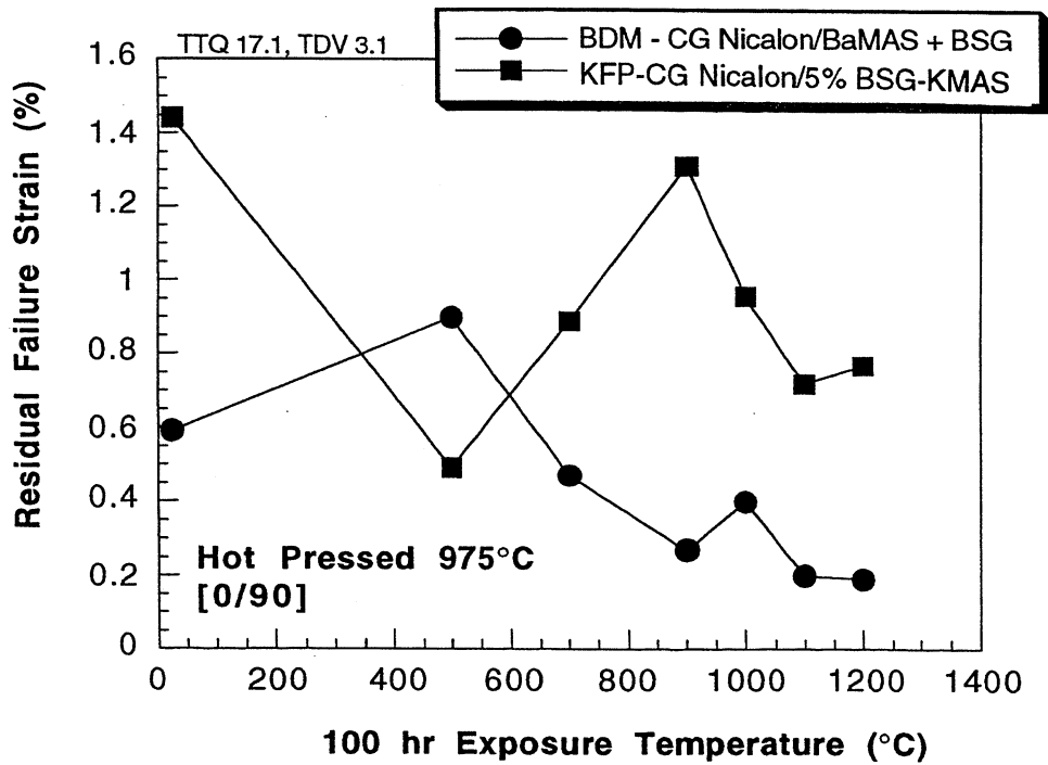
FIGURE 114. LONG TERM UNSTRESSED OXIDATION FLEXURAL STRENGTH AND FAILURE STRAIN FOR THE TWO MOST PROMISING MICA INTERFACE CMCs
