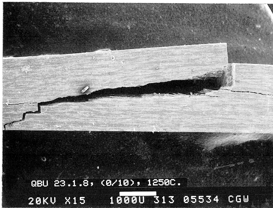
(C) 1250°C: NO PERMANENT DEFORMATION
