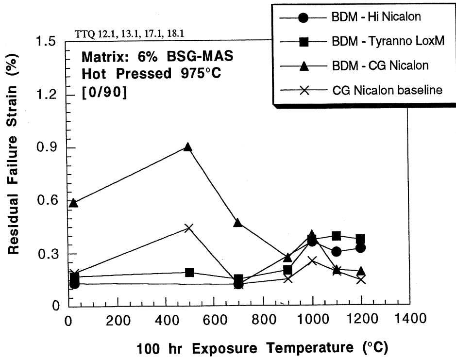
FIGURE 111. Residual Flexural Strength and Failure Strain After Thermal Exposure for BDM Mica Coated SiC Fiber CMCs.
