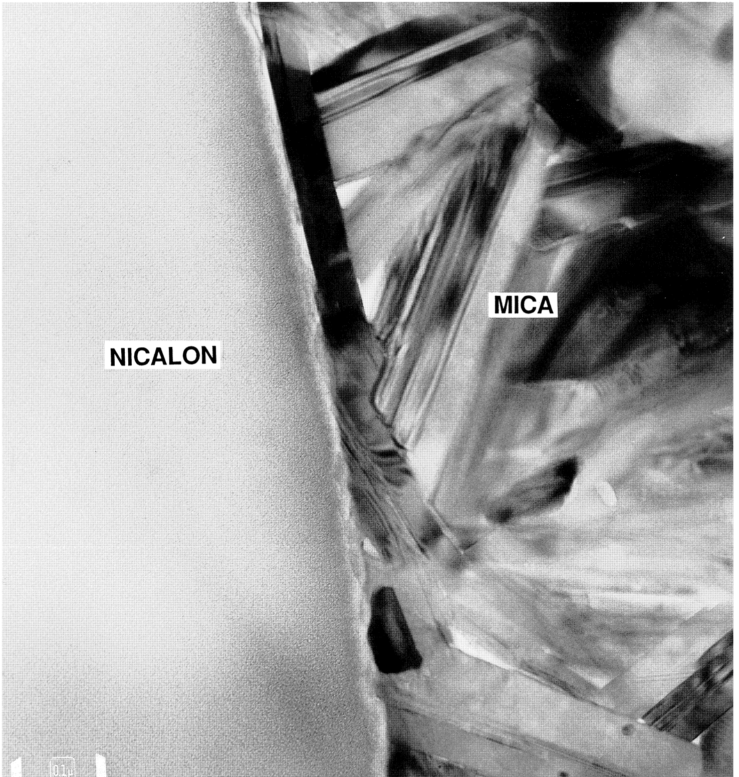
FIGURE 102. TEM THINFOIL OF MICA-Nicalon/6% BSG-MAS CMC (TTQ 11.1)
