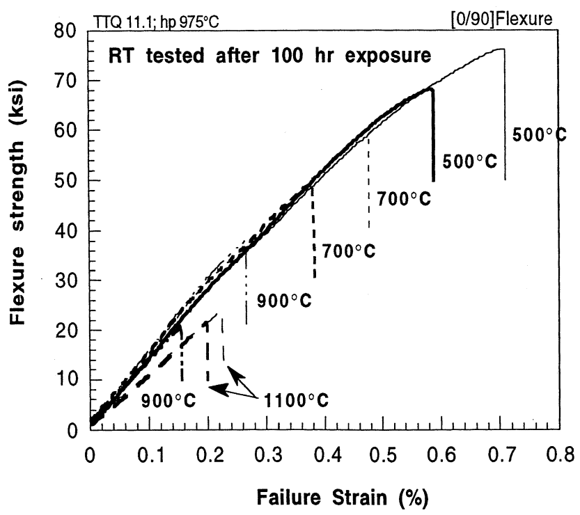
FIGURE 112. STRESS-STRAIN BEHAVIOR FOR (3s) BDM MICA COATED CG Nicalon/6% BSG-MAS CMCs AFTER LONG TERM THERMAL EXPOSURE
