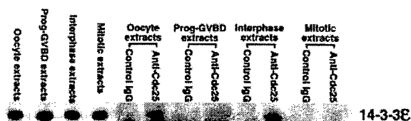
Fig. 1. Xenopus Cdc25 binds to 14-3-3 \epsilon in oocyte extracts and interphase egg extracts. Extracts were prepared from untreated Xenopus oocytes, oocytes undergoing progesterone-induced GVBD, Xenopus eggs arrested in mitosis or Xenopus eggs released into interphase. Two microliters of each extract was subjected to SDS-PAGE and immunoblotted with anti-14-3-3 \epsilon antibody (first four lanes). In addition, 60 \mu l of each extract was immunoprecipitated with either control IgG or anti-Cdc25 sera. Immunoprecipitated proteins were analyzed by SDS-PAGE followed by Western blotting with anti-14-3-3 \epsilon antibody. 14-3-3 \epsilon coprecipitated with Cdc25 only in the untreated oocyte and interphase egg extracts.
