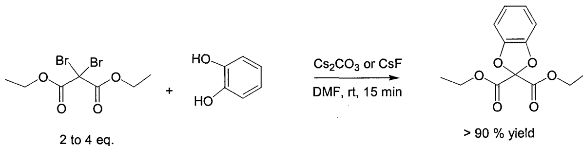
Figure 3. Catechol derivative of ethyl \alpha,\alpha -dibromomalonate.
