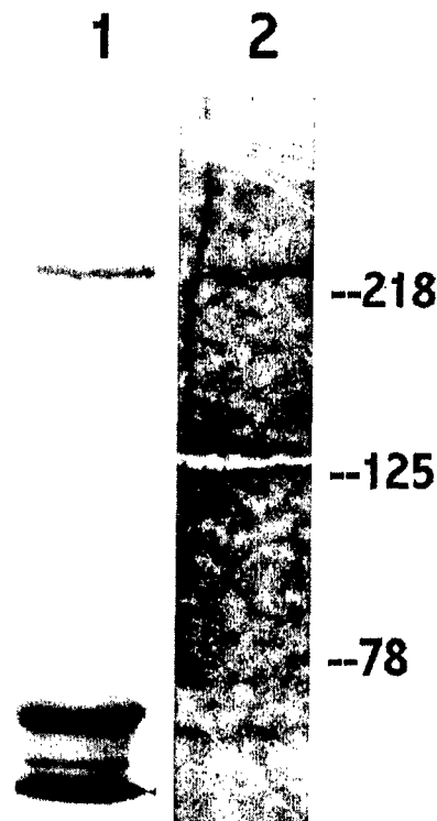
Fig. 3. C75 labels FAS. SDS/PAGE and fluorography of SKBr3 cell lysate after 4 h exposure of cells to [ ^3\text{H} ]C75 [ 5\text{ }\mu\text{g/ml} ]. Lane 1, whole cell lysate. Lane 2, FAS immunoprecipitation. Note the labeling of the approximately 250-kDa band, which represents human FAS.
