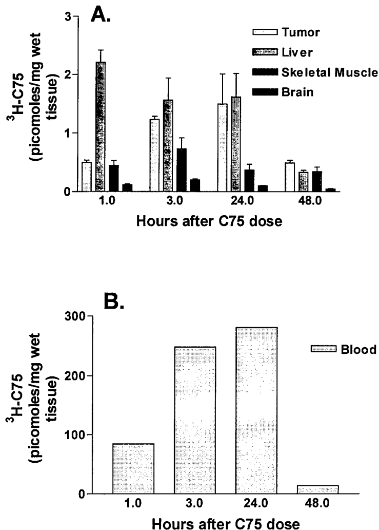
Figure 2A and B. Tissue distribution of [ ^3\text{H} -C75] in the MCF7 xenograft and normal tissues. Athymic nude mice with subcutaneous MCF7 xenografts were treated with 0.6 mg of [ ^3\text{H} -C75] i.p. in 200 \mu\text{l} of RPMI vehicle. At the indicated times, animals were sacrificed and 1-2 mg of tissues and 1 \mu\text{l} of blood were removed and counted for ^3\text{H} . Note the rapid rise in blood and liver levels except for brain. Tumor levels remain elevated above liver after 48 h. Error bars represent standard error of the mean.
