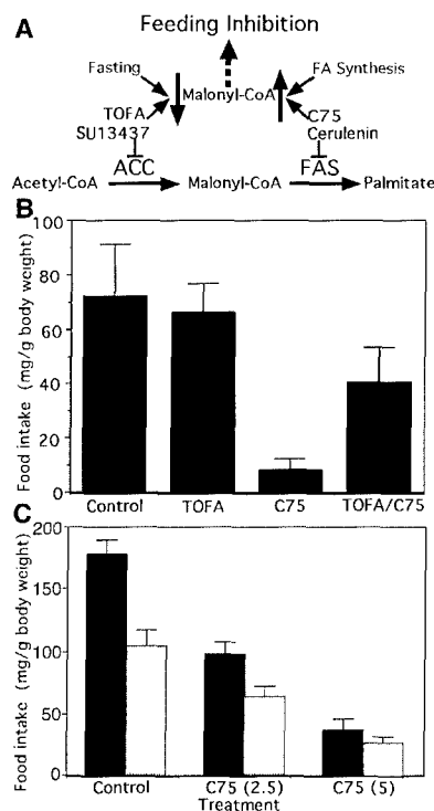
Fig. 4. Feeding regulation by malonyl-CoA. (A) Model of feeding regulation by inhibitors of FAS via malonyl-CoA. (B) BALB/c mice were anesthetized with metofane and received ICV injections of 2 \mu\text{g} of TOFA or dimethyl sulfoxide vehicle. After 2 hours recovery, mice received ip injections of C75 (15 mg/kg) or of RPMI vehicle and were monitored for total food intake over 2 hours. (C) Mice were anesthetized and received ICV injections of RPMI (2 \mu\text{l} ) or of C75 (2.5 or 5 \mu\text{g}/\mu\text{l} ), and food intake was monitored over 2 and 4 hours (gray and solid bars, respectively). (B) and (C) combine results from three experiments with n = 3 mice for each experiment (nine mice total).
