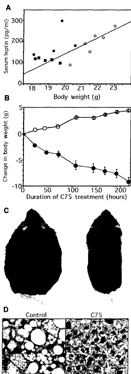
Fig. 3. Leptin independent of action C75. (A) Male BALB/c mice ( n = 5 ) were fasted (●) or received ip injections of RPMI (○) or of C75 (30 mg/kg) (■) and were free-fed for 24 hours, weighed, and then exsanguinated. Serum leptin was determined with a Quantikine murine leptin enzyme-linked immunosorbent assay (R&D Systems, Minneapolis, Minnesota) and plotted against total body weight. (B) Male ob/ob (C57BL/6J \Delta^{\text{Hsd-Lep}^{\text{ob}} ) (Harlan, Oxon, England) mice ( n = 3 ) were treated with ip injections of RPMI (○) or of C75 (22 mg/kg) (●) every third day (representative of two experiments). Change in body weight is displayed as mean \pm SEM. (C) Representative vehicle- (left) and C75-treated (right) mice from (B) after 14 days of treatment. (D) Livers from vehicle- (control) and C75-treated mice were formalin fixed and paraffin embedded. Tissue sections (4 \mu\text{m} ) were stained with hematoxylin and eosin. Bar, 50 \mu\text{m} .
