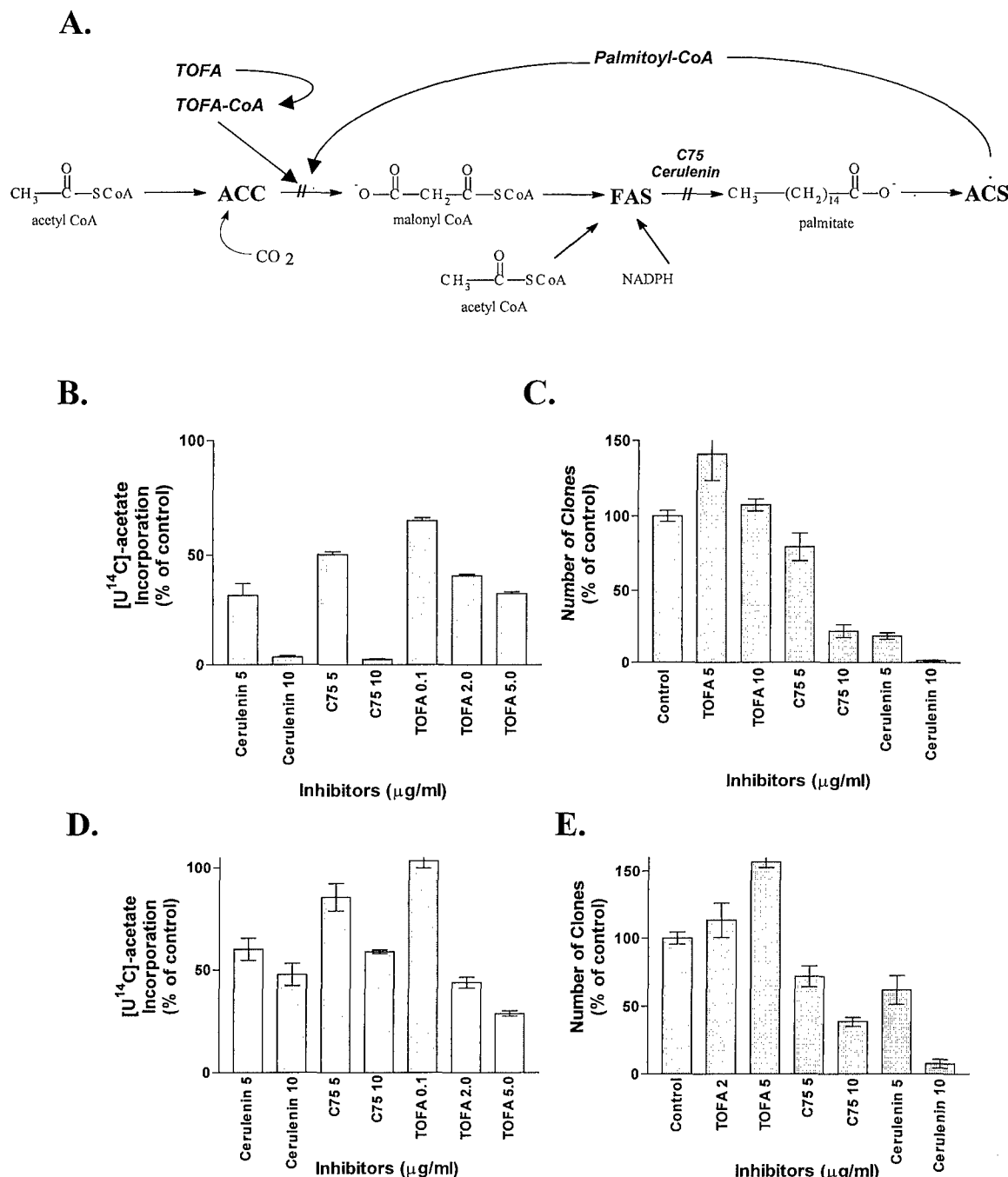
Fig. 1. Inhibitors of the FA synthesis pathway. A, schematic representation of the FA synthesis pathway showing the specificity of cerulenin and C75 for FAS and of TOFA for ACC. The three FA synthesis inhibitors reduced FA synthesis activity (incorporation of [ ^{14} C]acetate into extractable lipids) by comparable amounts in SKBR3 breast carcinoma cells (B) and in MCF7 breast carcinoma cells (D). The cytotoxic activity of the three FA synthesis inhibitors was determined by clonogenic assay in the dose range for FA synthesis inhibition. A 6-h exposure to cerulenin or C75 reduced the clonogenic fraction of SKBR3 breast carcinoma cells (Student's t test, P = 0.0002 for C75, P < 0.0001 for cerulenin; C) and MCF7 breast carcinoma cells ( P = 0.0004 for C75, P < 0.0001 for cerulenin; E), whereas TOFA did not.
