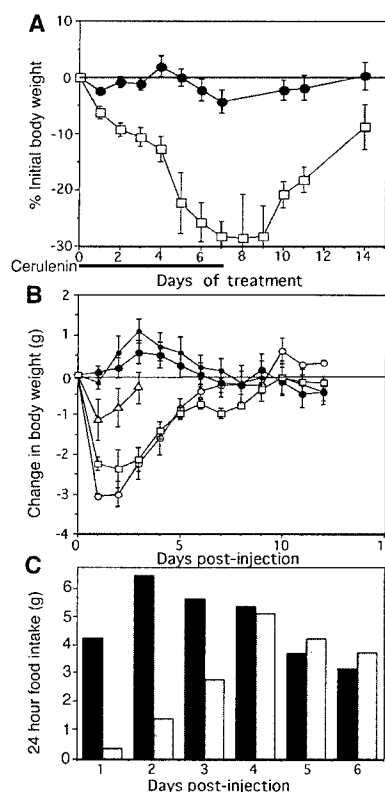
Fig. 1. Effect of FAS inhibitors on body weight and food intake. (A) Female BALB/c mice were treated by ip injection of RPMI medium vehicle (●) or cerulenin at 60 mg/kg/day (□) for 7 days. (B) Female BALB/c mice were given a single ip injection of C75 at doses of 7.5 (Δ), 15 (○), or 30 (□) mg/kg or (●) RPMI vehicle. Mice were housed in metabolic cages and monitored for body weight, food and water intake, and urine and feces output. Mean change from initial body weight is expressed \pm SEM. (C) Total food intake per day by mice treated with vehicle (black bars) or C75 (15 mg/kg) (gray bars) from (B). Experiments consisted of three animals per group and were repeated four times.
