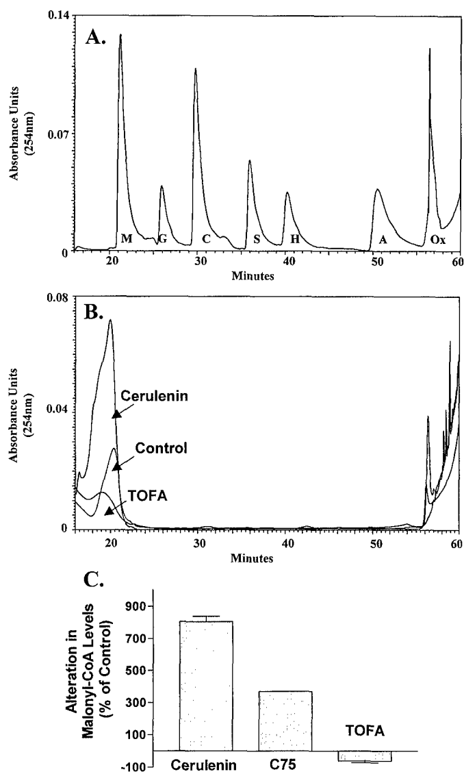
Fig. 2. Effects of the FA synthesis inhibitors on malonyl-CoA levels. Chemical standards (A) and acid soluble extracts of MCF7 breast carcinoma cells (B) were resolved by reversed-phase HPLC for quantitation of malonyl-CoA. Changes in intracellular malonyl-CoA content after exposure to the three FA synthesis inhibitors are shown in C. Assays were performed in triplicate.
