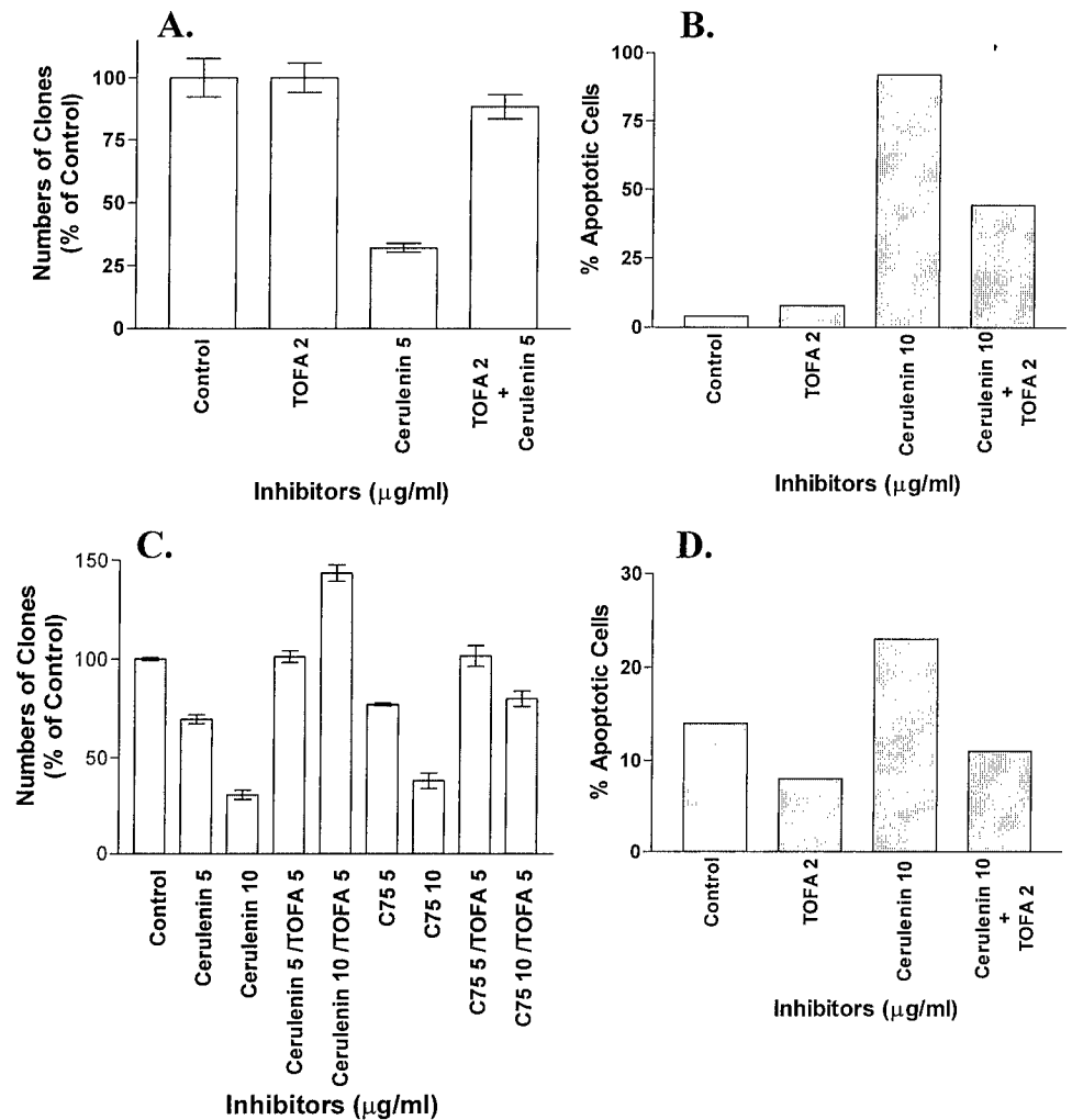
Fig. 3. ACC inhibition rescued the cytotoxic effects of FAS inhibition in breast cancer cells. A , pretreatment with TOFA rescued SKBR3 cells from cerulenin cytotoxicity as determined by clonogenic assays (Student's t test, P = 0.001 ). C , similarly, TOFA reduced both cerulenin and C75 cytotoxicity in MCF7 cells ( P = 0.0016 for C75, P < 0.0001 for cerulenin). Using merocyanine 540 staining as an indicator of apoptosis, TOFA rescued both SKBR3 cells ( B ) and MCF7 cells ( D ) from cerulenin cytotoxicity.
