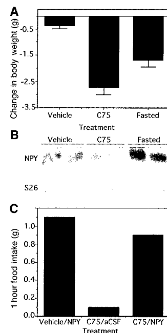
Fig. 2. Role of NPY in regulation of feeding by C75. (A) Male BALB/c mice were preweighed and fasted or were treated with vehicle or C75 (30 mg/kg) and fed ad libitum. After 24 hours, mice were weighed ( n = 6 mice, repeated seven times). Change from initial body weight is expressed as mean \pm SEM. (B) Hypothalamic RNA from mice in (A) was analyzed by Northern blot using random primed probes for transcripts encoding NPY and the ribosomal protein S26 (which was used as a loading control) ( n = 6 mice). (C) Mice were pretreated for 4 hours with C75 (30 mg/kg) or with RPMI by ip injection, anaesthetized by inhaled metofane, and given an ICV injection of 2.5 \mu g of NPY (2.5 \mu l) or artificial cerebrospinal fluid vehicle. Mice were observed for feeding behavior and were monitored for food intake for 1 hour (three repetitions of three mice per group, nine mice total).
