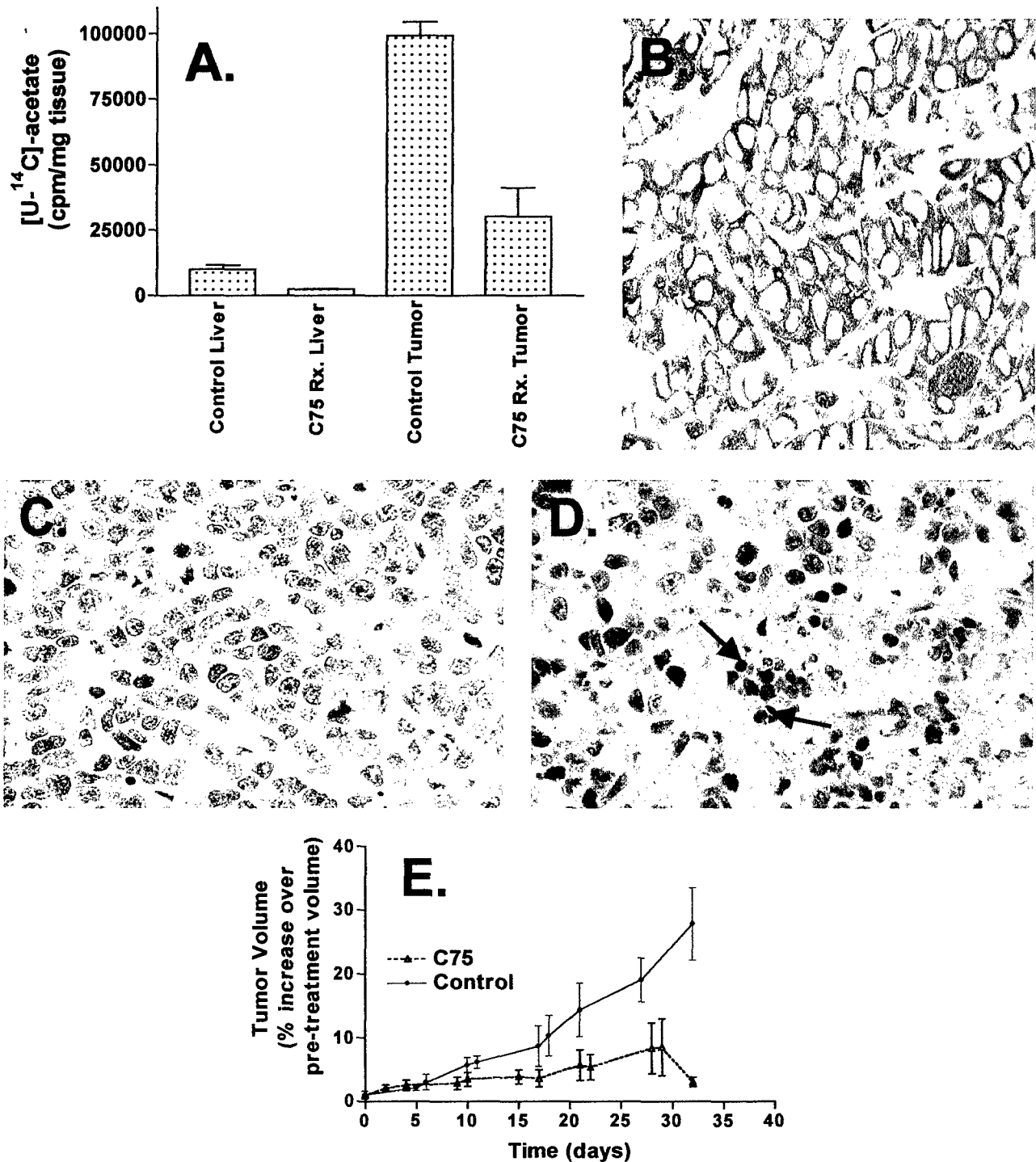
Fig. 4. Selective cytotoxicity of the FAS inhibitor, C75, to MCF7 breast carcinoma flank xenografts in nude mice. A. xenografted tumor had high FA synthesis activity relative to liver, determined by ex vivo metabolic labeling. A standard i.p. dose of C75 (30 mg/kg) inhibited FA synthesis in both liver and tumor by 76 and 70%, respectively, at 3 h (Student's t test, P = 0.04 for liver, P = 0.03 for tumor). B. FAS expression was elevated in the xenografted tumor in parallel with FA synthesis, determined by immunohistochemistry. C and D. a standard i.p. dose of C75 (30 mg/kg) produced histological evidence of widespread apoptosis in the xenografted tumor at 6 h ( D ), which was not evident in vehicle-treated animals ( C ). E. weekly treatment with i.p. C75 (30 mg/kg) inhibited the growth of established MCF7 xenografts, resulting in a greater than 8-fold difference in mean tumor growth between vehicle and drug-treated tumors after 32 days (Student's t test, P = 0.0003 ). Arrows, apoptotic bodies.
