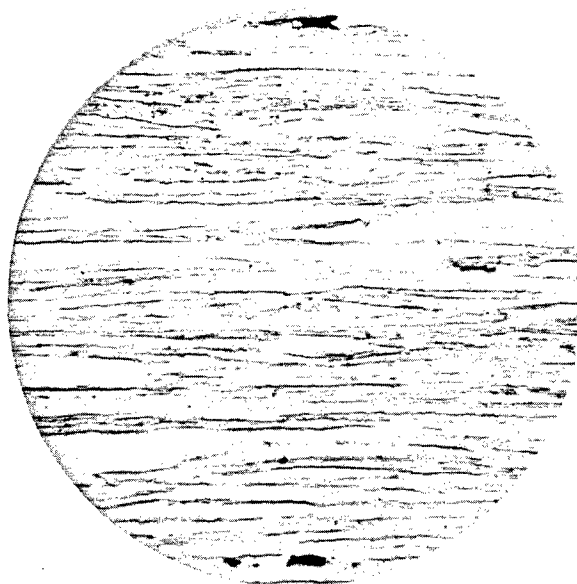
(a) As-extruded
