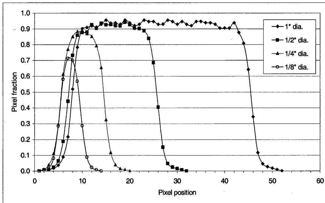
Figure 8. Variation in the intensity of pixels through the axis of a circular hole
