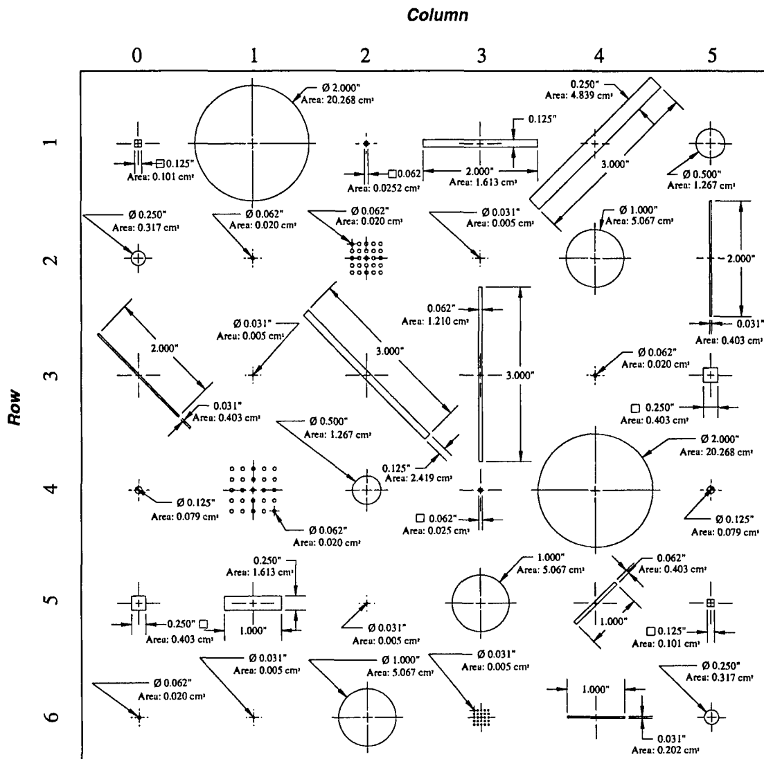
Figure 1. Basic calibration plate pattern
