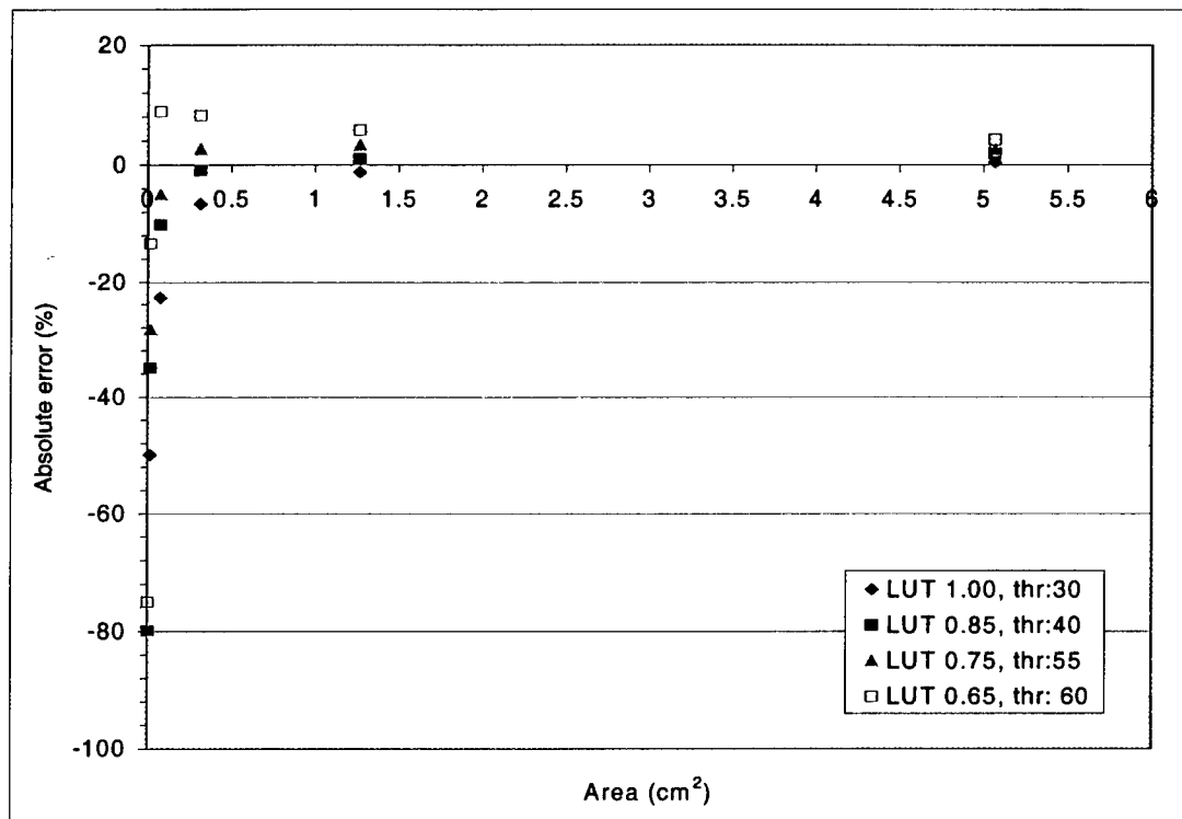
Figure 13. Effect of the LUT value and of the threshold value for circular holes
