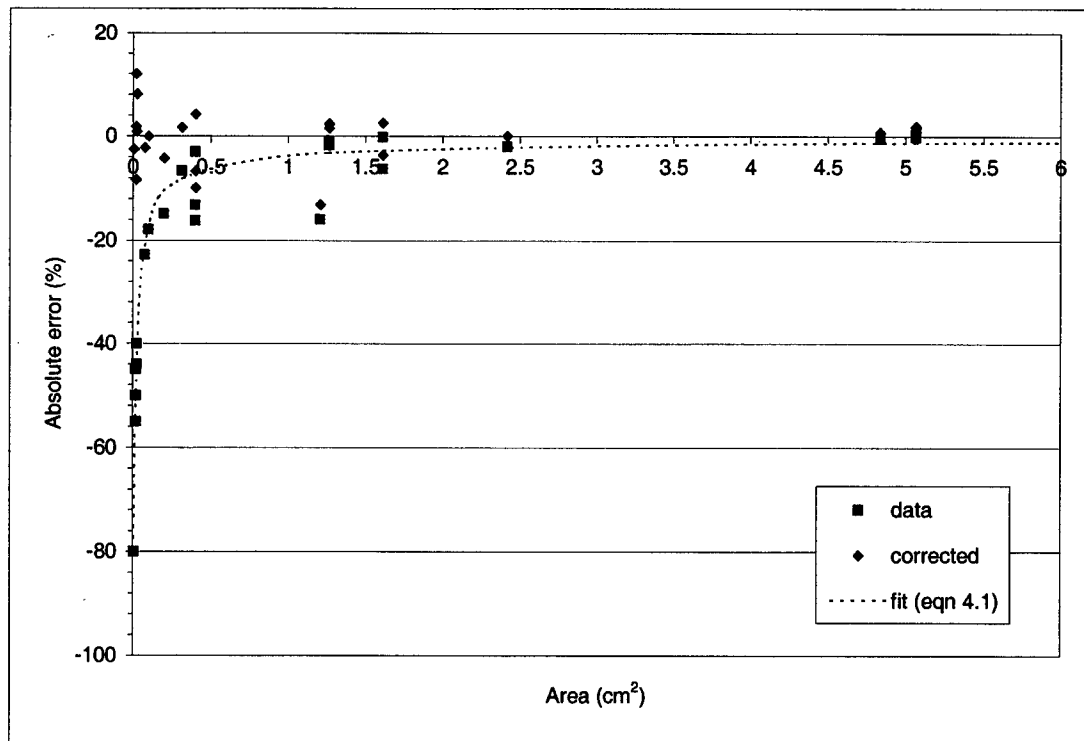
Figure 12. Data of the absolute error (%) for the calibration plate with and without correction (the threshold value=30 and the LUT=1)
