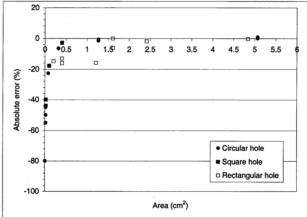
Figure 14. Absolute error (%) for the calibration plate (LUT=1 and threshold=30)
