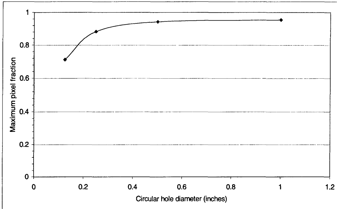
Figure 9. Maximum value of the fraction of pixel found in a hole
