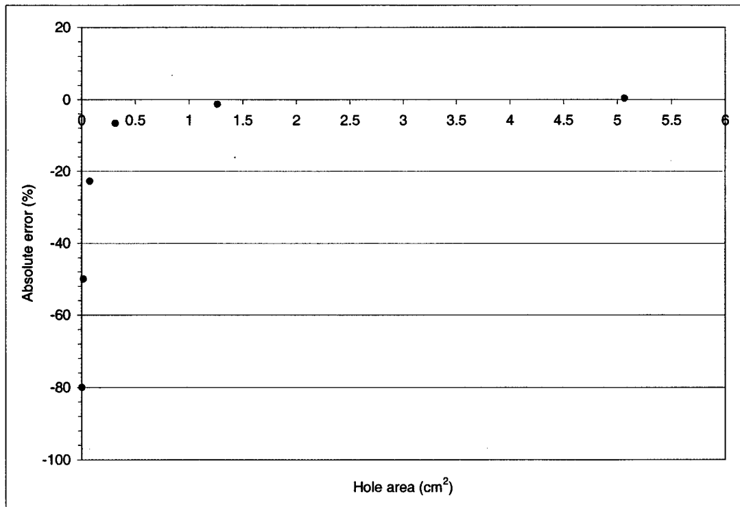
Figure 2. Absolute hole area error (%) for circular holes
