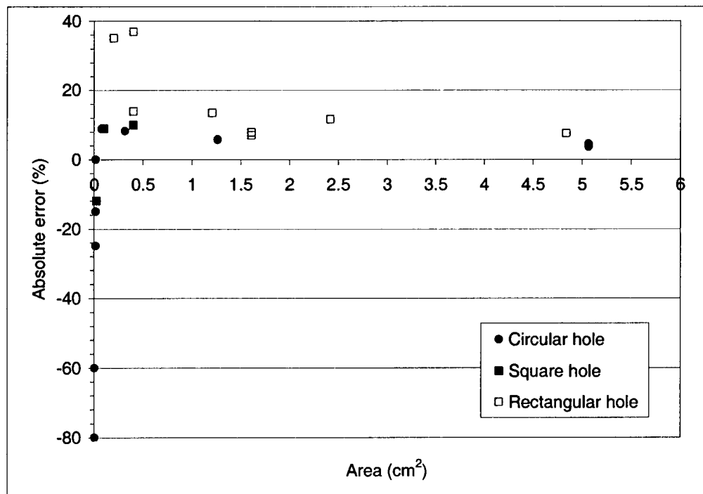
Figure 17. Absolute error (%) for the calibration plate (LUT=0.65 and threshold=60)
