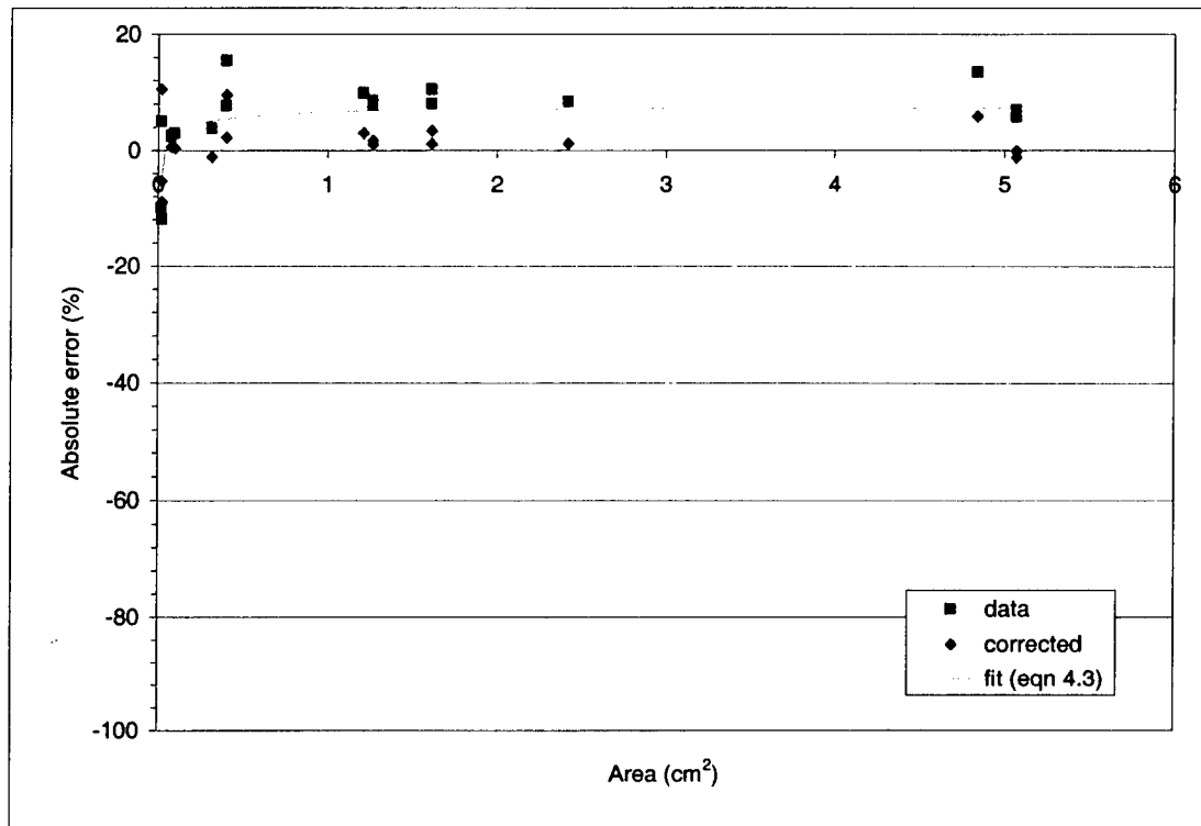
Figure 19. Data of the absolute error (%) for the calibration plate with and without correction (threshold value=40 and the LUT=0.70)
