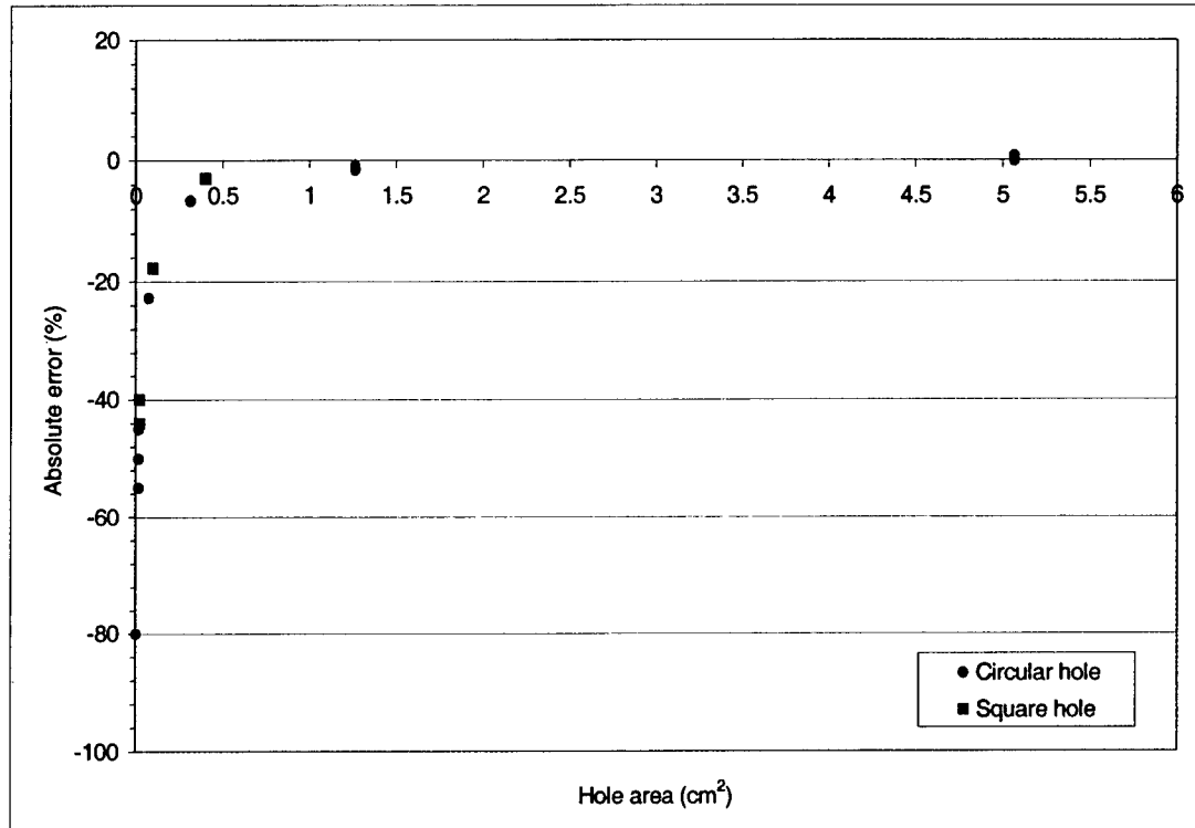
Figure 3. Absolute error (%) for holes having a ratio h/w=1 (i.e. circles and squares)
