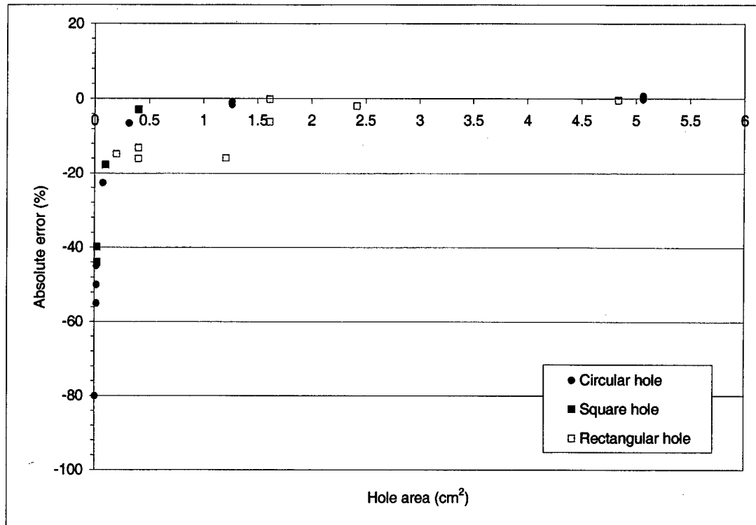
Figure 4. Absolute error (%) for all the holes of the calibration plate using a threshold value equal to 30
