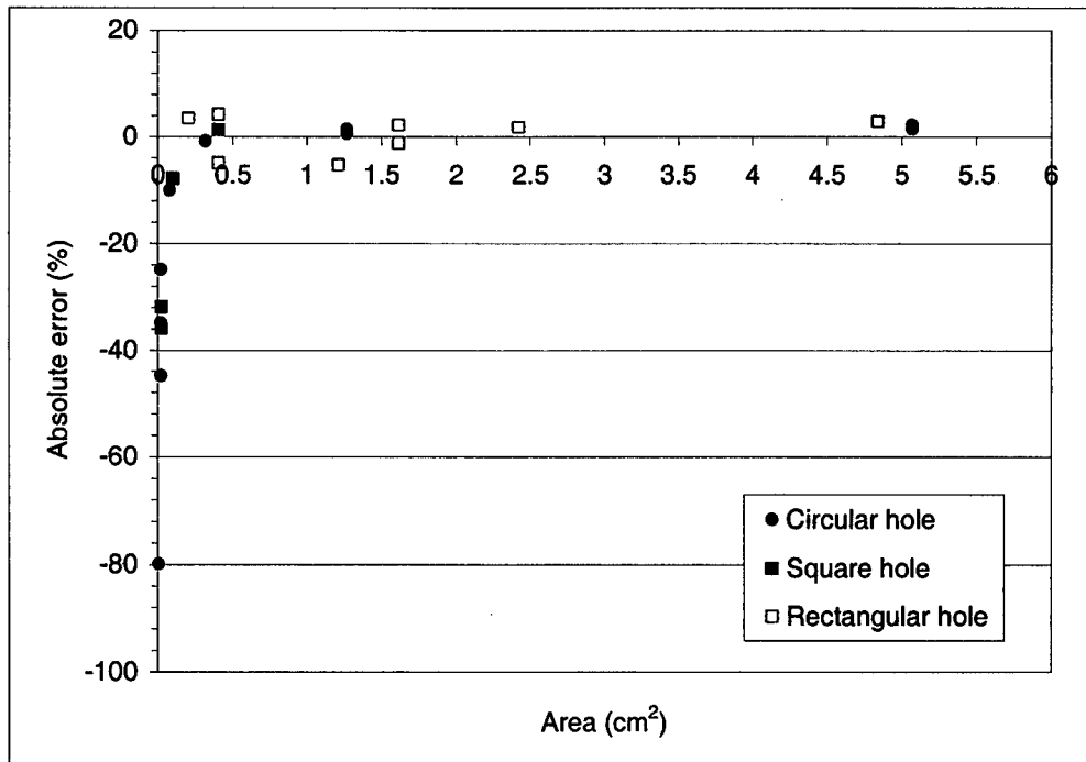
Figure 15. Absolute error (%) for the calibration plate (LUT=0.85 and threshold=40)
