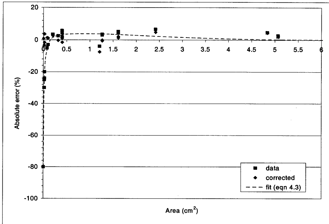
Figure 18. Data of the absolute error (%) for the calibration plate with and without correction (threshold value=55 and the LUT=0.75)
