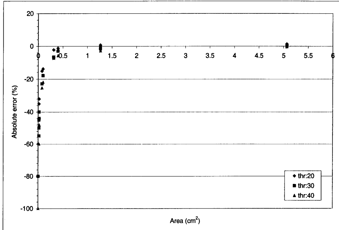
Figure 10. Effect of the threshold value for circular holes from 1/32"Ø to 2"Ø
