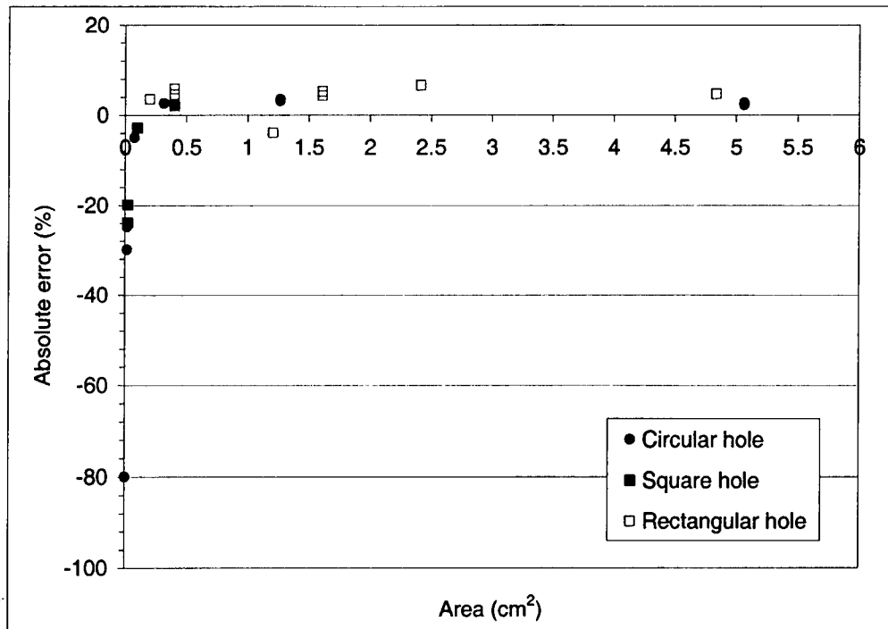
Figure 16. Absolute error (%) for the calibration plate (LUT=0.75 and threshold=55)
