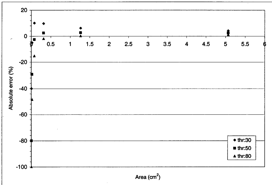
Figure 11. Effect of the threshold value for circular holes from 1/32"Ø to 2"Ø using a LUT value of 0.75
