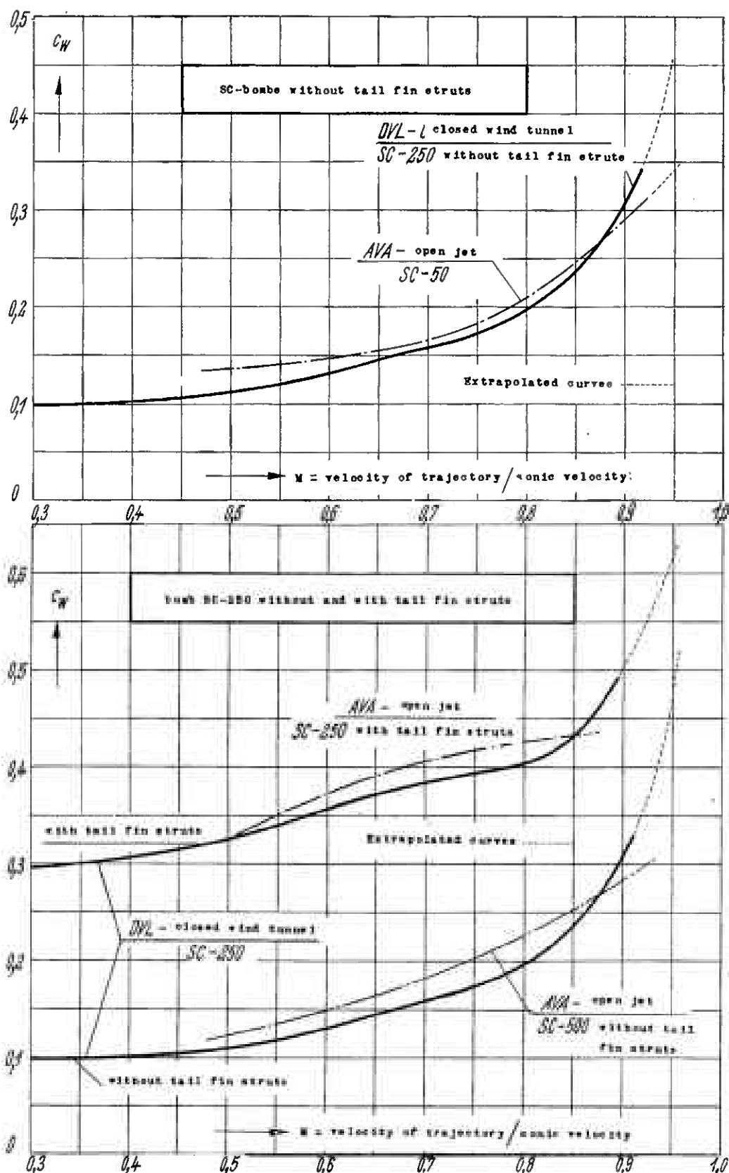
Figure 4.- Comparison of bomb drag coefficients from measurements in the closed DVL wind tunnel and the open jet, AVA-Gottingen.
