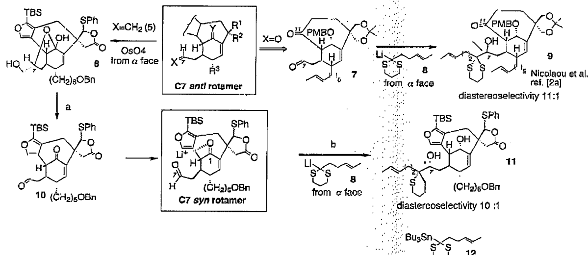
Scheme 2. a) \text{Pb}(\text{OAc})_4 , \text{PhMe} , 0^\circ\text{C} , 20–45 min, 90%; b) 12, \text{MeLi/LiBr} , THF, -78^\circ\text{C} , then add aldehyde at -200^\circ\text{C} , warm to -78^\circ\text{C} , 15 min, 70% total. PMB = p -methoxybenzyl.
