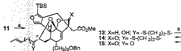
Scheme 3. a) 1. \text{LiOH} , THF, 36 h; 2. \text{CH}_2\text{N}_2 , 60%; b) (\text{COCl})_2 , DMSO, \text{CH}_2\text{Cl}_2 , \text{Et}_3\text{N} , -78^\circ\text{C} , 75%, 14 : 15 = 1:1.
