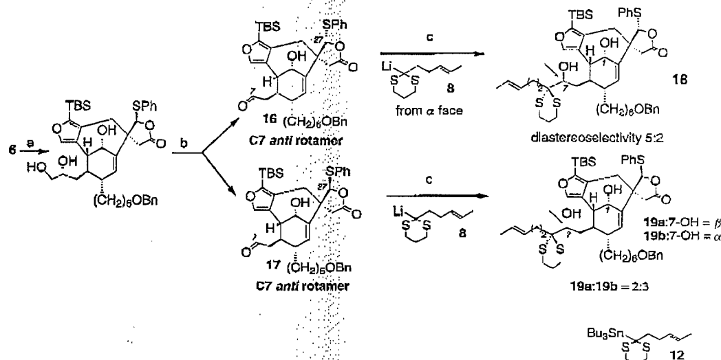
Scheme 4. a) \text{NaBH}_4 , \text{PhMe}/i\text{PrOH} , 6.5 h, 70%; b) \text{Pb}(\text{OAc})_4 , \text{PhMe} , 0^\circ\text{C} , 20–45 min, 90%; c) 12, \text{MeLi/LiBr} , THF, -78^\circ\text{C} , then add aldehyde at -200^\circ\text{C} , warm to -78^\circ\text{C} , 15 min, 70% total.
