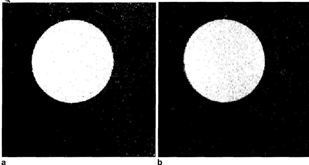
FIG. 9. ADC maps of a T_2 = 60 ms agar phantom obtained (a) using the whole-body coils to provide all diffusion and imaging gradients, TE = 80 ms, and (b) using the breast gradient coils to provide all gradients, where the diffusion gradient strengths were four times the whole-body gradient strengths and TE = 46 ms. In all cases, the ADC maps were constructed from 10 images with b = 0 to b = 1000 s/mm^2 .
