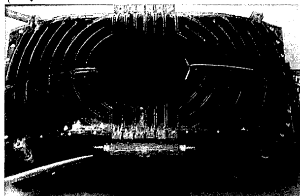
FIG. 5. Assembled gradient coil module showing RF coil and cooling channels.
