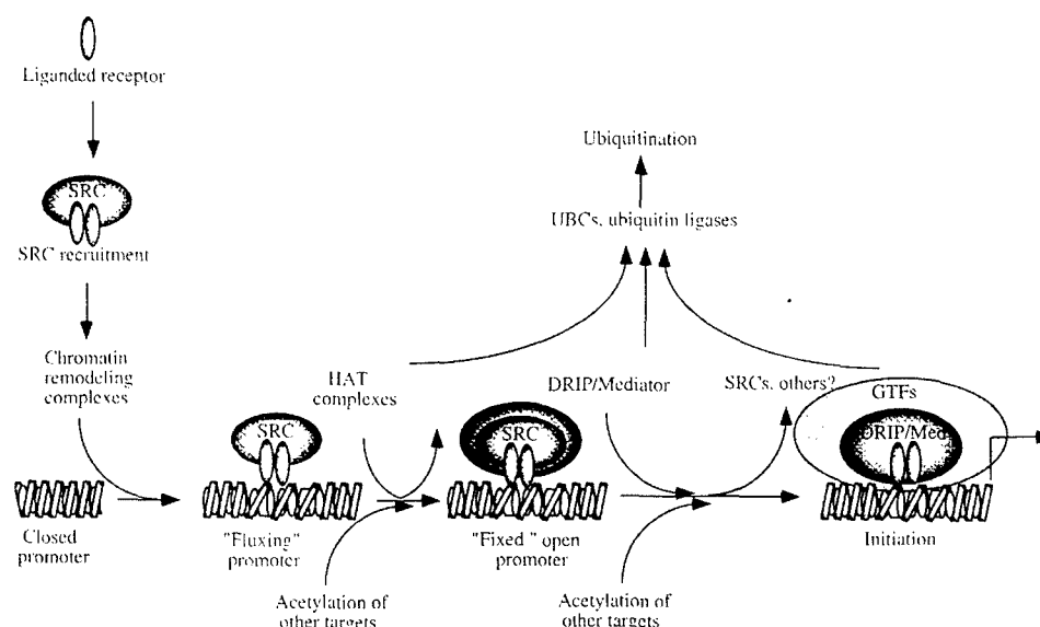
Fig. 2. General dynamic model of assembly and disassembly of distinct coactivator complexes at a hormone-regulated promoter. Acetylase activity and other targeted posttranslational modifications may act as catalysts for promoter fluidity and sequential recruitment of functional domains as required. Ubiquitination appears dominant in cessation of function of the transcriptional complex.
