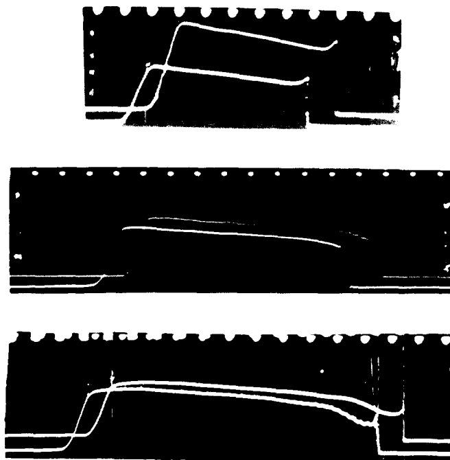
Plate 8. Typical Simultaneous Pressure-time and Thrust-time Traces of 8.5" diameter End-burning Solid Grains of Cast Perchlorate Propellant. (Time axis from right to left)
