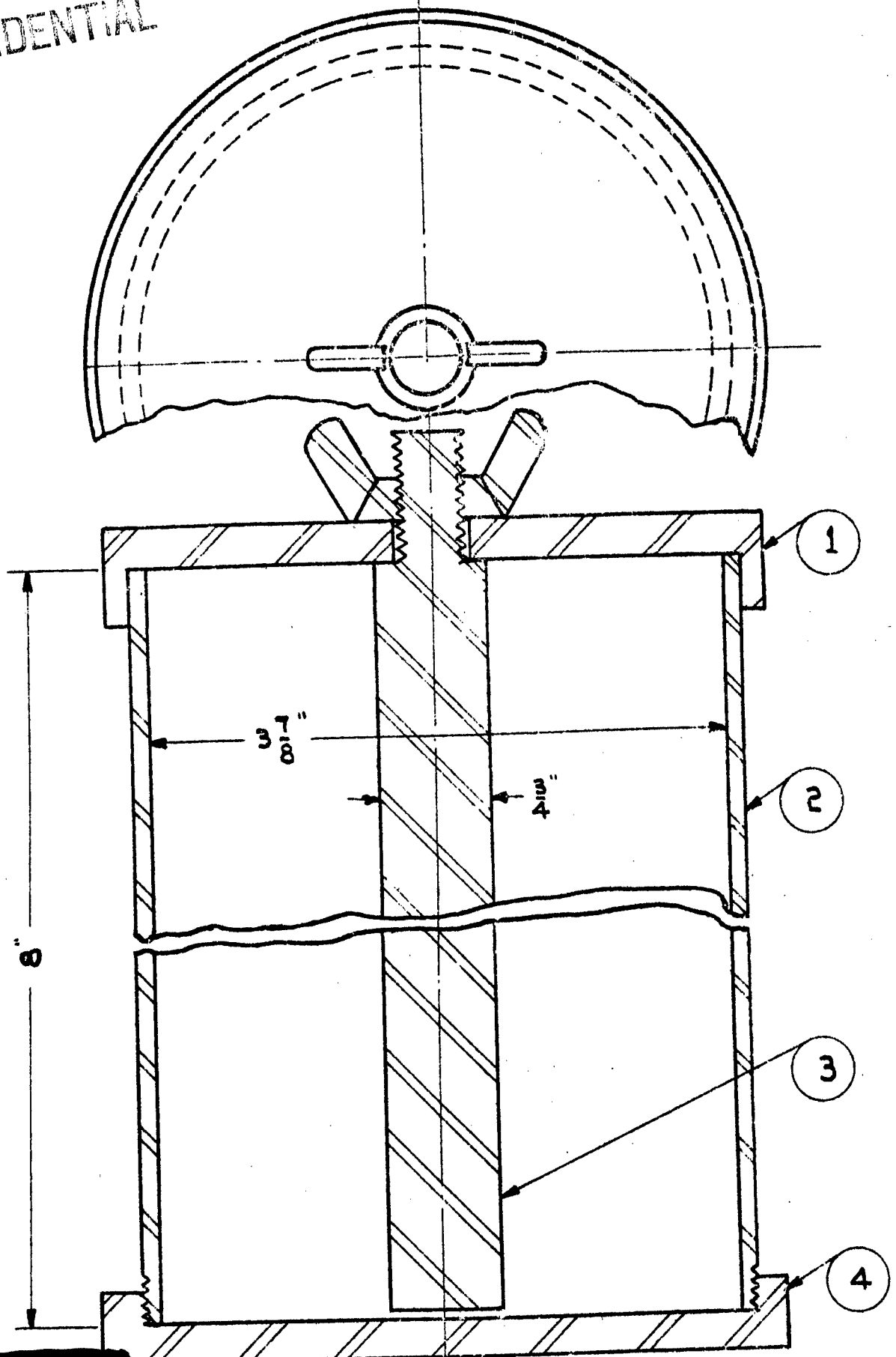
MOLD FOR PERFORATED GRAINS FIGURE 11
