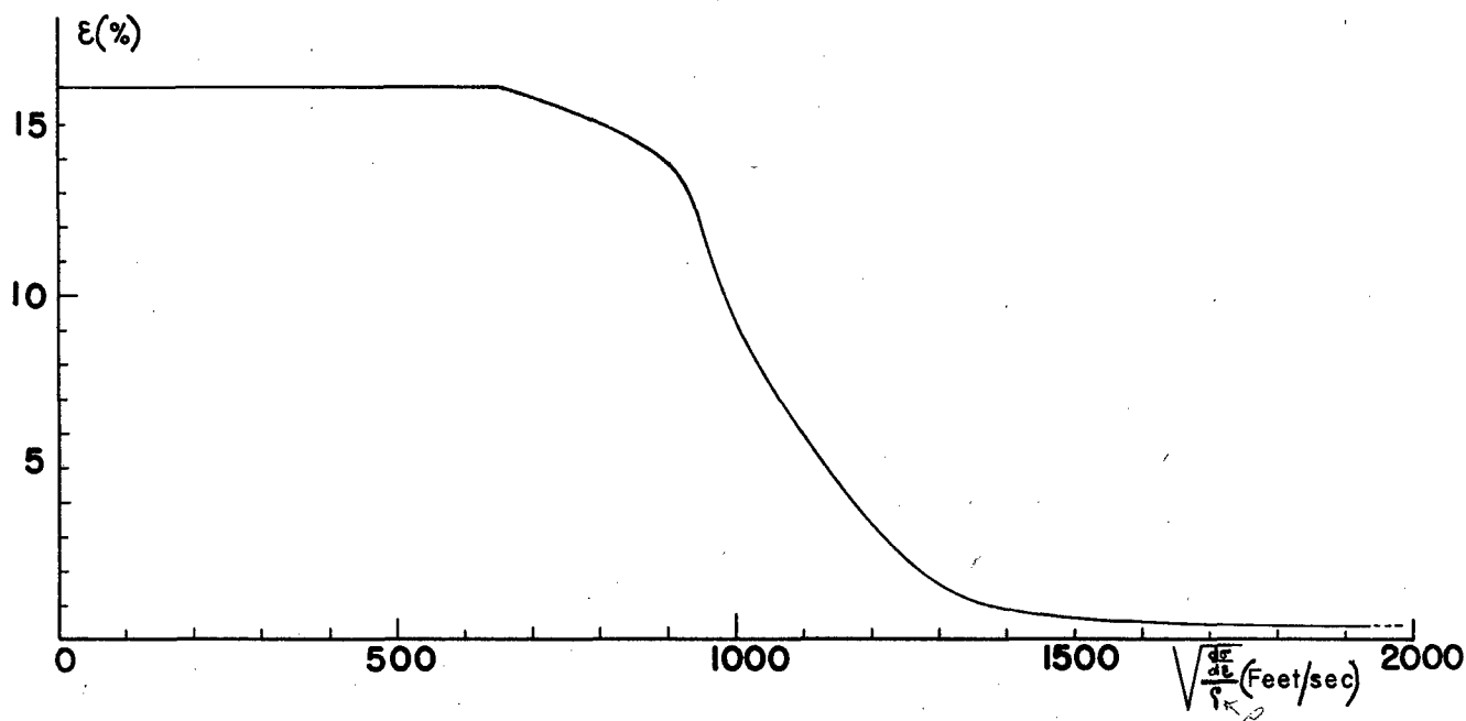
Fig. 3. Permanent set \epsilon versus speed of propagation, as calculated from the static stress-strain curve.
