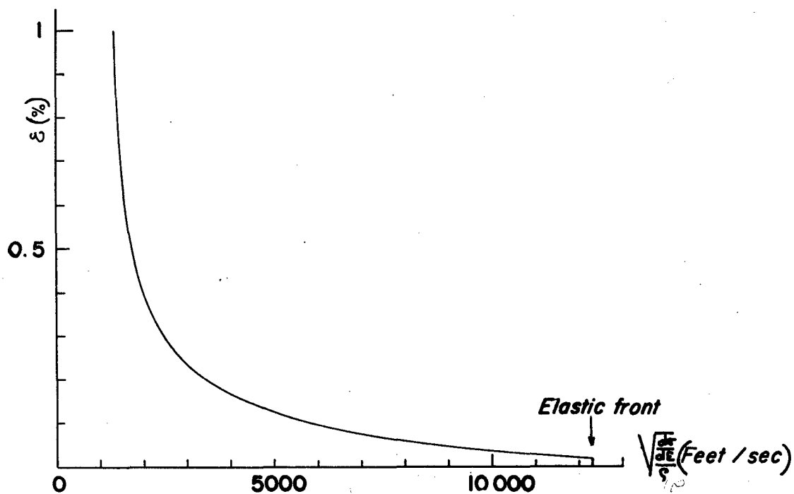
Fig. 4. Continuation of the curve of Fig. 3 up to the elastic front.
