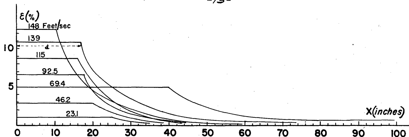
Fig. 10. Distribution of the strain \epsilon along the specimen. The speed of the impact (ft/sec) is indicated on each curve.
