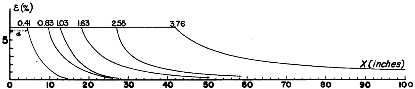
Fig. 8. Distribution of the strain \epsilon along the specimen. Speed of impact, 92.5 ft/sec. The duration of impact (millisec) is indicated on each curve.
