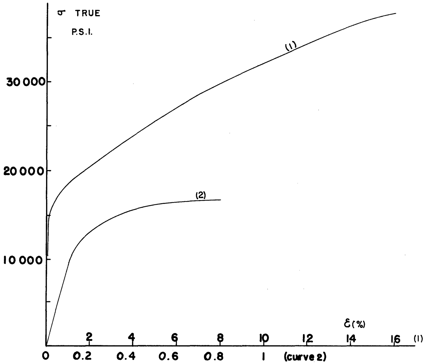
Fig. 2. Static-strain curve for the specimen (copper wire, 0.071 in. diameter). Curve 2 is the portion of the same stress-strain curve with an enlarged scale for the strain.
