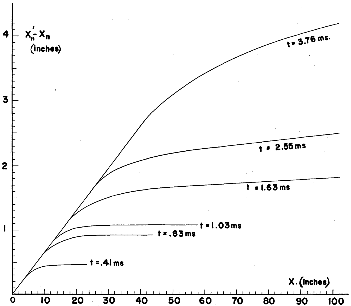
Fig. 6. Distribution of the elongation X'_n - X_n along the specimen. Speed of impact, 92.5 ft/sec. The duration of impact (millisec) is indicated on each curve.
