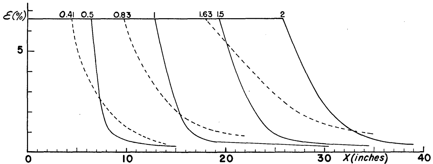
Fig. 12. Plastic waves computed from theory (solid curves) and measured (broken curves). Speed of impact, 92.5 ft/sec. The duration of impact (millisec) is indicated on each curve.
