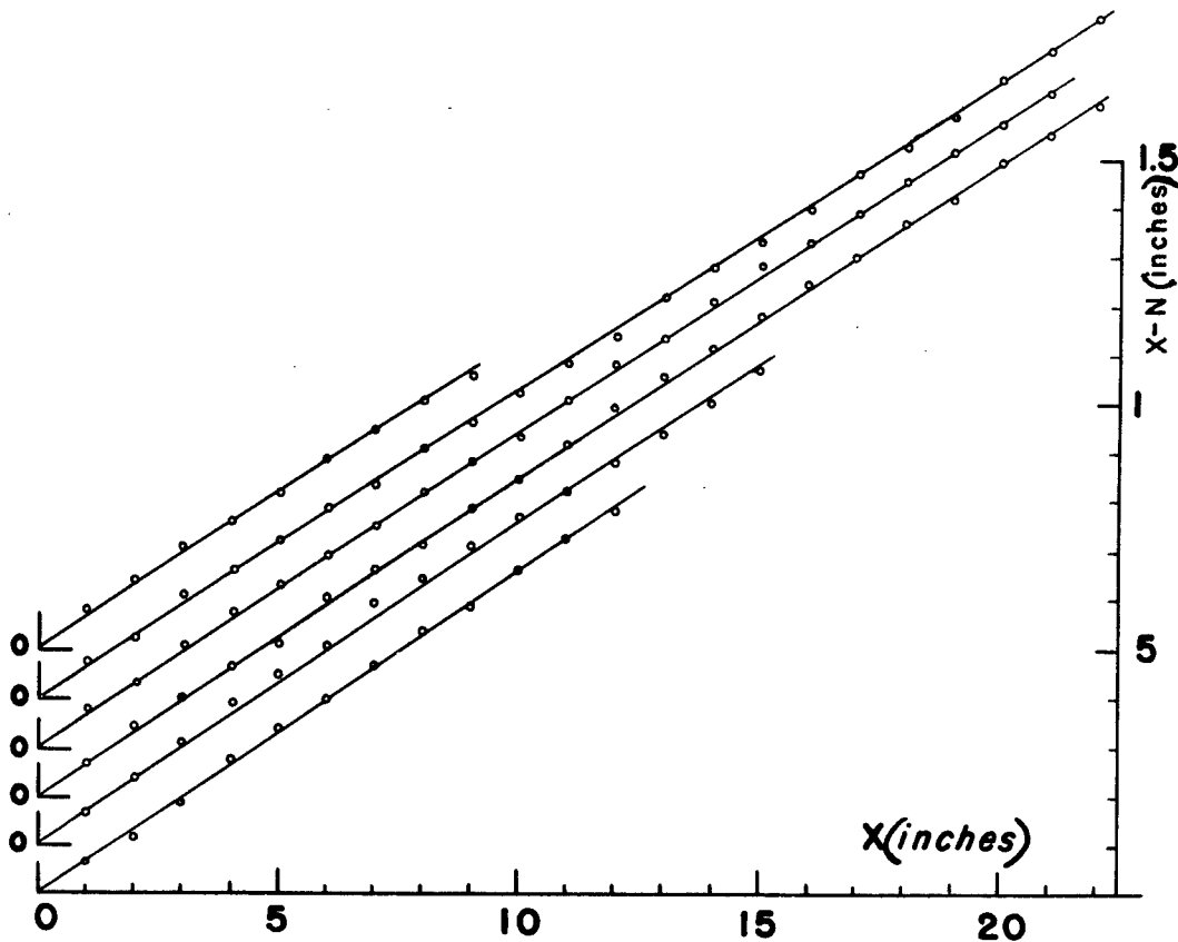
Fig. 7. Linear portions of the curves of Fig. 6, showing the actual readings and their deviations from a straight line.
