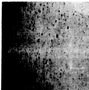
24ST, etched with Kellers reagent.
