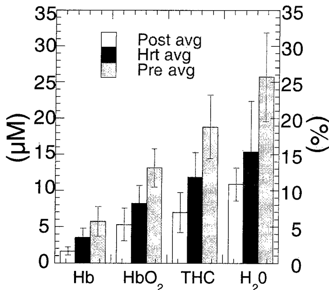
Fig. 6. Mean Hb concentrations [ \mu\text{M} , \text{HbO}_2 , deoxy, and total (THC)] and water ( \text{H}_2\text{O} ) concentration relative to pure water (%) for each subject group. Values are determined from wavelength-dependent absorption values at 674, 803, 849, and 956 or 980 nm. Error bars represent the normalized standard deviation to the mean for six premenopausal, five HRT, and three postmenopausal subjects. Confidence values are \approx 99\% for Hb, \text{HbO}_2 , THC, and \text{H}_2\text{O} .
