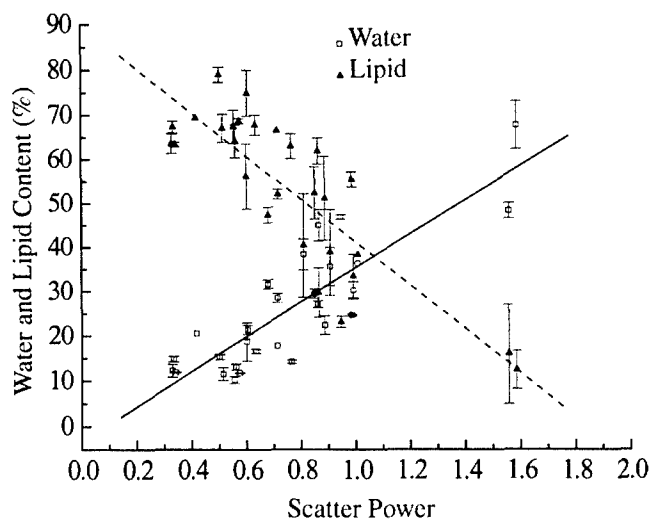
Figure 7. Correlation plots for water percentage (□, solid line) and lipid percentage (▲, dashed line) versus scatter power. Percentages are referenced to the concentration of pure water and the mass density of pure fat. Scatter power correlates with water ( R^2 = +0.850 , P < .001 ) and correlates negatively with lipids ( R^2 = -0.841 , P < .001 ). Error bars show the SDs of repeated measurements.
