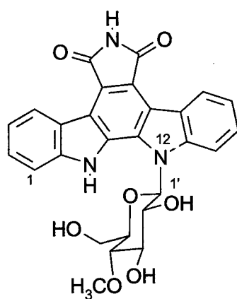
Deschlororebeccamycin
