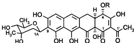
9-C-mycarosylpremithramycinone: R = H
