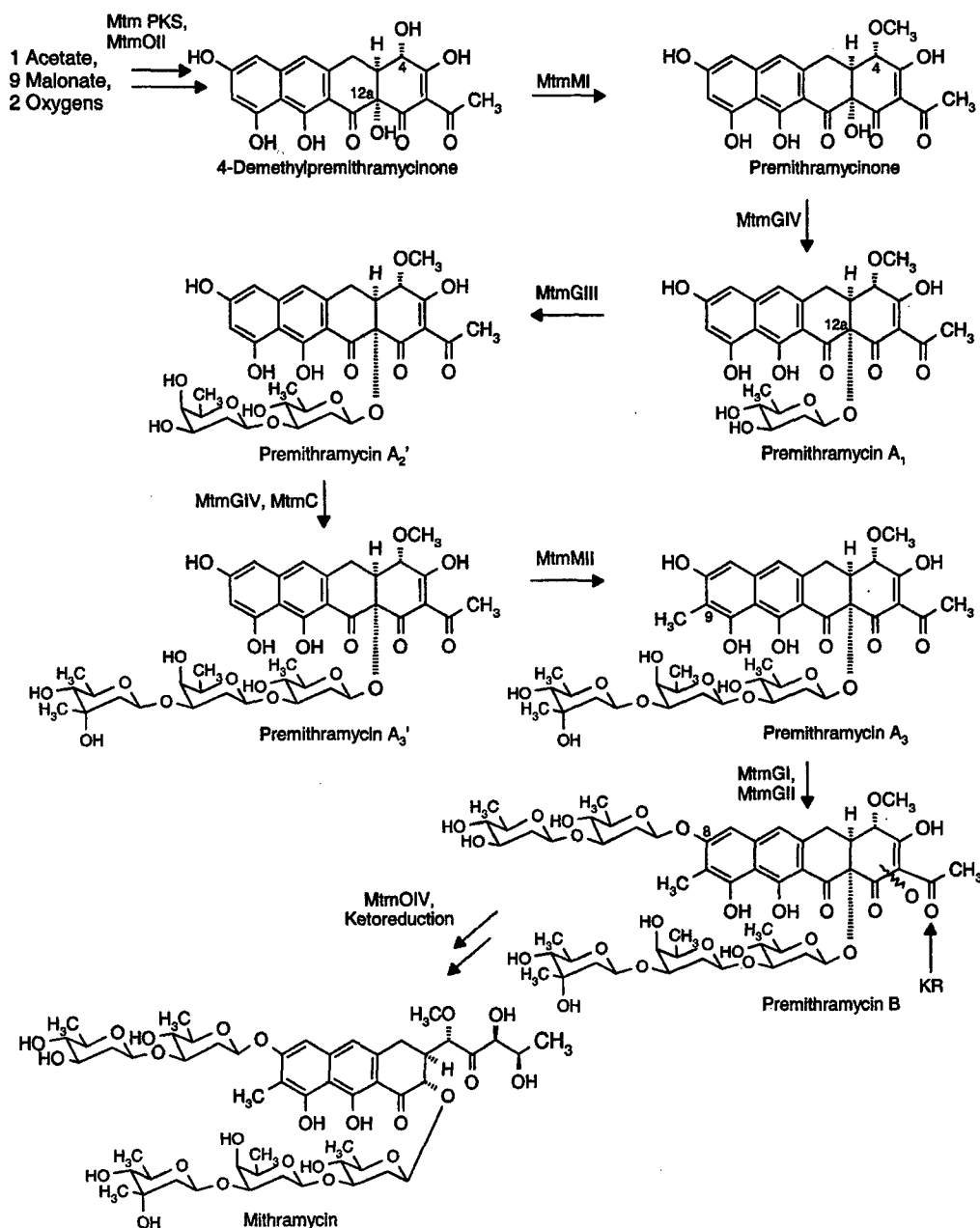
Figure 1. Late biosynthetic pathway to mithramycin showing the sequence of events of the post-PKS tailoring steps catalyzed by oxidoreductases (O = oxygenase; KR = ketoreductase) or group transferases (G = glycosyltransferase; M = methyltransferase). The newly added structural elements of each shown step are highlighted in bold.
