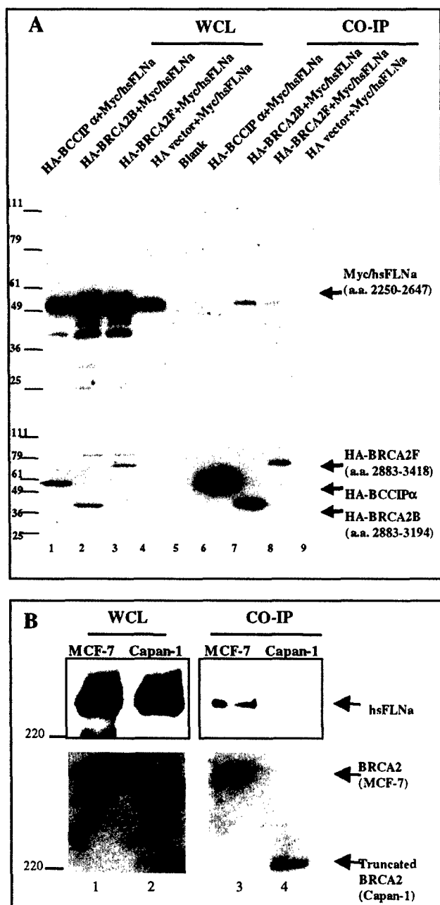
FIG. 4. In vivo interactions of BRCA2 and hsFLNa. A, Myc/hsFLNa (aa 2250–2647) interacts with HA/BRCA2B (aa 2883–3194) or HA/BRCA2F (aa 2883–3418). HA/BCCIPα, HA/BRCA2B (aa 2883–3194), HA/BRCA2F (aa 2883–3418), or empty HA vector was co-expressed with Myc/hsFLNa (aa 2250–2647) in 293 human kidney cells. The HA-tagged proteins were immunoprecipitated with anti-HA affinity matrix. Co-immunoprecipitated Myc/hsFLNa (aa 2250–2647) was detected by anti-Myc antibody (top panel), and HA-tagged proteins were detected with anti-HA antibody (bottom panel). Lanes 1–4 show the protein from whole cell lysate (WCL), and lanes 6–9 are the precipitated proteins. Lane 5 is a blank. Myc/hsFLNa co-precipitates with HA-BRCA2B (aa 2883–3194) (lane 7) and HA-BRCA2F (aa 2883–3418) (lane 8), but not HA-BCCIPα (lane 6) or the HA vector control (lane 9). B, endogenous BRCA2 interacts with hsFLNa. Whole cell lysate (WCL) from MCF-7 and Capan-1 cells were incubated with anti-BRCA2 (Ab1, Oncogene) that reacts with amino acids 1651–1821 of BRCA2 in both MCF-7 and Capan-1 cells. The precipitated BRCA2 complex was immunoblotted with anti-hsFLNa antibody (top panel) and anti-BRCA2 antibody (bottom panel). In the bottom panel, full-length BRCA2 from MCF-7 (lane 1) or truncated BRCA2 from Capan-1 (lane 2) is detected in whole cell lysate as well as the immunoprecipitated complex (lanes 3 and 4). However, hsFLNa is only co-precipitated with the full-length BRCA2 in MCF-7 cells (lane 3, top panel) but not with the truncated BRCA2 in Capan-1 cells (lane 4, top panel). This figure shows that the endogenous full-length BRCA2 in MCF-7 co-precipitates the endoge-
