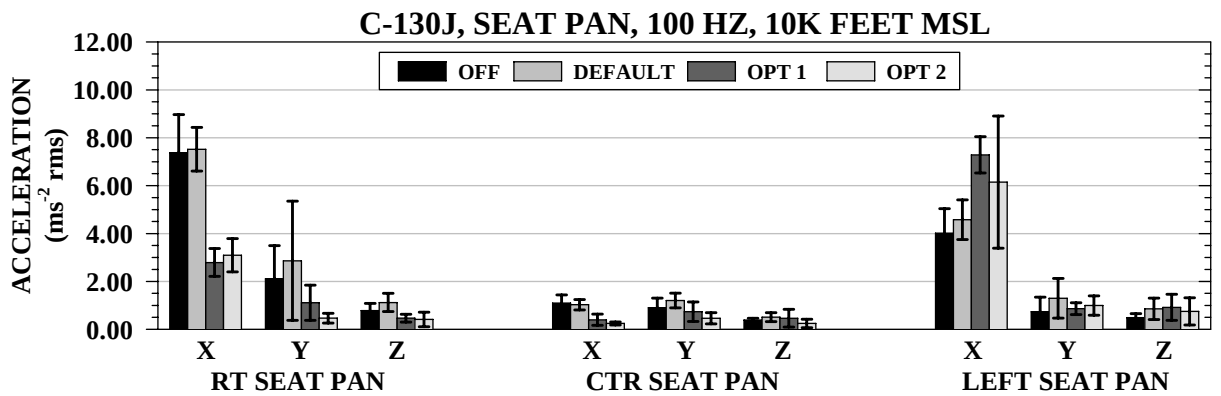
Figure A-8. Mean C-130J 100-Hz One-Third Octave Propeller Plane Seat Pan Accelerations +/- One Standard Deviation at 10K Feet MSL
