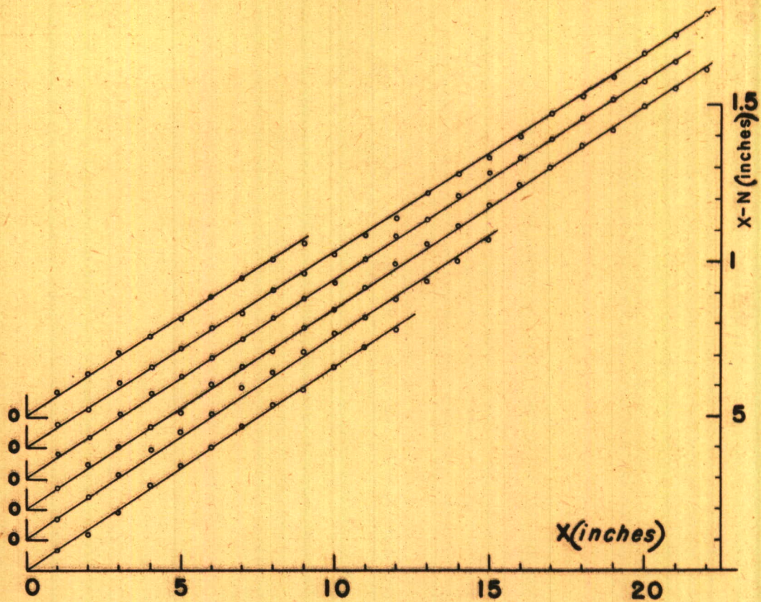
Fig. 7. Linear portions of the curves of Fig. 6, showing the actual readings and their deviations from a straight line.
