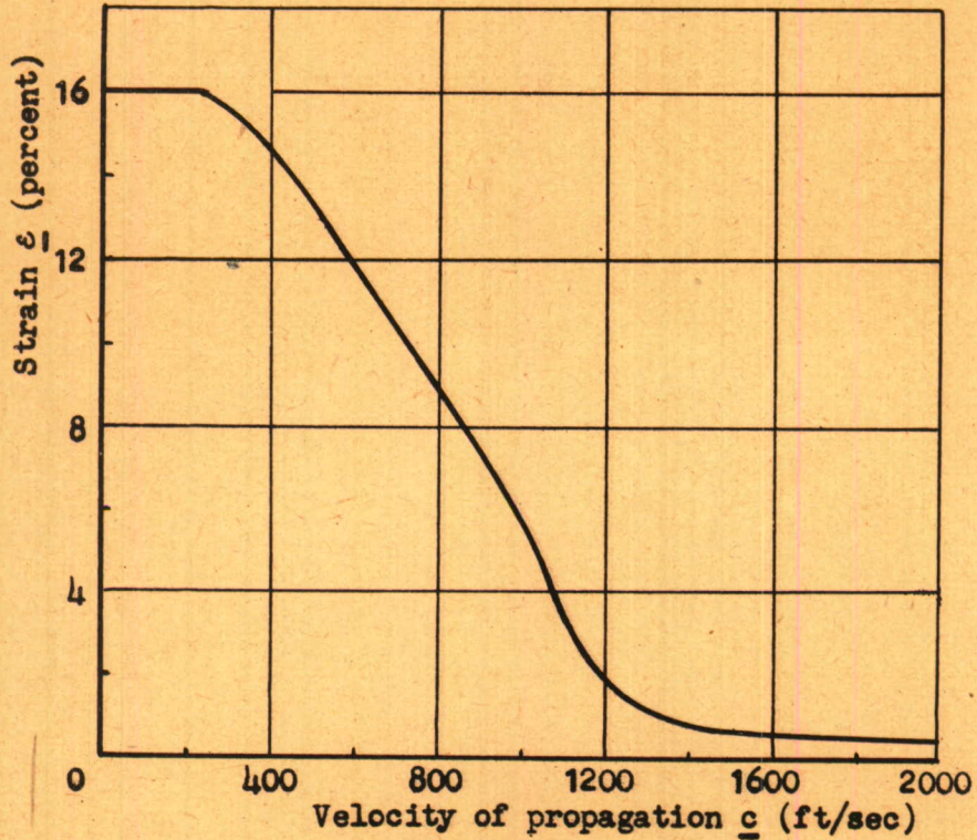
Fig. 3. Strain \epsilon_1 versus velocity of propagation c , as calculated from the static stress-strain curve.
