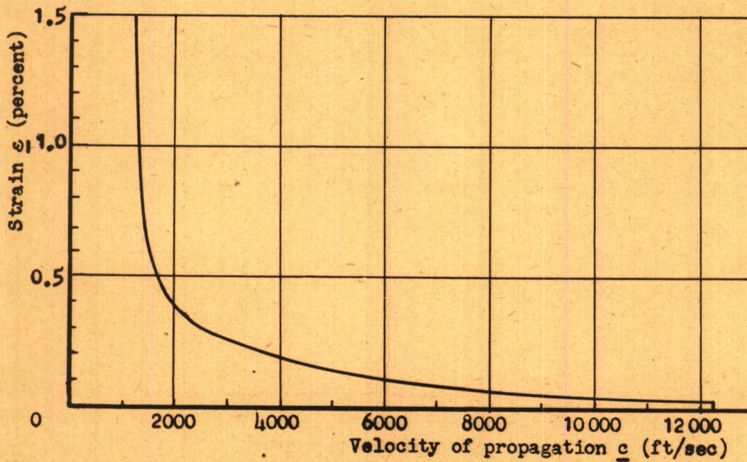
Fig. 4. Continuation of the curve of Fig. 3 up to the elastic point.
