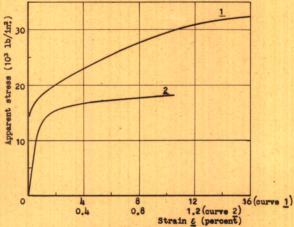
Fig. 2. Static apparent stress-strain curve for copper wire 0.071 in. in diameter. Curve 2 is the portion of the same stress-strain curve with an enlarged scale for the strain.
