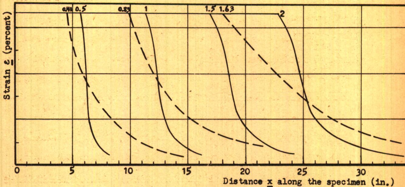
Fig. 12. Plastic waves computed from theory (solid curves) and measured (broken curves). Impact velocity, 92.5 ft/sec. The duration of impact (millisec) is indicated on each curve.
