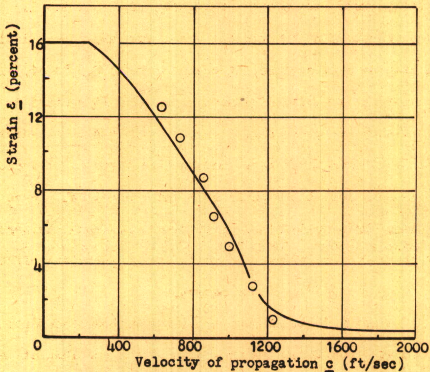
Fig. 13. Same curve as Fig. 3 with experimental results (dots) added.
