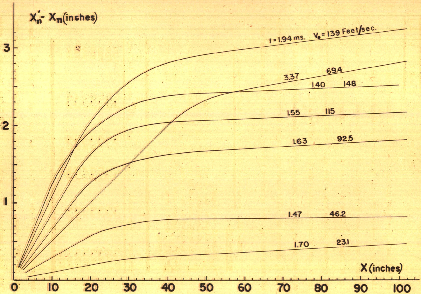
Fig. 9. Distribution of the elongation X'_n - X_n along the specimen. The velocity and duration of impact are indicated on each curve.
