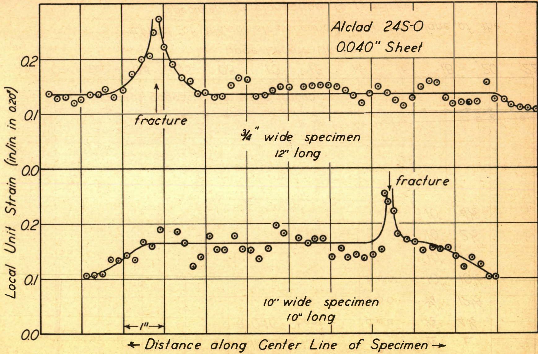
Effect of specimen width on local elongation near fracture
