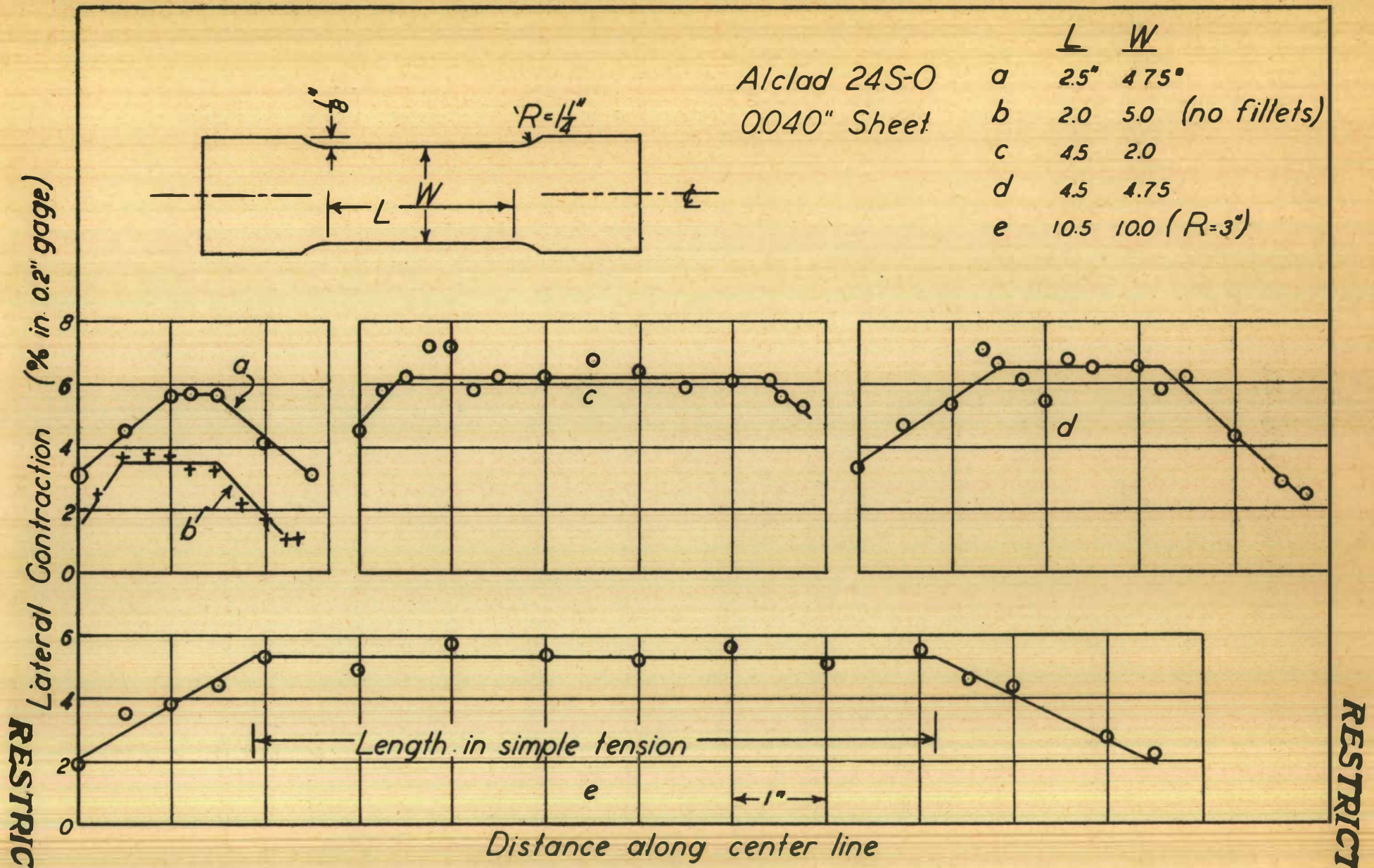
Fig. 1 Method of determining length in simple tension from lateral contraction measurements
