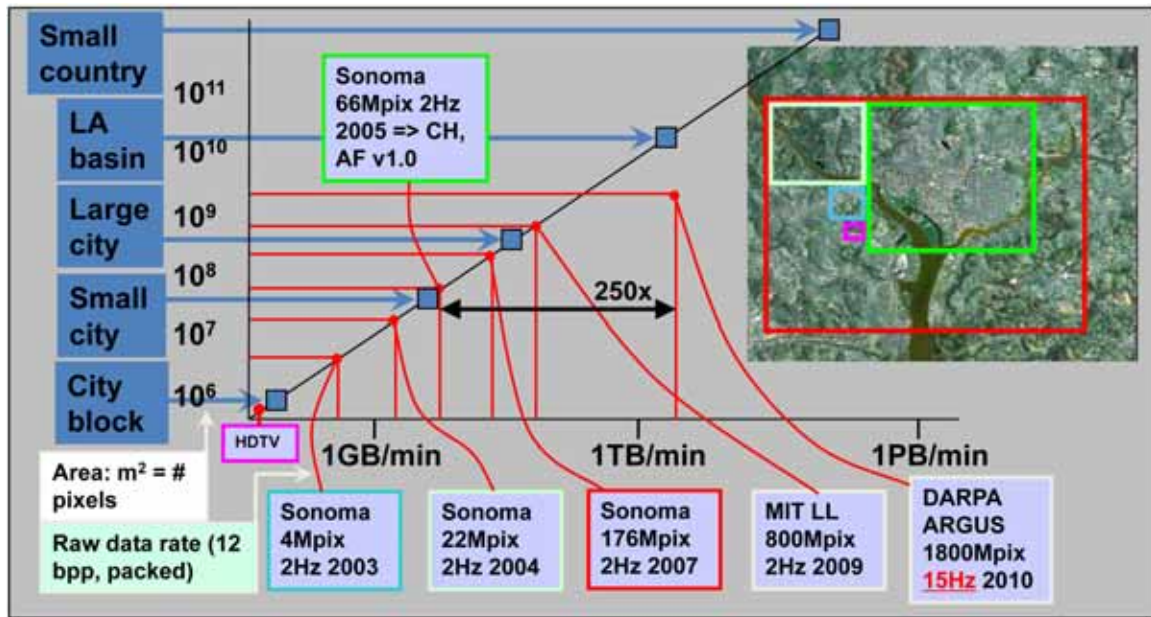
Figure 6-1: A plot of sensor capability vs. data rate for past, present day and future sensor systems [7]
