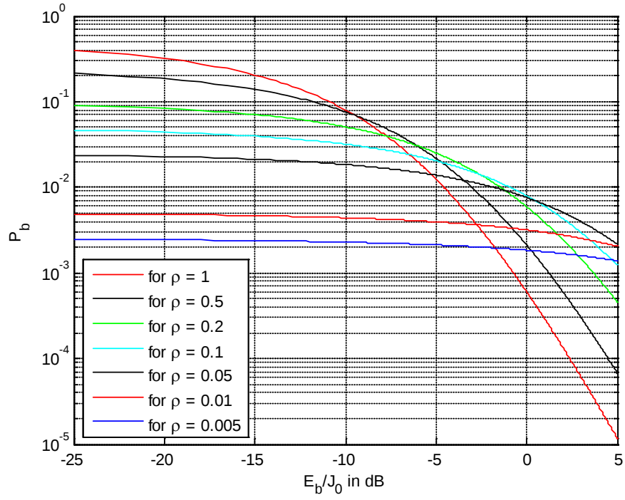
Figure 37. BER of DS QPSK system for pulsed jamming and diversity L=4 .
