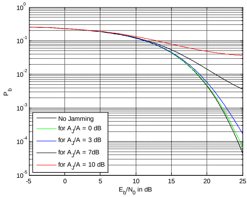
Figure 135. BER of DS 64QAM MIMO for tone jamming and diversity L=9 .
