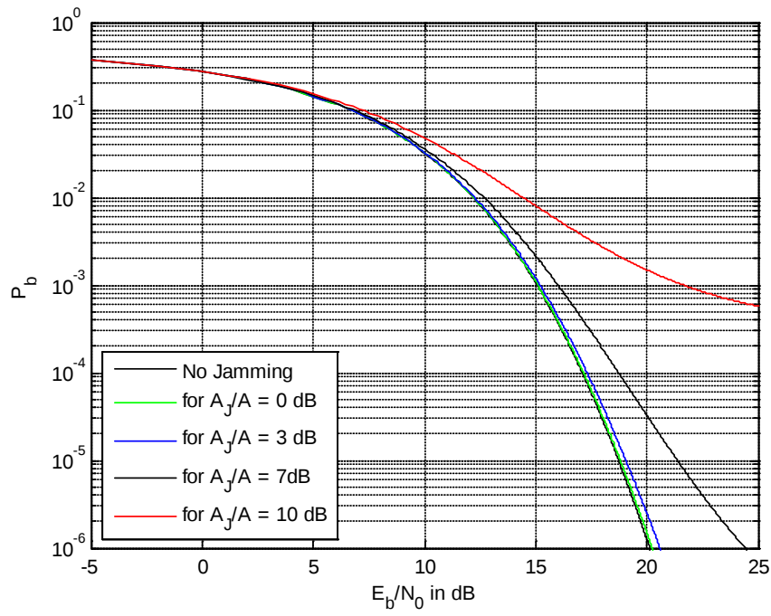
Figure 120. BER of DS QPSK MIMO for tone jamming and diversity L=12 .
