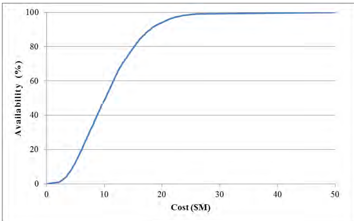
Figure 17: The Cost vs. Availability Curve of One Aircraft
