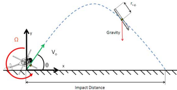
Figure 23: Ballistic Trajectory of Rotor Blade with no Wind Resistance
