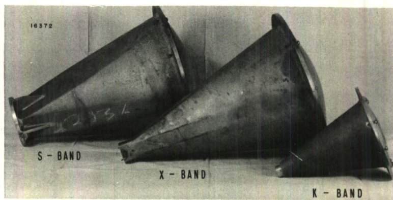
Figure 3 - Cast aluminum horns assembled with lenses
