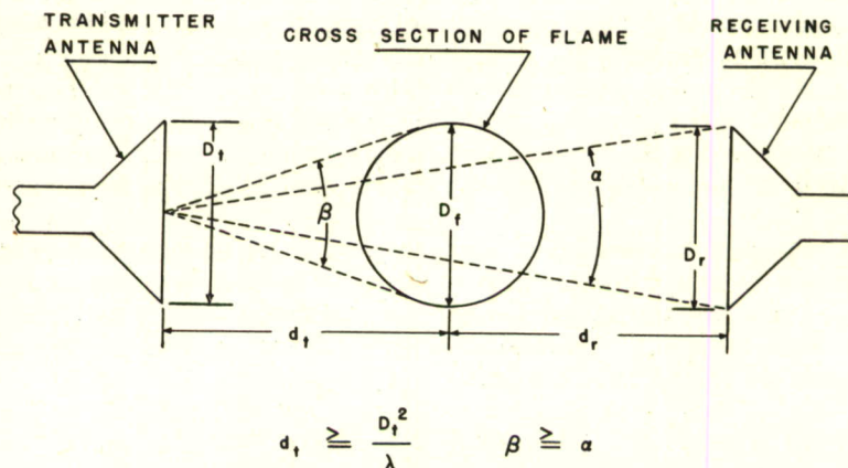
Figure 1 - Antenna arrangement
