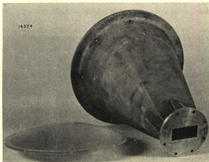
Figure 2 - Cast aluminum horn and converging lens
