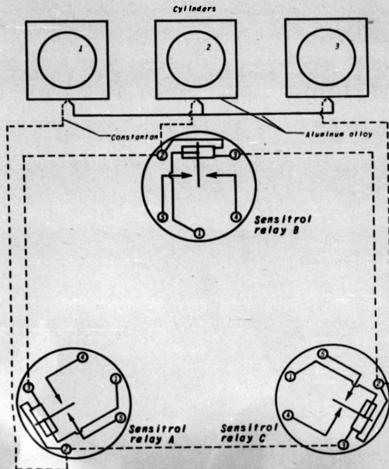
Figure 2. - Simplified circuit diagram of preignition indicator.
