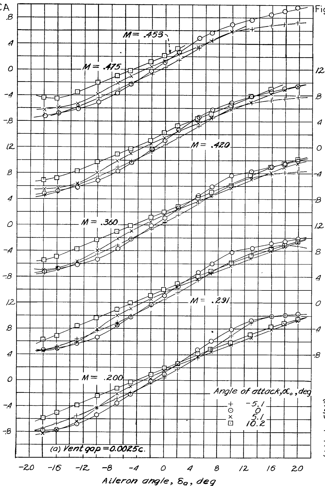
Figure 8. - Variation of pressure coefficient across the balance with aileron angle
