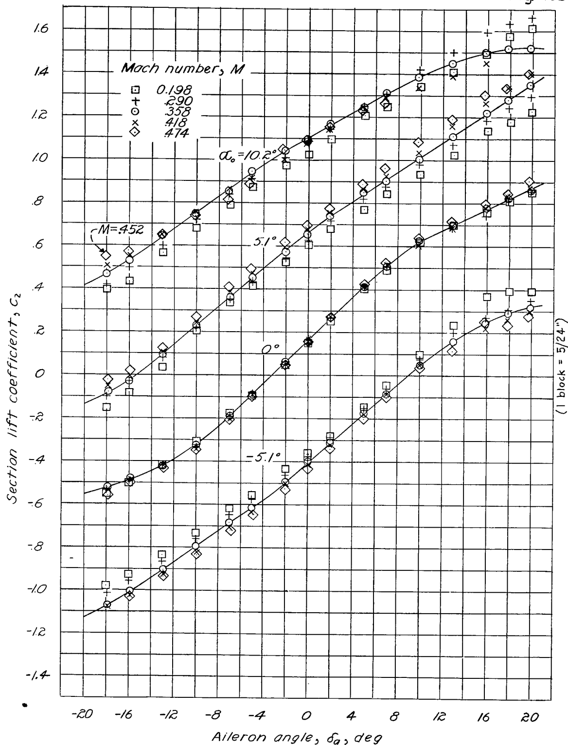
Figure 13. — Variation of section lift coefficient with aileron angle. (Continued.)
