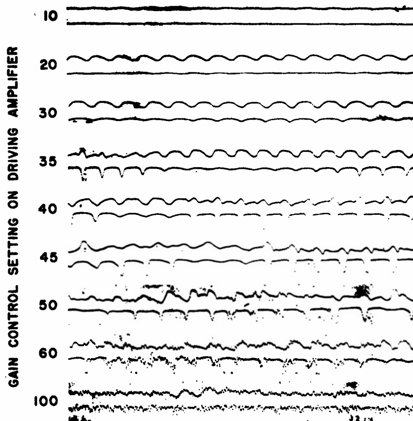
Figure 35.- Oscillograms of u -fluctuations showing development of turbulence from oscillations produced by vibrating ribbon at position 2.5 feet downstream from ribbon. Ribbon 3 feet from leading edge of plate. Simultaneous records at 0.014 inch from surface, upper trace; and 0.114 inch from surface, lower trace. Frequency 70 cps. U_0 = 50 ft per sec.
