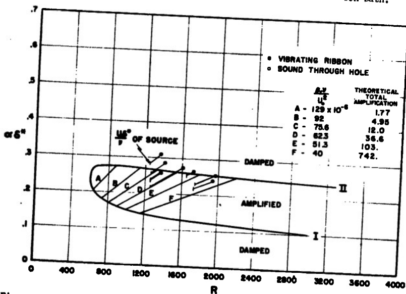
Figure 20.- Wave-length diagram showing zone of amplification according to Schlichting. Points show values of \alpha\delta^2 for frequencies of Figure 19. Lines from points show path of amplification.
