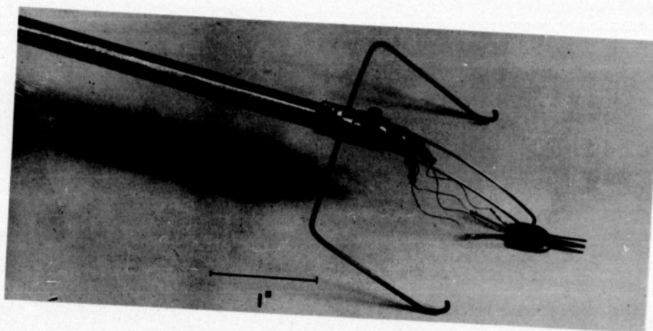
Figure 6.- Sled-like hot-wire head arranged for two hot wires.
