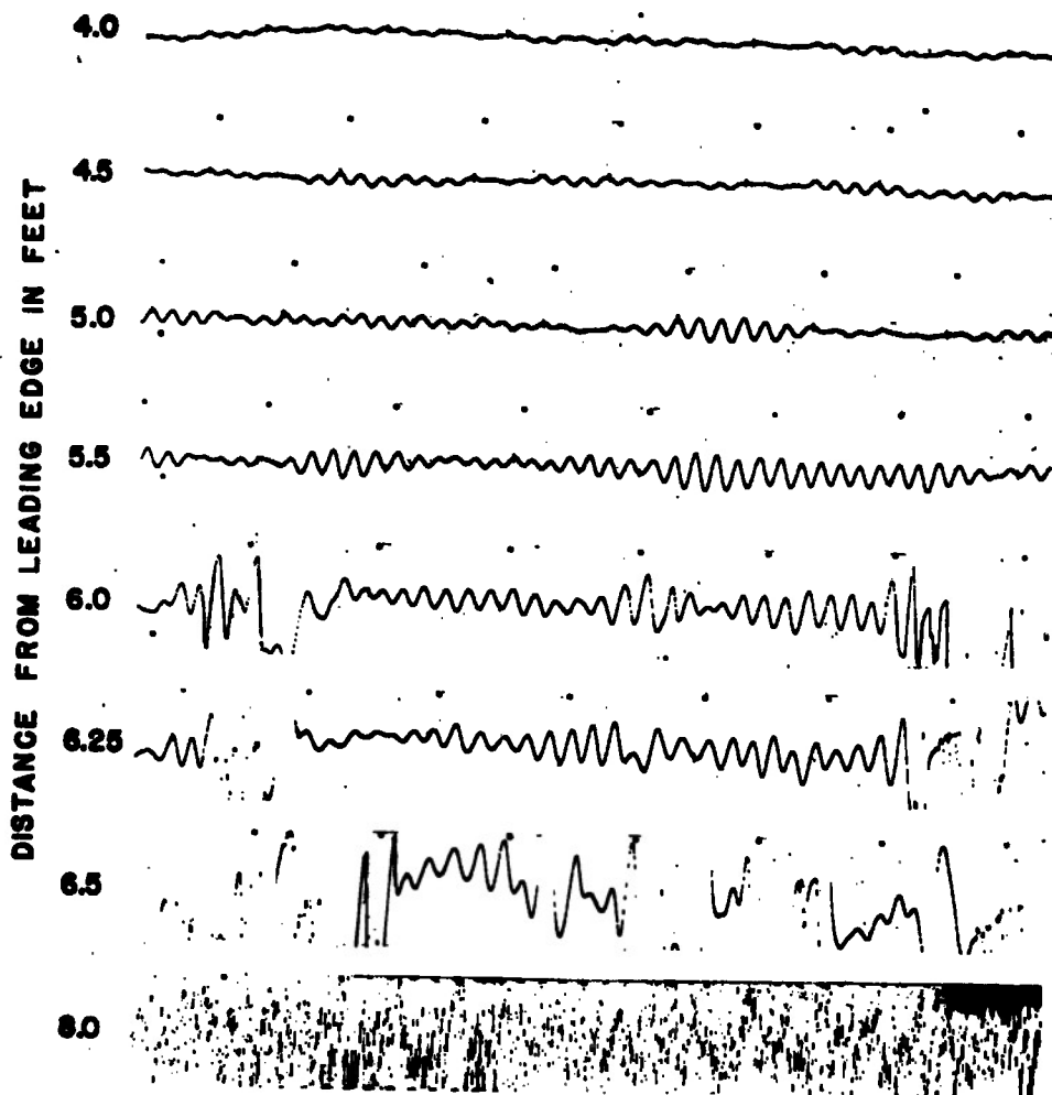
Figure 9.- Oscillograms of u-fluctuations showing laminar boundary-layer oscillations in boundary layer of flat plate. Distance from surface = 0.023 inch. U_0 = 80 ft per sec. Time interval between dots = 1/30 sec.
