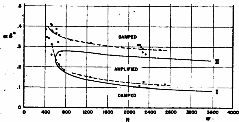
Figure 25.- Wave-length of neutral oscillations excited in boundary layer by vibrating ribbon. Solid curve is neutral curve according to Schlichting. Broken curves are neutral curves defined by experimental points. Closed circles-branch I. Open circles-branch II.
