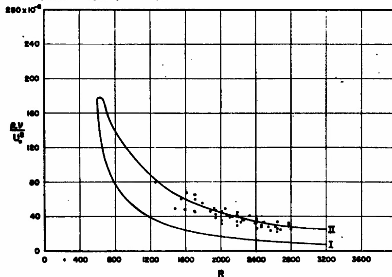
Figure 16.- Boundary layer oscillations excited by loudspeaker. Points show sound frequency giving maximum amplification. Curve outlines theoretical amplification zone. (See Figure 13).
