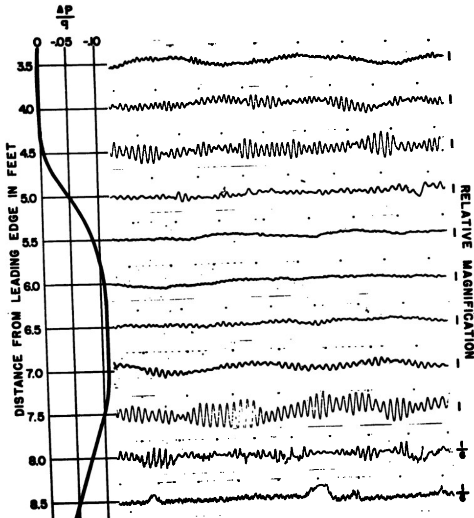
Figure 29.- Oscillograms of u -fluctuations showing effect of pressure gradient on boundary-layer oscillations. Distance from surface = 0.081 inch. U_0 = 95 ft per sec. Time interval between dots = 1/30 sec.
