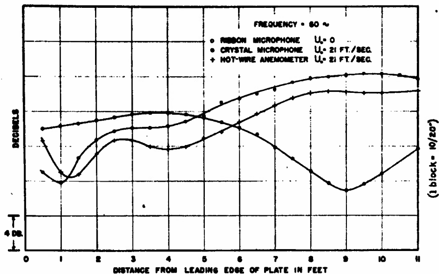
Figure 15.- Relative sound intensity from loudspeaker in ceiling of working chamber at leading edge of plate, measured along center 2 inches from plate. Frequency = 60 cps.
