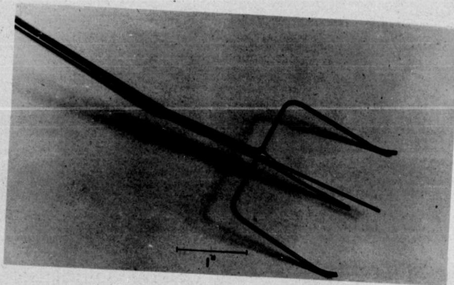
Figure 2.- Pitot-static surface tubes used to measure pressure distribution and position of transition.
