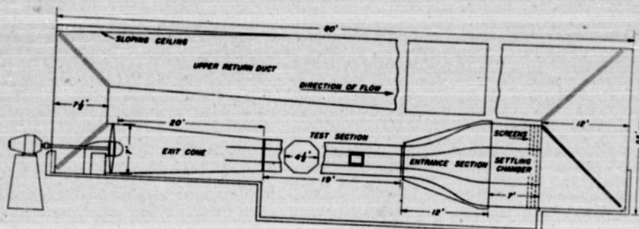
Figure 1.- Elevation view of 4 1/2-foot wind tunnel.
