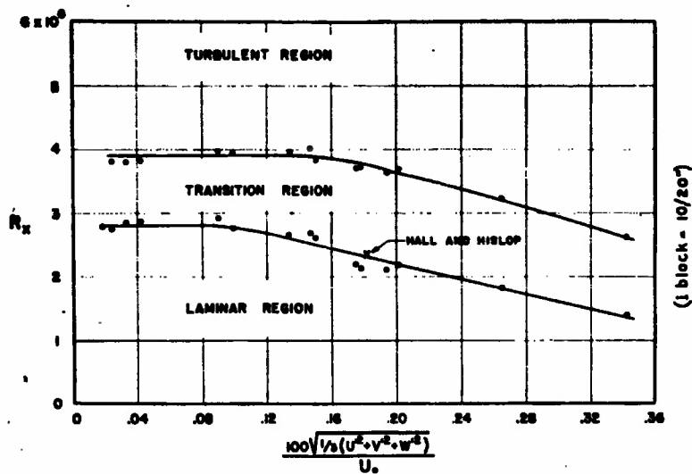
Figure 7.- Effect of turbulence on x-Reynolds number of transition. Flat plate, zero pressure gradient.
