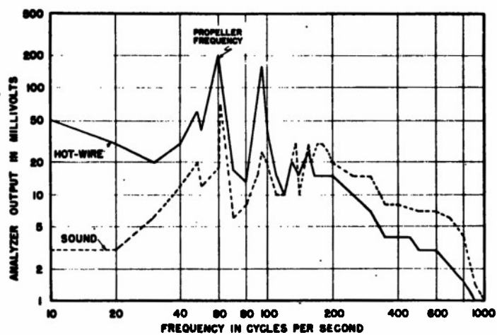
Figure 8.- Distribution with frequency of u-component of turbulence and sound. Wind speed = 80 ft per sec, u'/U_0 (total) = 0.033%.
