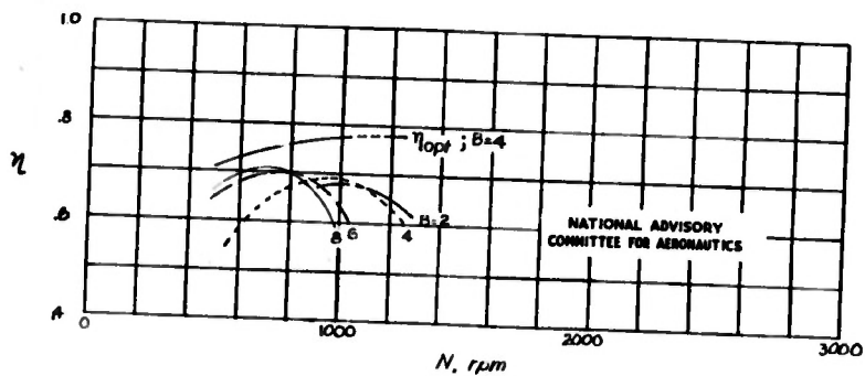
Figure 16.- Propeller efficiency. V = 50 miles per hour; P = 100 horsepower; \sigma_{0.7R} = 0.03458 .
