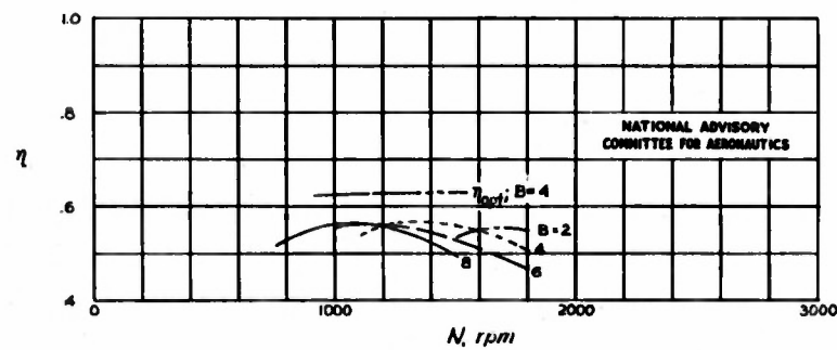
Figure 4.- Propeller efficiency. V = 50 miles per hour; P = 300 horsepower; \sigma_{0.7R} = 0.0345B .
