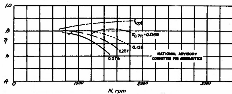
Figure 2.- Propeller efficiency. V = 100 miles per hour; P = 300 horsepower; B = 4 .
