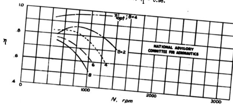
Figure 18.- Propeller efficiency. V = 150 miles per hour; P = 100 horsepower; \sigma_{0.7R} = 0.03458 .
