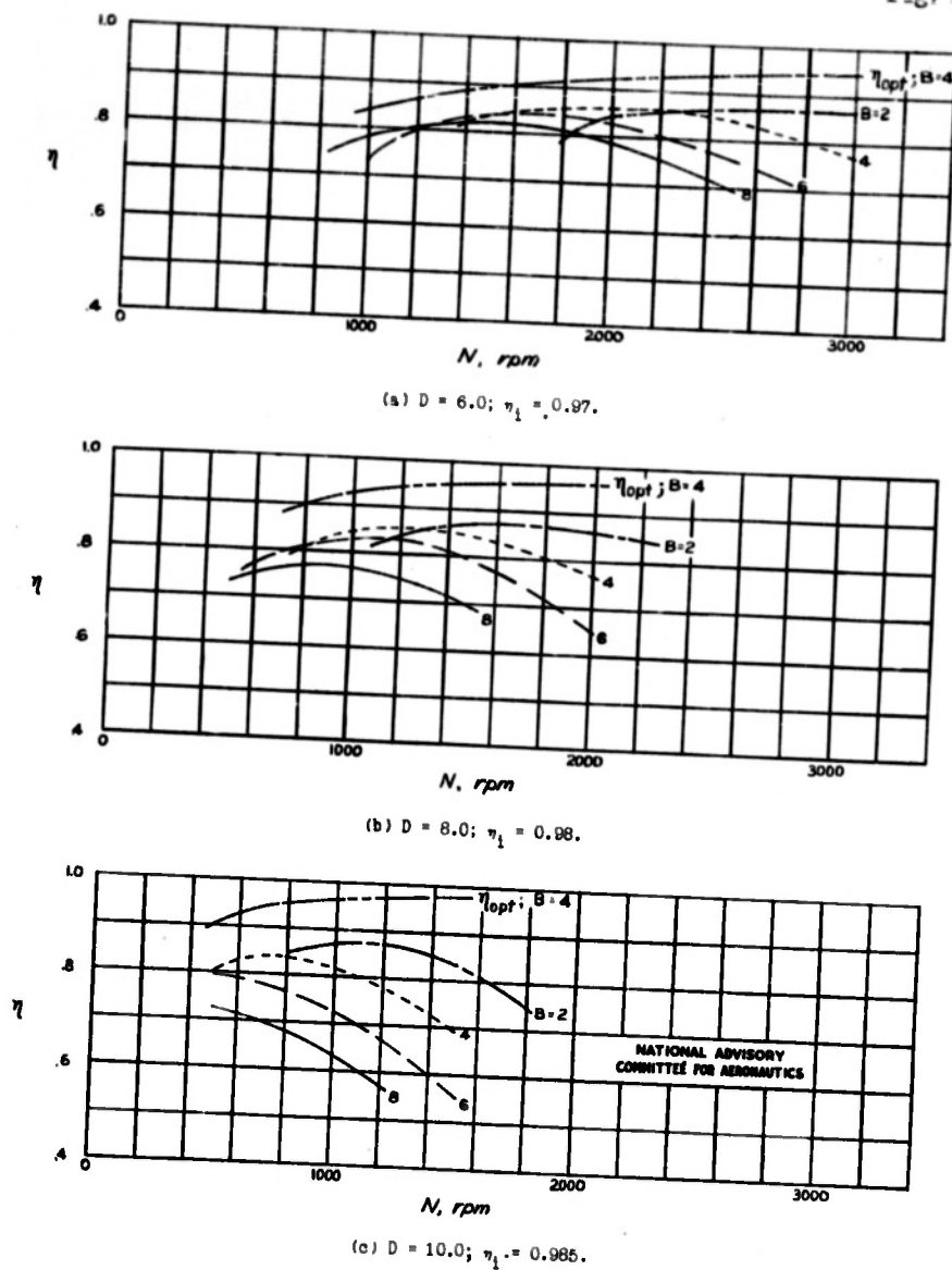
Figure 11.- Propeller efficiency. V = 200 miles per hour; P = 225 horsepower; \sigma_{0.7R} = 0.0345B .
