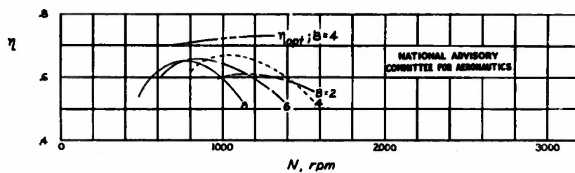
Figure 12.- Propeller efficiency. V = 50 miles per hour; P = 150 horsepower; \sigma_{0.7R} = 0.0345B .
