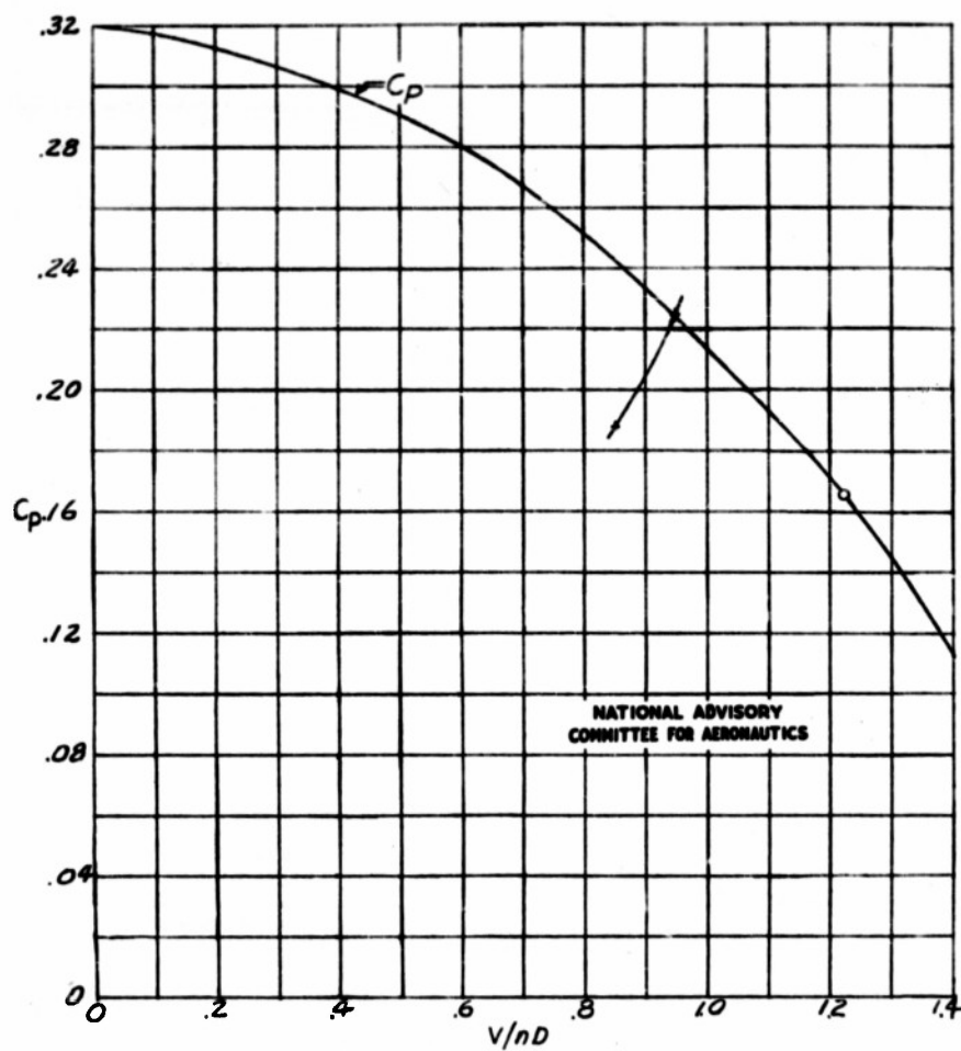
Figure 24.- Power-coefficient curve for use in fixed-pitch analysis.
