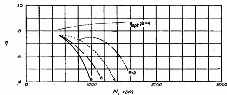
Figure 20.- Propeller efficiency. V = 50 miles per hour; P = 50 horsepower; \sigma_{0.7R} = 0.0345B .
