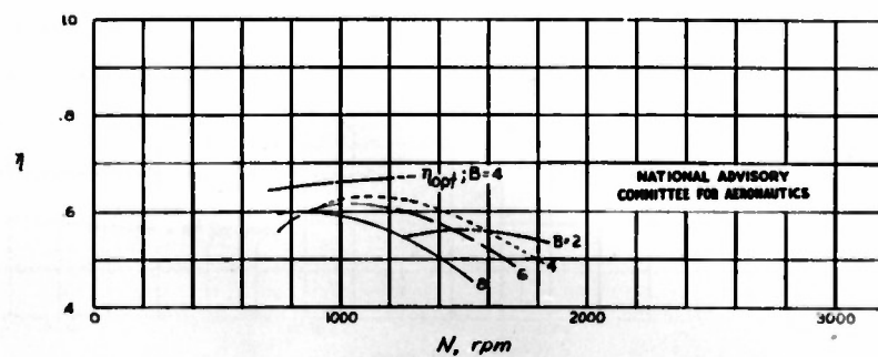
Figure 8.- Propeller efficiency. V = 50 miles per hour; P = 225 horsepower; \sigma_{0.7R} = 0.0345B .
