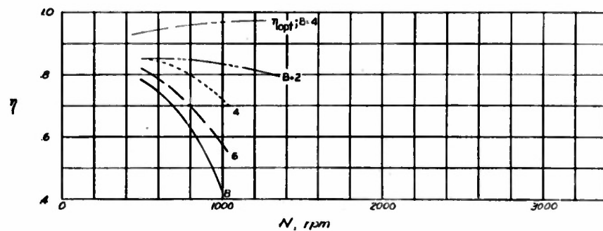
Figure 21.- Propeller efficiency. V = 100 miles per hour; P = 50 horsepower; \sigma_{0.7R} = 0.03458 .
