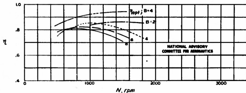
Figure 6.- Propeller efficiency. V = 150 miles per hour; P = 300 horsepower; \sigma_{0.7R} = 0.03455 .
