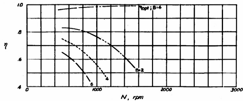
Figure 22.- Propeller efficiency. V = 150 miles per hour; P = 50 horsepower; \sigma_{0.7R} = 0.0345B .
