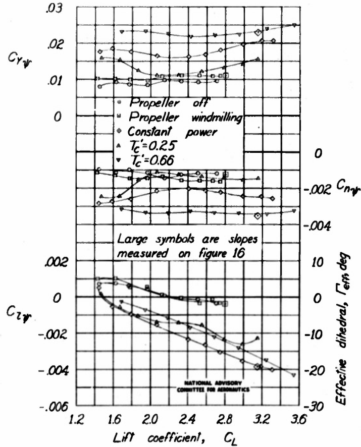
Figure 10.-Effect of power on the variation of C_{L\gamma} , C_{N\gamma} , and C_{Y\gamma} with lift coefficient for the model as a single-engine high-wing airplane with a full-span double slotted flap. Tail on.
