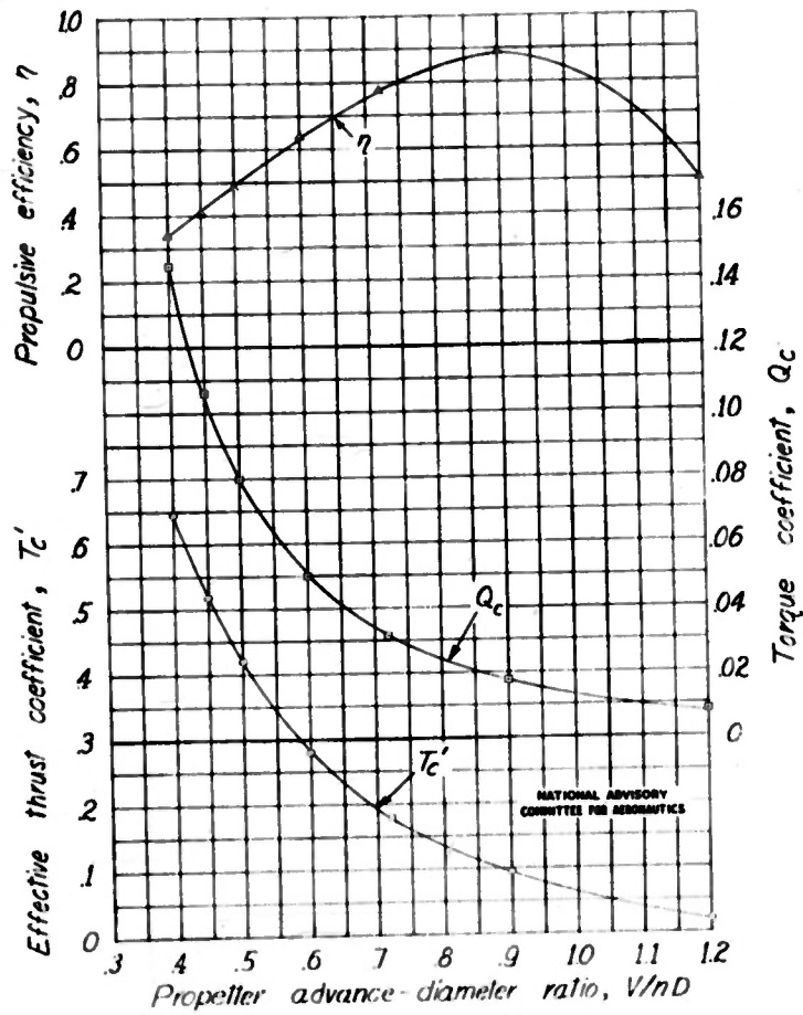
Figure 5.-Effective thrust coefficient, torque coefficient, and efficiency as functions of propeller advance-diameter ratio for the model as a high-wing airplane. D = 2.0 feet; \beta = 25^\circ .
