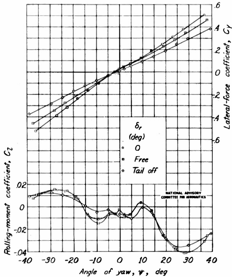
Figure 16.- Aerodynamic characteristics in yaw of the model as a single-engine high-wing airplane with full-span double slotted flap. \alpha \approx 9.4^\circ .
