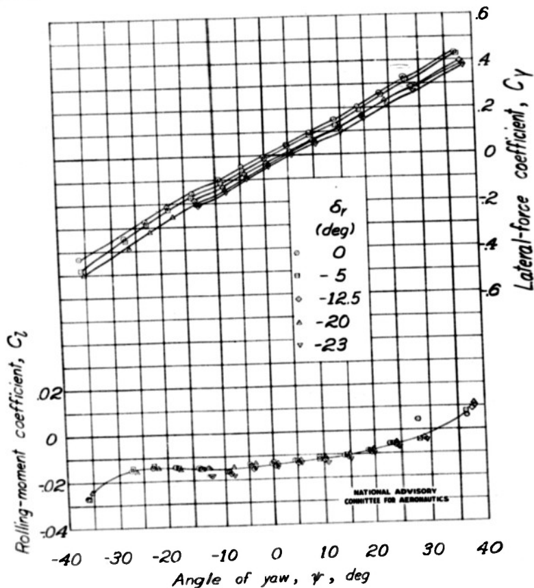
Figure 18.-Effect of rudder deflection on the aerodynamic characteristics of the model as a single-engine high-wing airplane with full-span single slotted flap. \alpha \approx 9.6^\circ .
