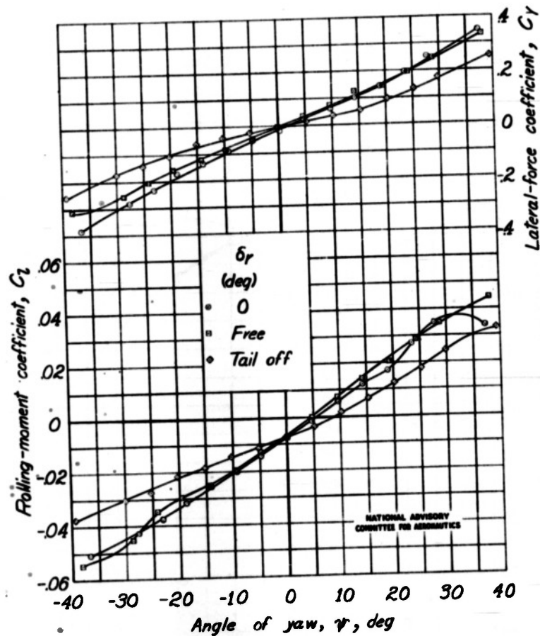
Figure 14.- Aerodynamic characteristics in yaw of the model as a single-engine high-wing airplane with flap neutral. \alpha \approx 1.7^\circ
