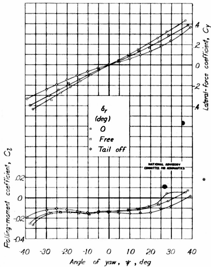
(a) Propeller windmilling. Figure 15.- Aerodynamic characteristics in yaw of the model as a single-engine high-wing airplane with the full-span single slotted flap. \alpha \approx 9.6^\circ .
