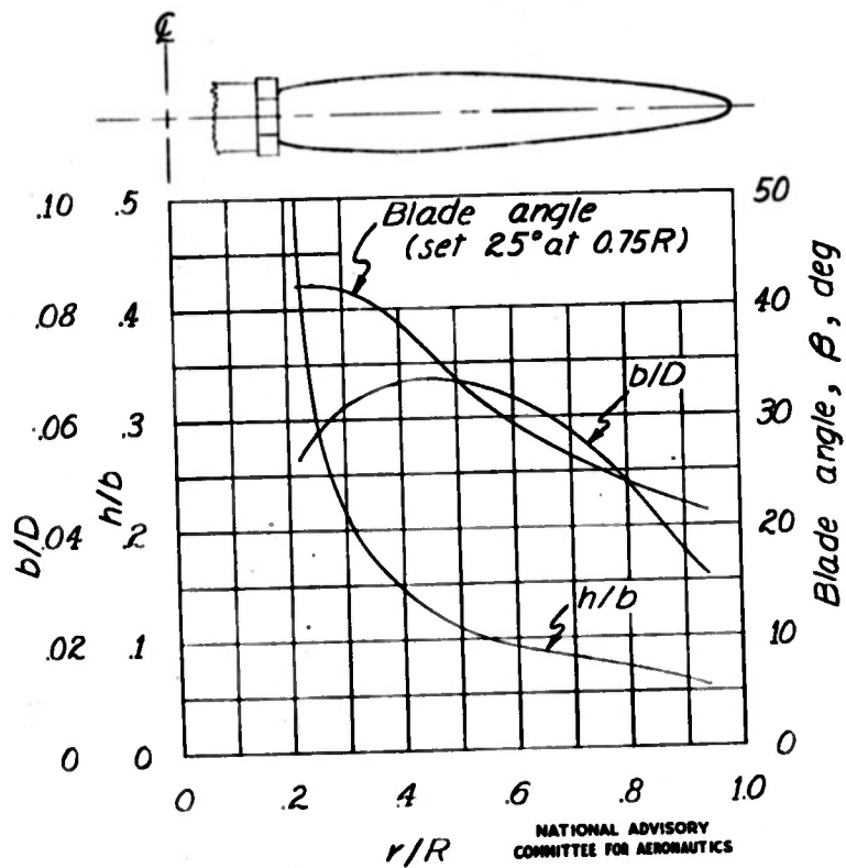
Figure 4.-Plan-form and blade-form curves for the model propeller. D , diameter; R , radius to tip; r , station radius; b , section chord; h , section thickness; RAF 6 airfoil section.
