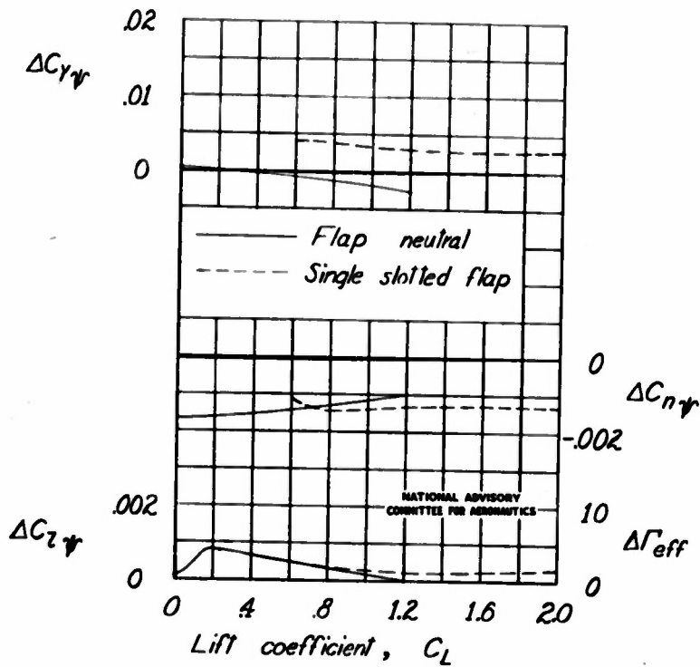
Figure 13.-Increments in C_{z\psi} , C_{n\psi} , and C_{y\psi} contributed by the tail surfaces for the model as a single-engine high-wing airplane.
