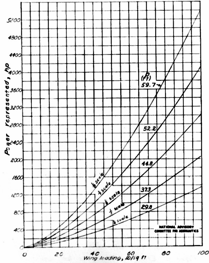
Figure 7.- Variation of approximate horsepower represented with airplane wing loading for various model scales.
