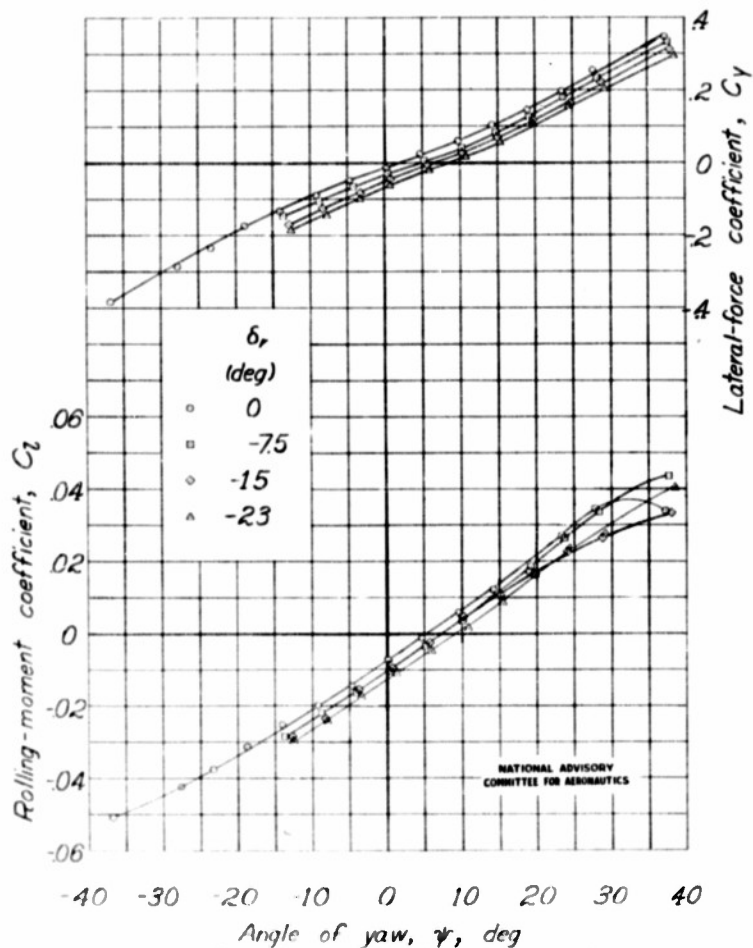
(a) Propeller windmilling. Figure 17. -Effect of rudder deflection on the aerodynamic characteristics of the model as a single-engine high-wing airplane with flap neutral. \alpha \approx 1.7^\circ .
