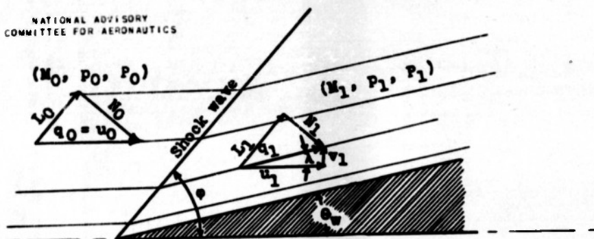
Figure 1.- Supersonic flow over inclined plane surface of infinite span and chord.
