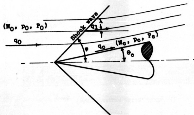
Figure 2.- Supersonic flow over axially symmetric cone.
