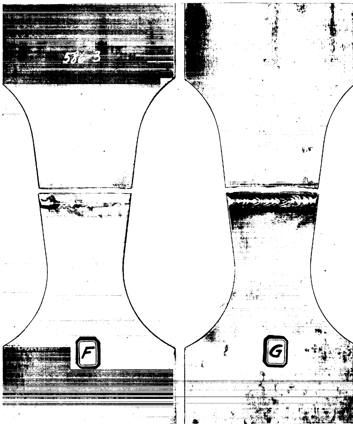
Continuous single-bead weld (root side). Failure at toe of face bead.
