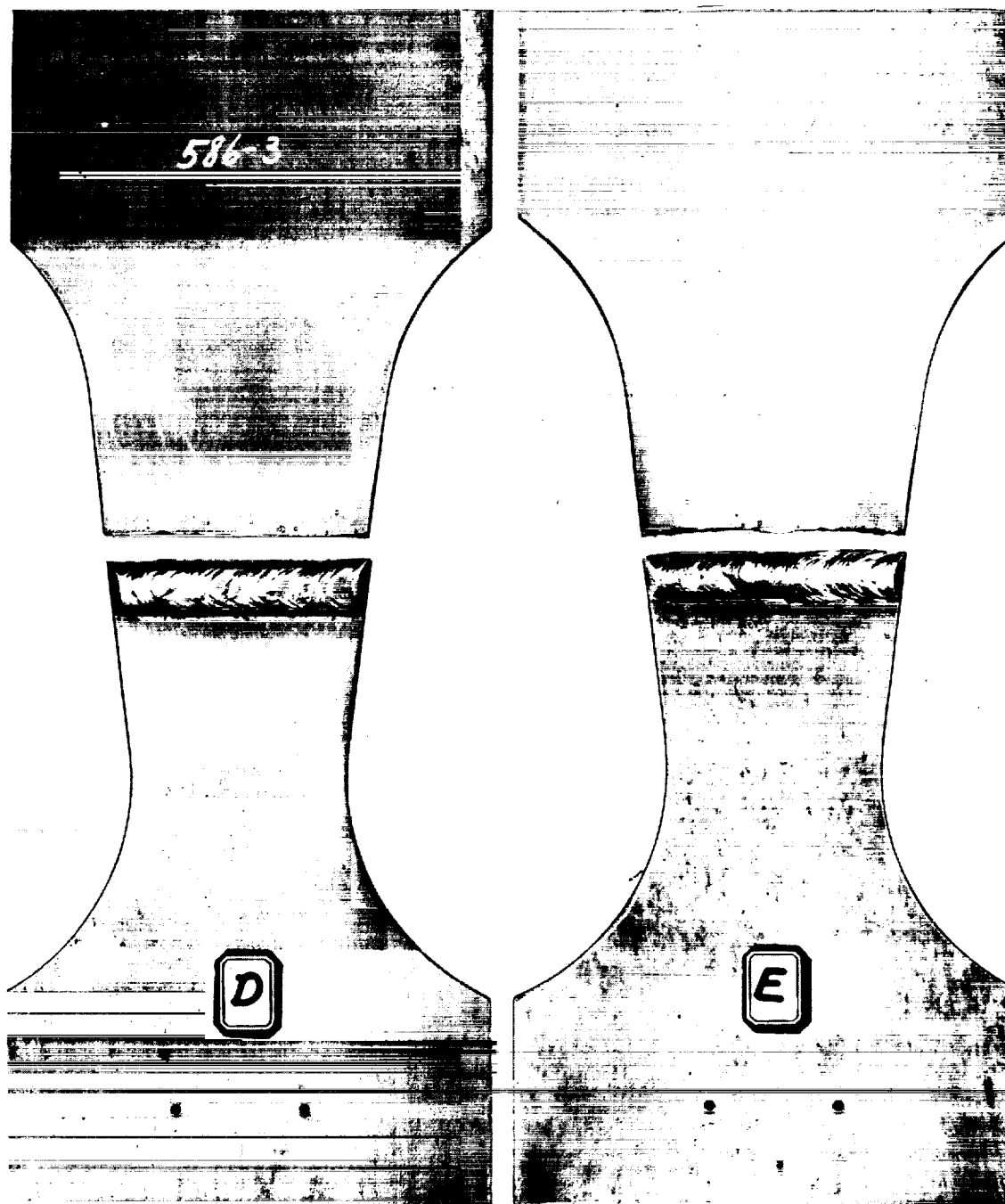
Continuous single-bead weld (face side).
