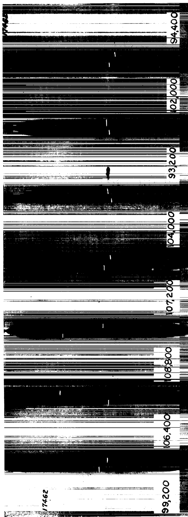
Figure 5.—Radiograph of metal-arc-welded static tension specimens in \frac{1}{8} -inch SAE 4130 sheet.
