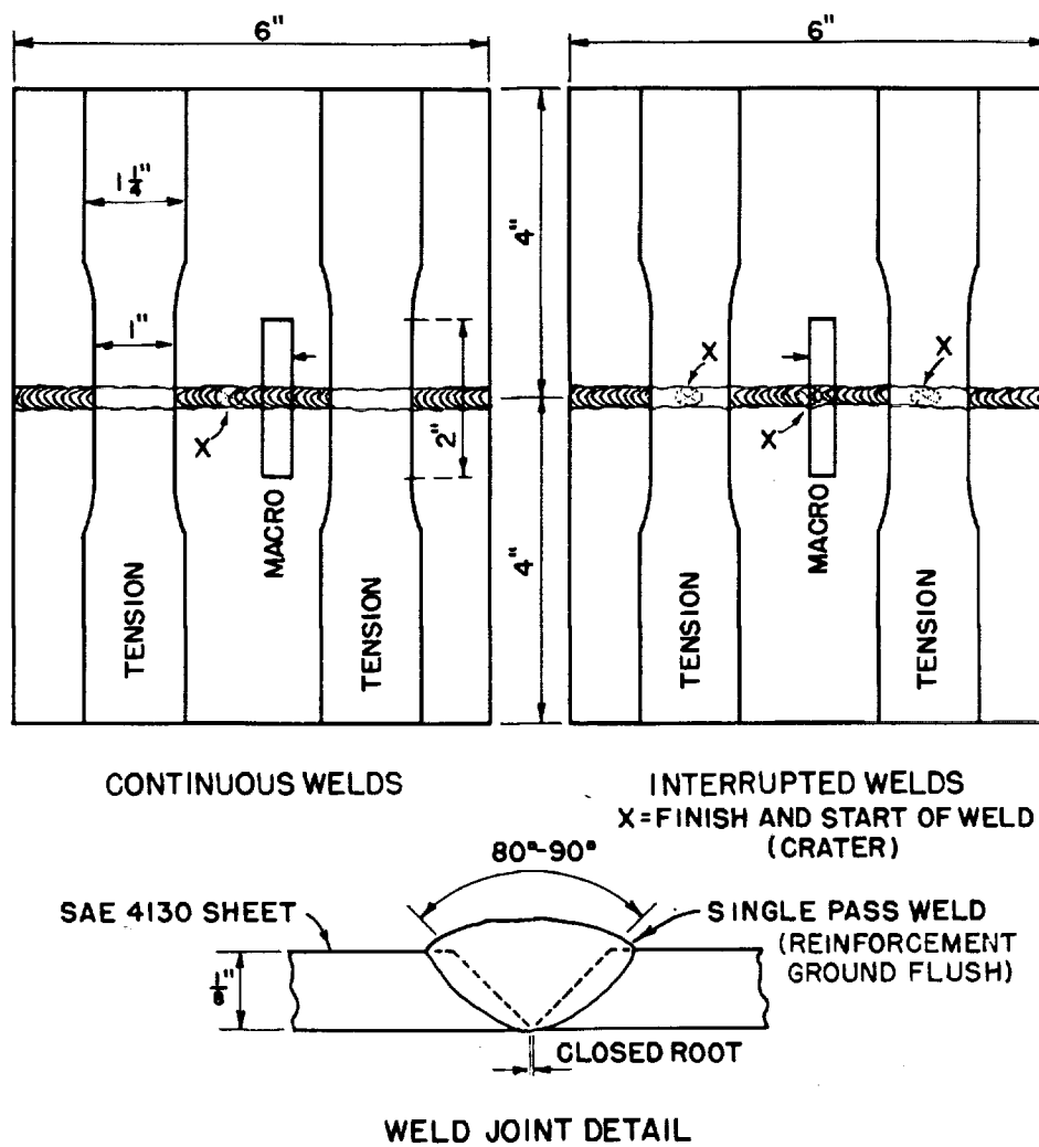
FIGURE 1— BUTT-WELDED SPECIMEN FOR STATIC TENSION TESTS OF JOINTS WITH CONTINUOUS AND INTERRUPTED WELDS.
