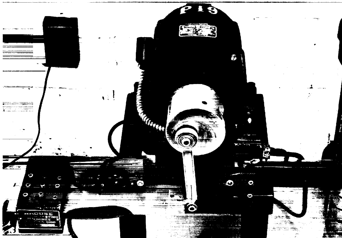
Figure 20.—Krouse plate-bending machine with welded specimen in place for fatigue test.
