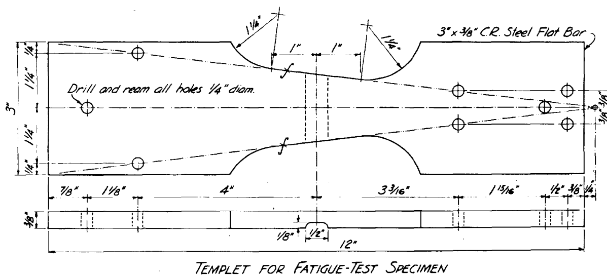
FIGURE 19- SPECIMEN AND TEMPLT FOR PLATE BENDING-FATIGUE TEST
