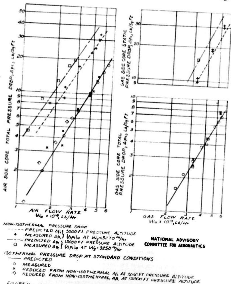
FIGURE 16.—COMPARISON OF ISOTHERMAL AND REDUCED NON-ISOTHERMAL PRESSURE DROP DATA FOR UNTINNED HEAT EXCHANGER AT STANDARD CONDITIONS, 59°F AND 167°F.
