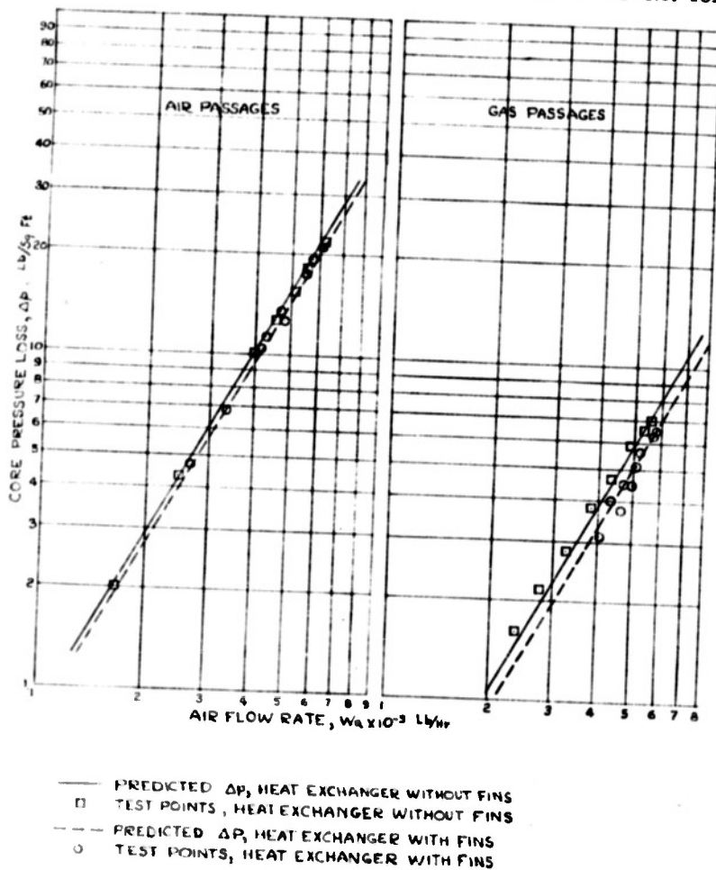
FIGURE 17.- COMPARATIVE CORE PRESSURE DROPS OF FINNED AND UNFINNED HEAT EXCHANGERS AT STANDARD CONDITIONS, 59°F AND 14.7 3 / 32 in. Hg.
