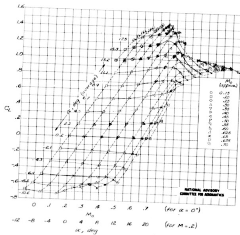
Figure 3 - Wing lift coefficient as a function of angle of attack and Mach number. (From reference 1)
