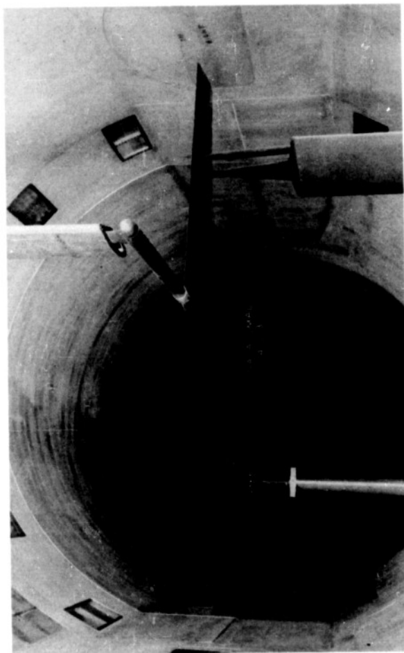
Figure 2.- Rear view of wing mounted in the tunnel for the pressure-distribution tests.
