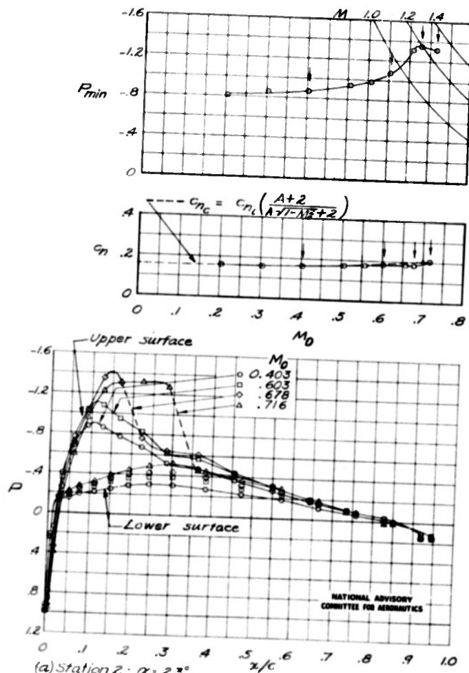
(a) Station 2; \alpha = 2.3^\circ . Figure 4.- Pressure distributions over stations 2 and 3 of fighter-type wing, with curves of minimum pressure coefficient and normal-force coefficient against Mach number.
