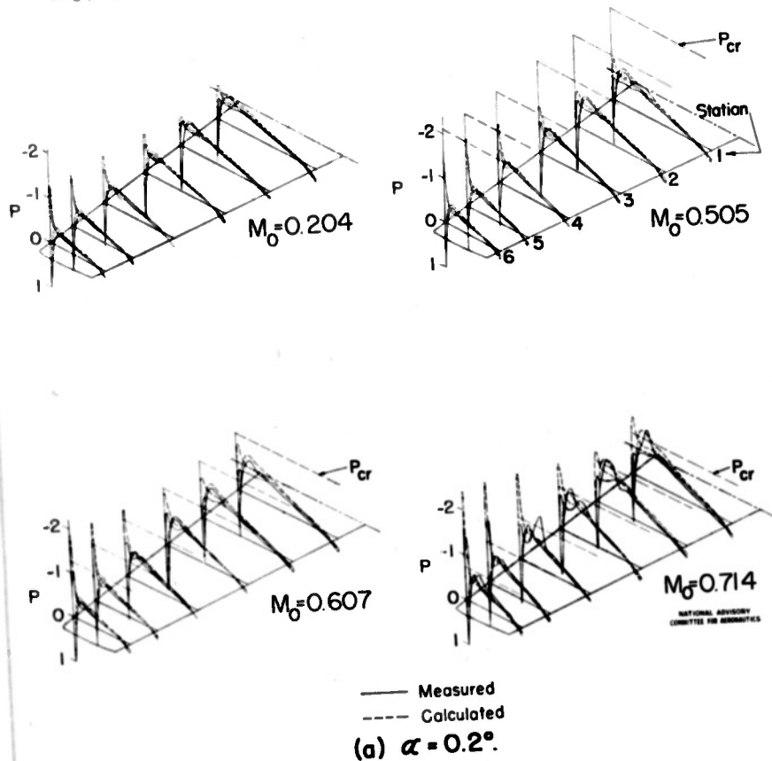
Figure 7.-Measured and calculated pressure distributions about fighter-type wing at various Mach numbers and angles of attack.
