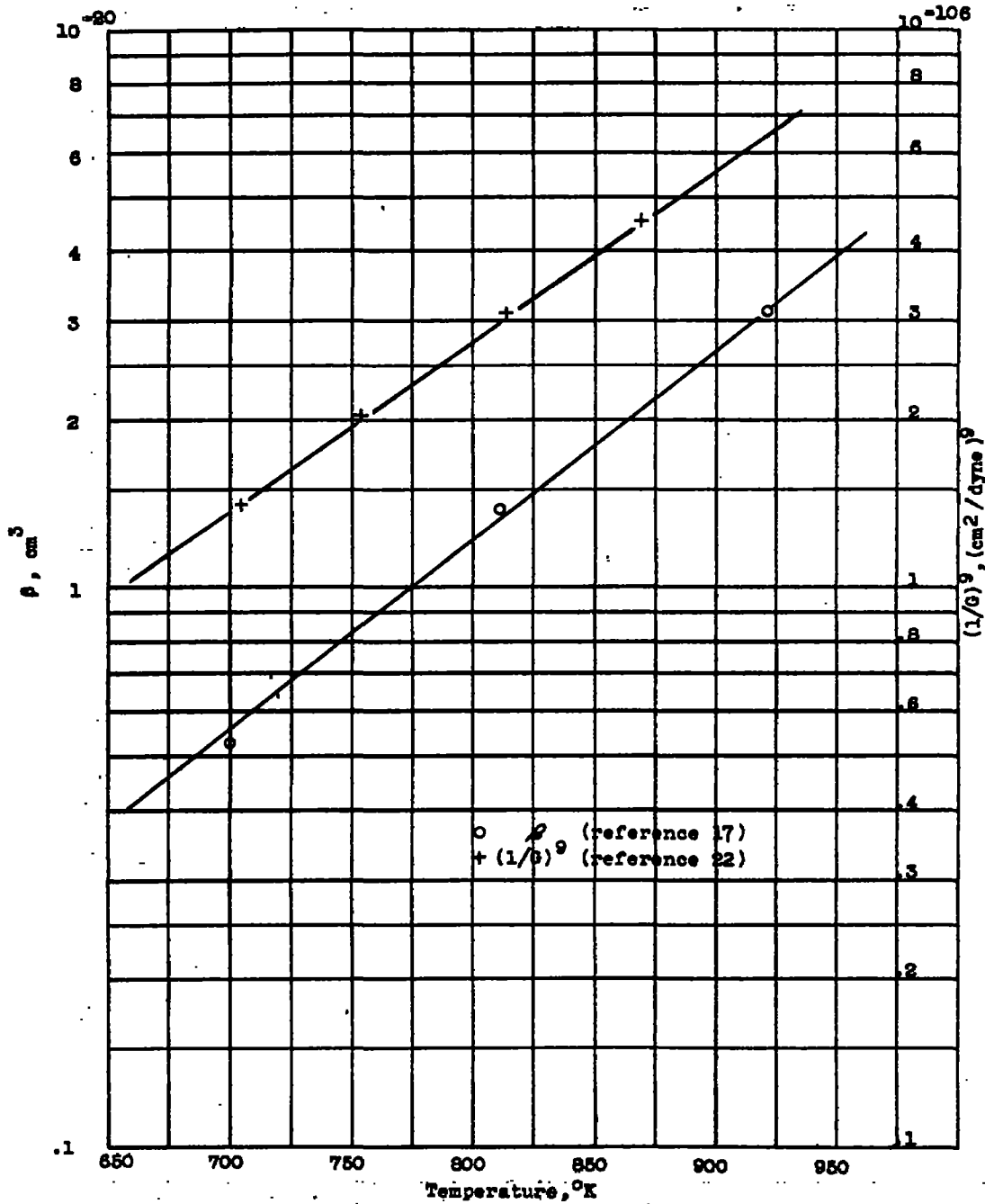
Figure 8.- Temperature dependence of \beta and 1/\beta for iron.
