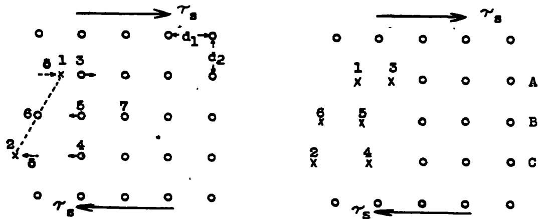
(a) Activated complex for a positive dislocation.
