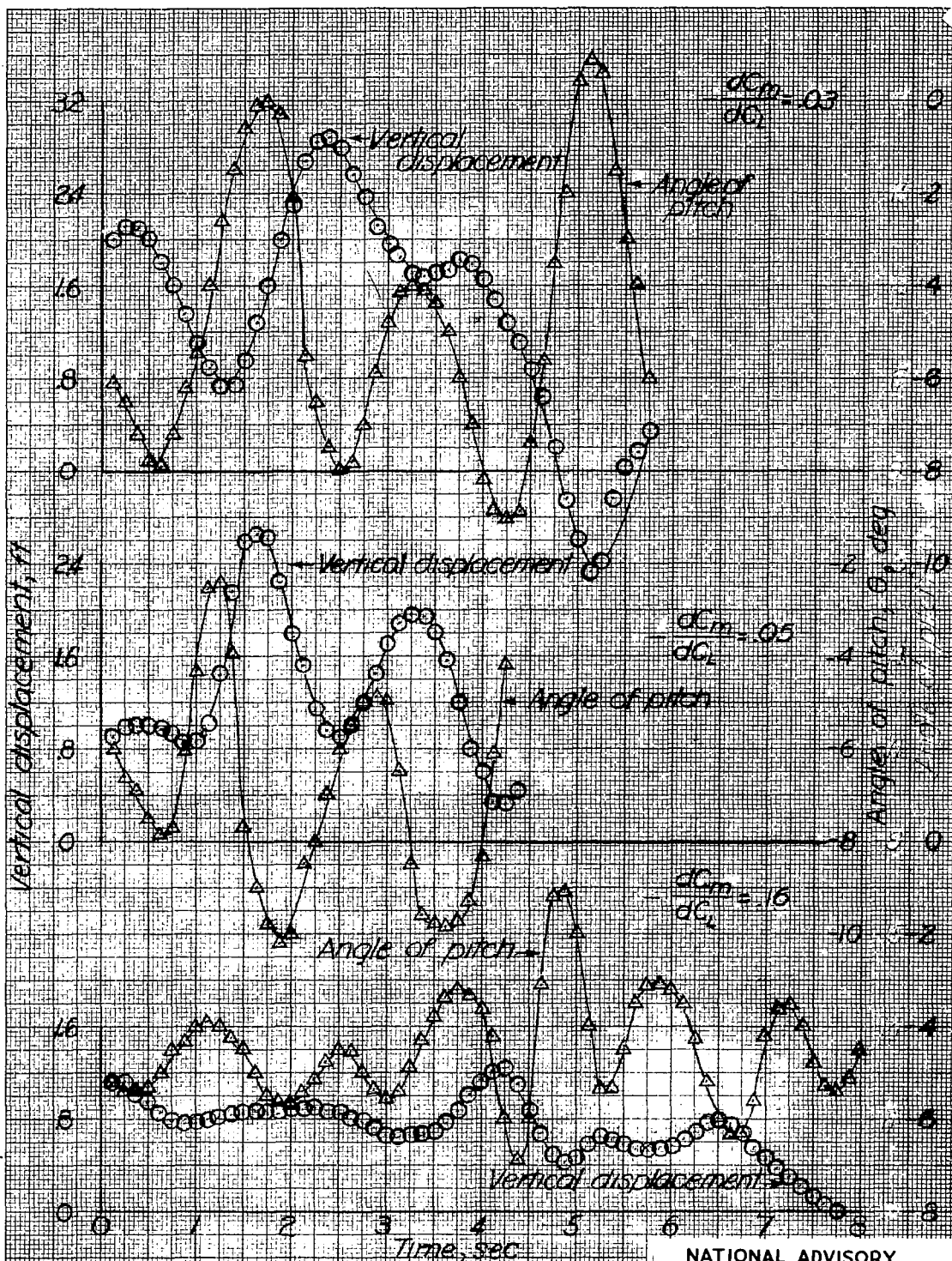
Figure 5 - Typical motion-picture records of model motions. Large tail (tail 1), C_{m_0} = -14.3 , C_L = 0.5 ; model controlled by Elevator.
