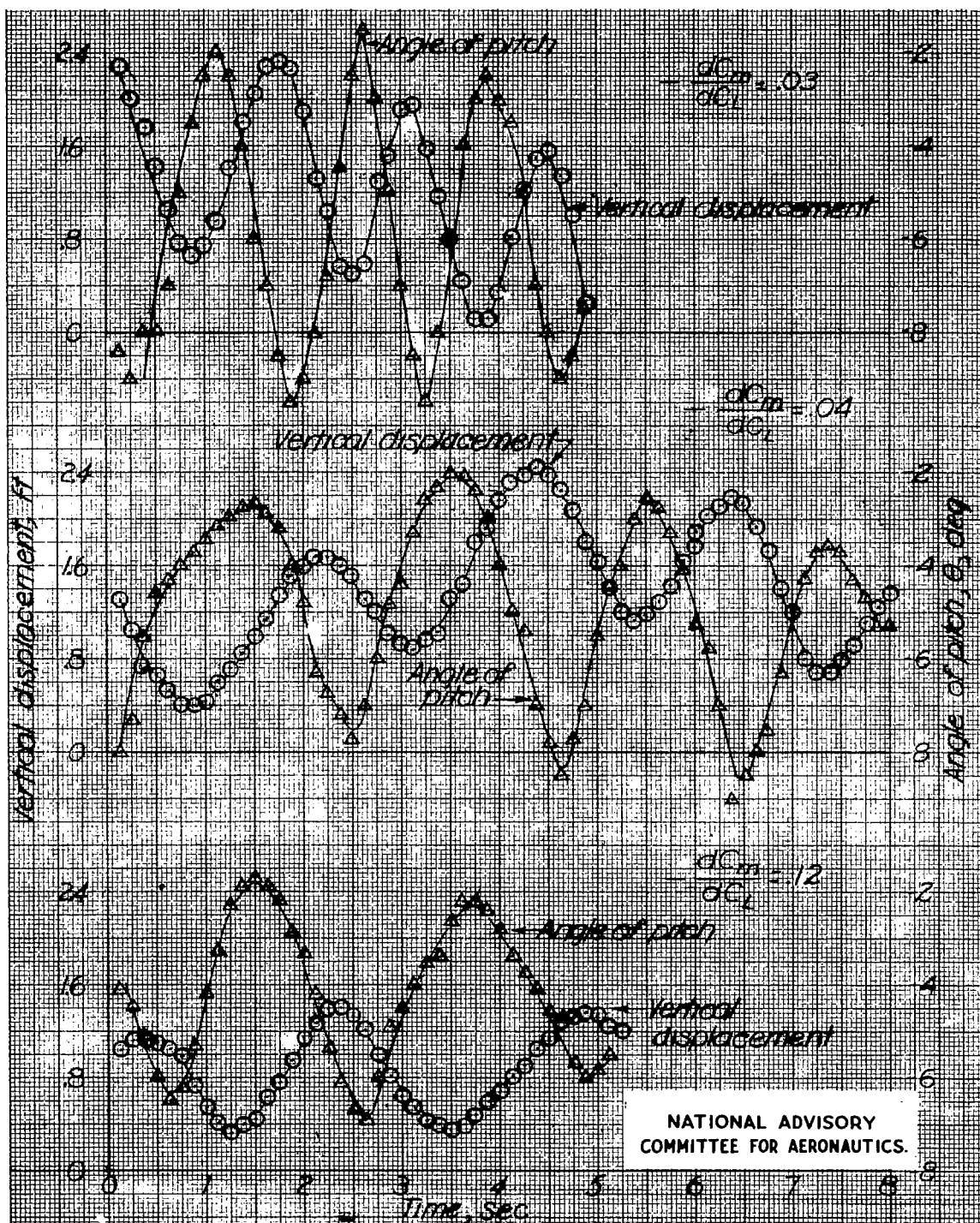
Figure 6.- Typical motion-picture records of model motions. Small tail (tail 3). C_{m4} = -7.6 ; C_L = 0.5 , model controlled by elevator.
