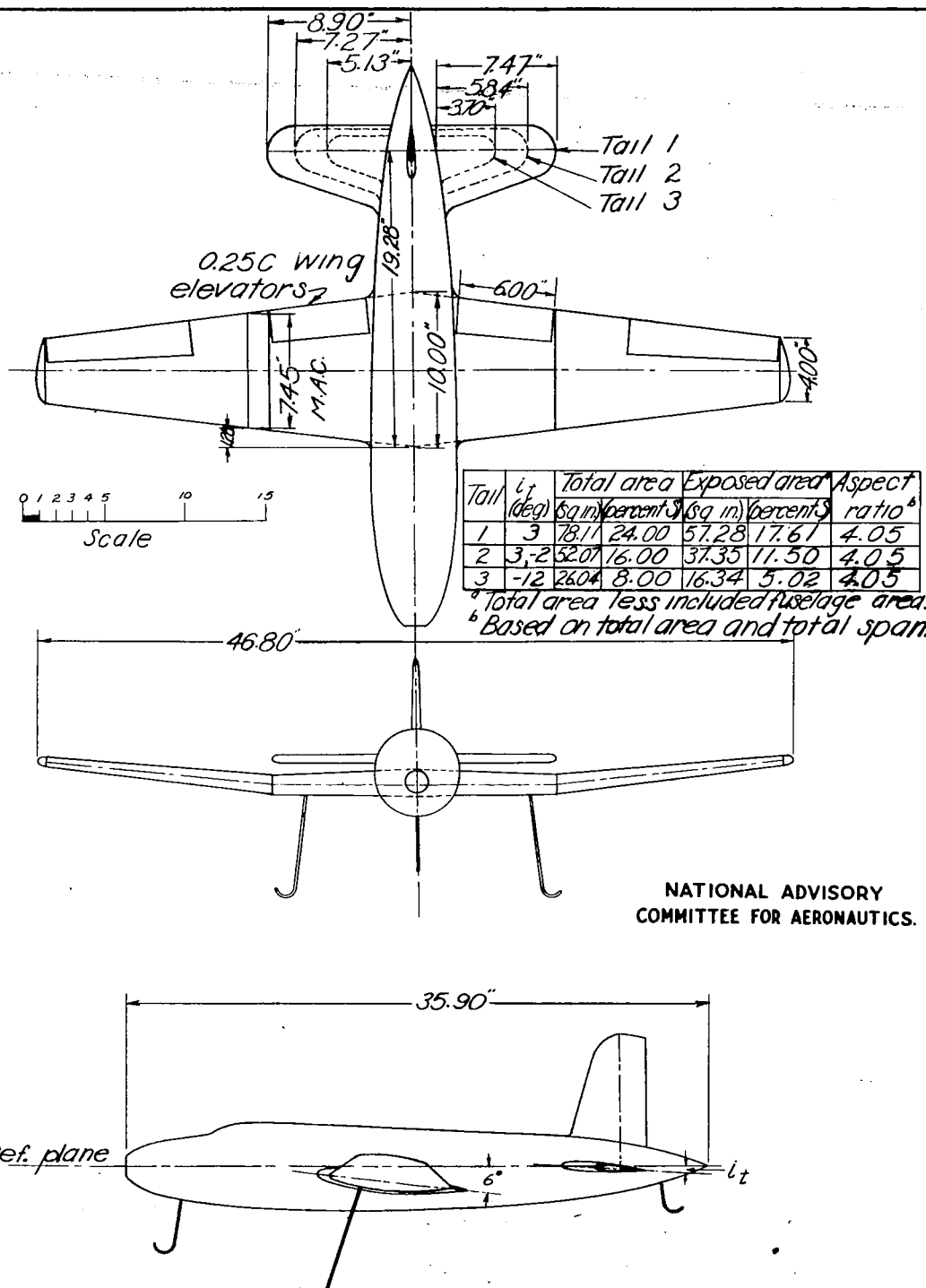
Figure 2.-Model used in free-flight-tunnel longitudinal-stability investigation.
