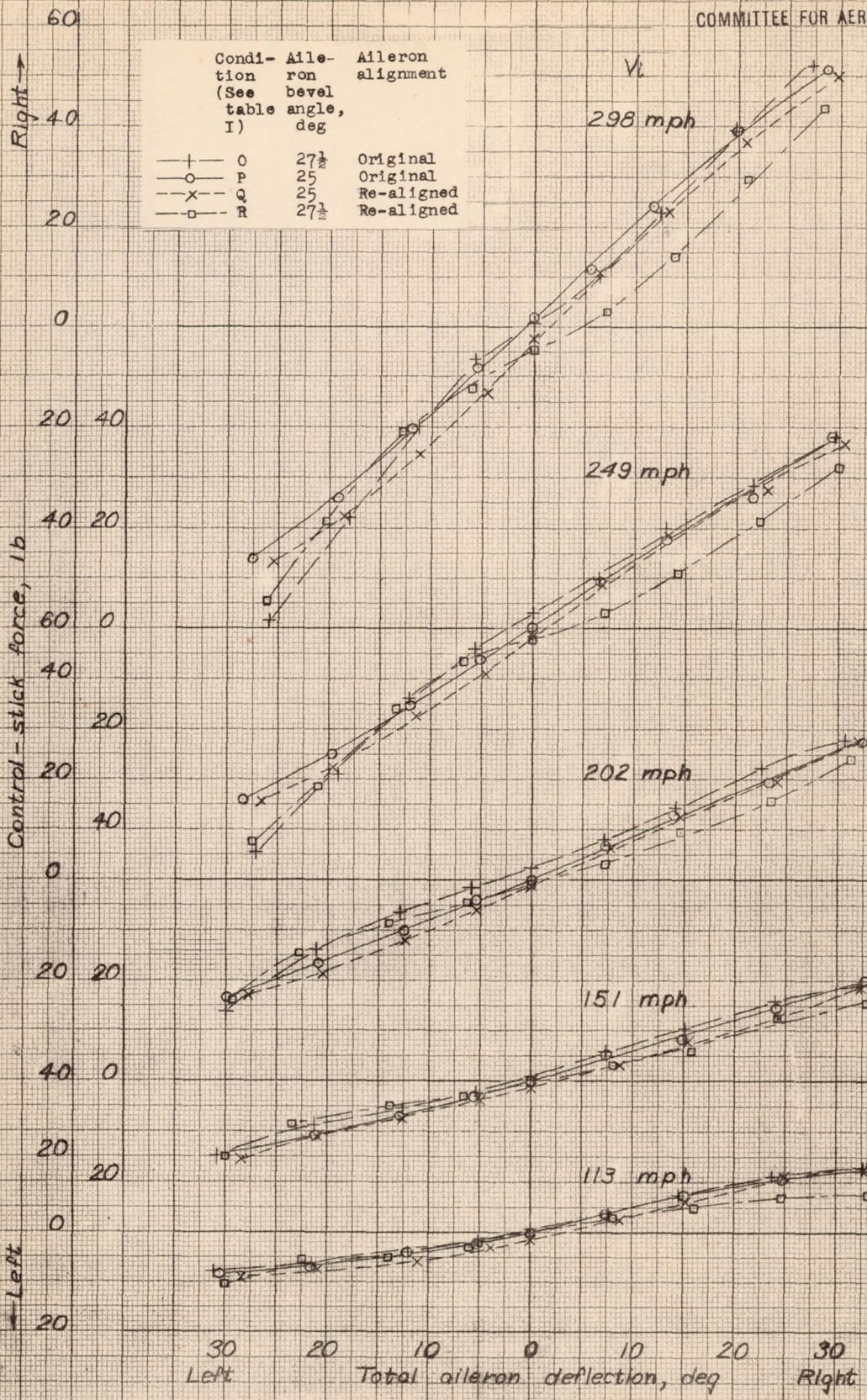
Figure 10- Effect of bevel angle and aileron alignment on stick-force characteristics of beveled trailing-edge ailerons North American XP-51 airplane
