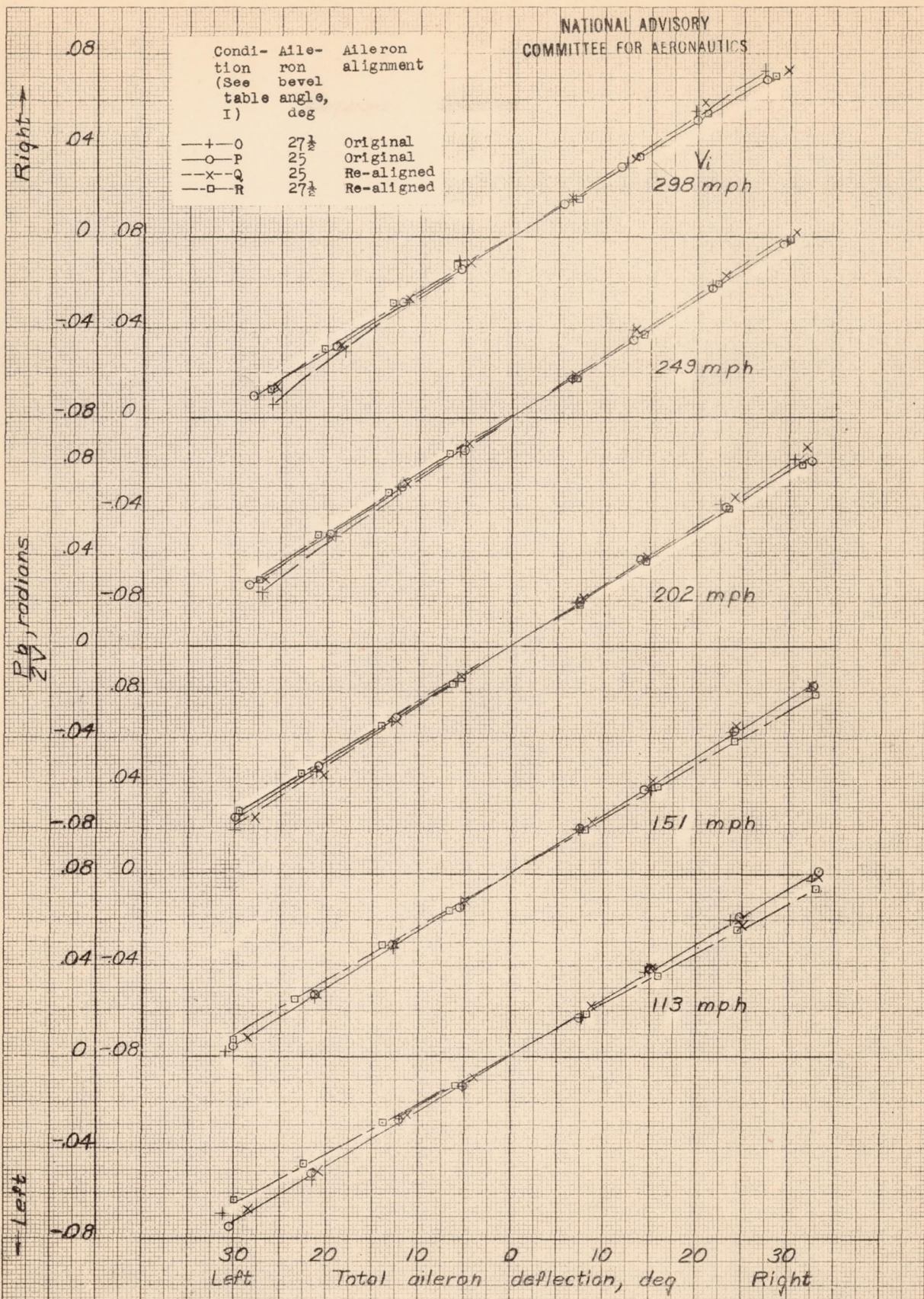
Figure 11.-Effect of bevel angle and aileron alignment on effectiveness characteristics of beveled trailing-edge ailerons North American XP-51 airplane
