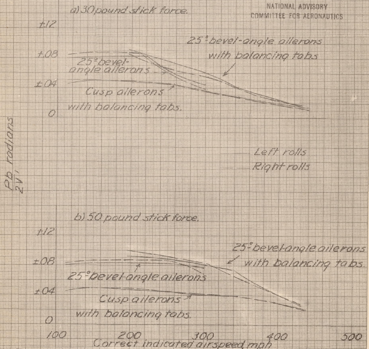
Figure 19. - Comparison of aileron characteristics of 25° bevel-angle ailerons, cusp ailerons with balancing tabs, and 25° bevel-angle ailerons with balancing tabs. Data from figures 17 and 18. North American XP-51 airplane.
