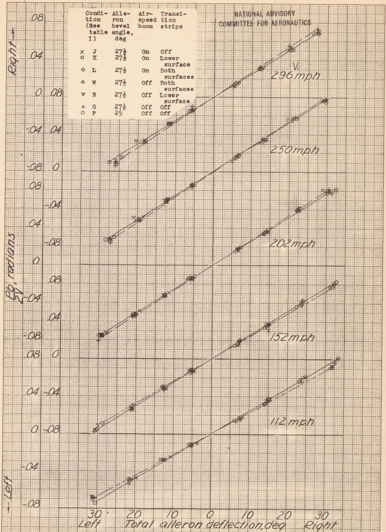
Figure 25.-Effect of airspeed boom and transition strips on the aileron-effectiveness characteristics of 27½° bevel angle ailerons. North American XP-51 airplane
