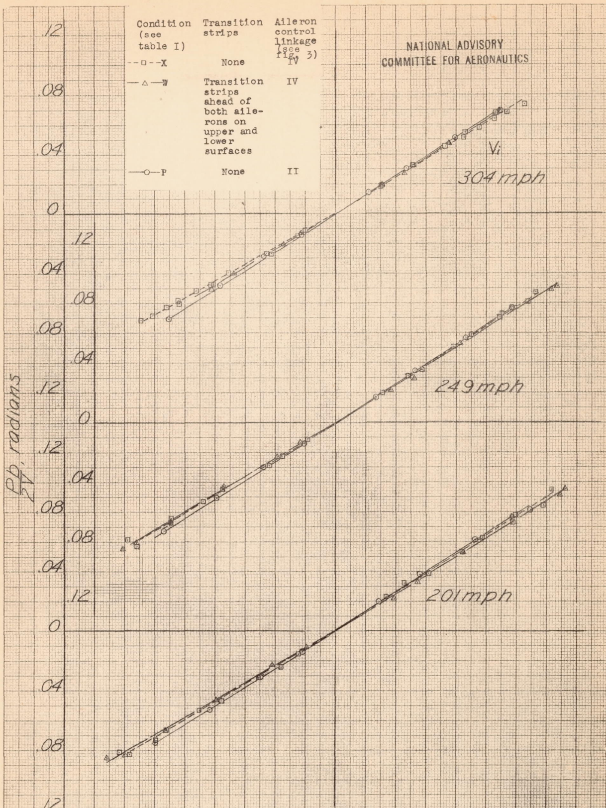
Figure 27.- Effect of transition strips on aileron-effectiveness characteristics of beveled trailing-edge ailerons. 25° bevel-angle ailerons with balancing tabs. North American XP-51 airplane.
