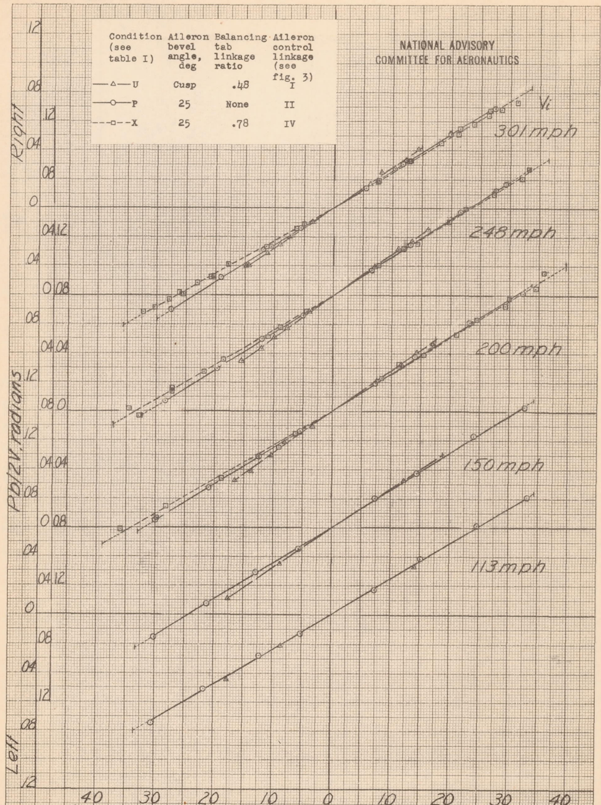
Figure 18.—Comparison of effectiveness characteristics of 25°-bevel-angle ailerons with balancing tabs, cusp ailerons with balancing tabs, and 25°-bevel-angle ailerons. North American XP-51 airplane.
