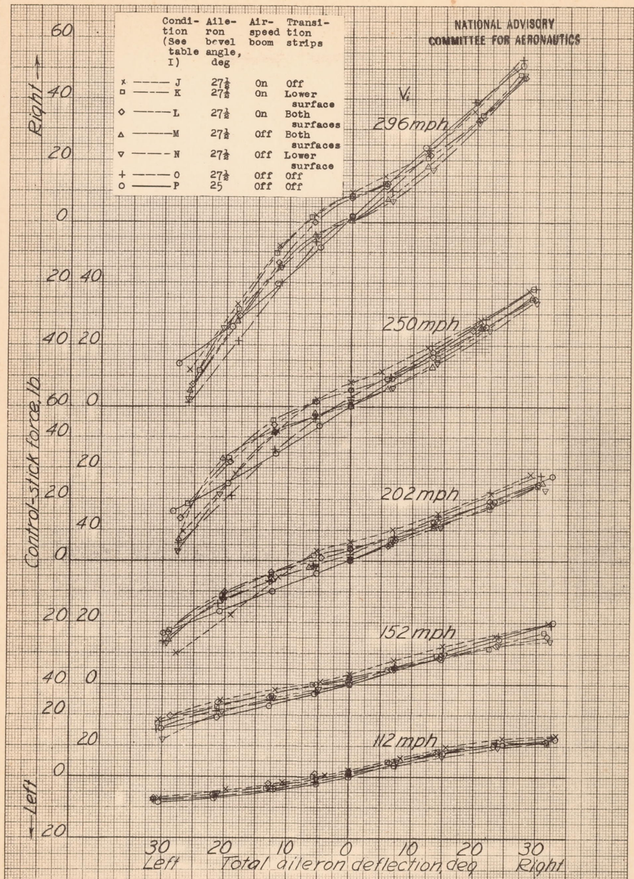
Figure 24. Effect of airspeed boom and transition strips on stick-force characteristics of 27½° bevel angle ailerons, North American XP-51 airplane.
