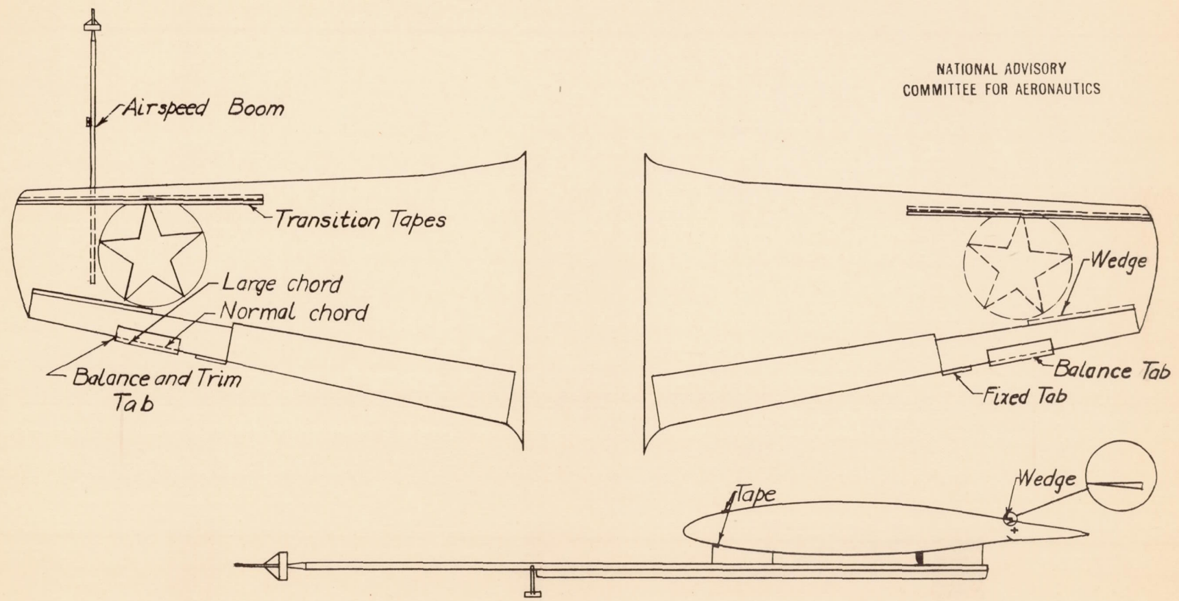
Figure 1.-XP-51 wing showing modifications
