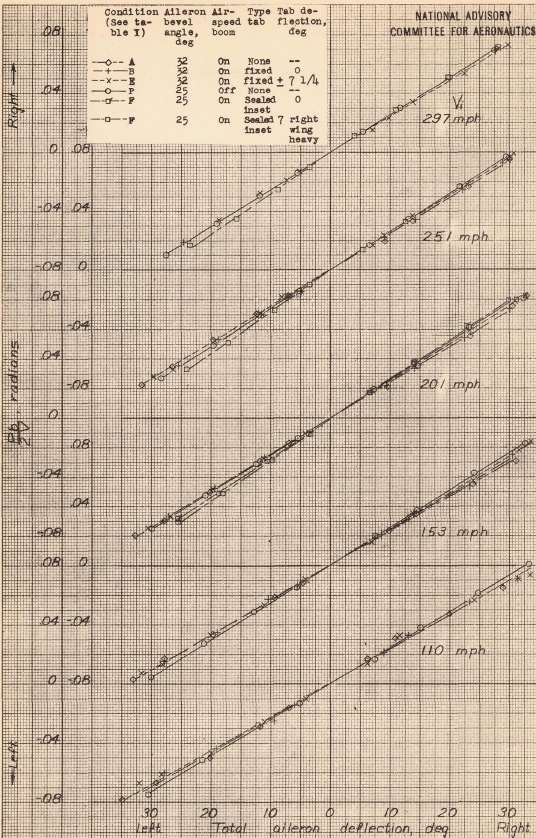
Figure 23: Aileron-effectiveness characteristics of beveled trailing-edge ailerons with fixed and inset tabs North American XP-51 airplane
