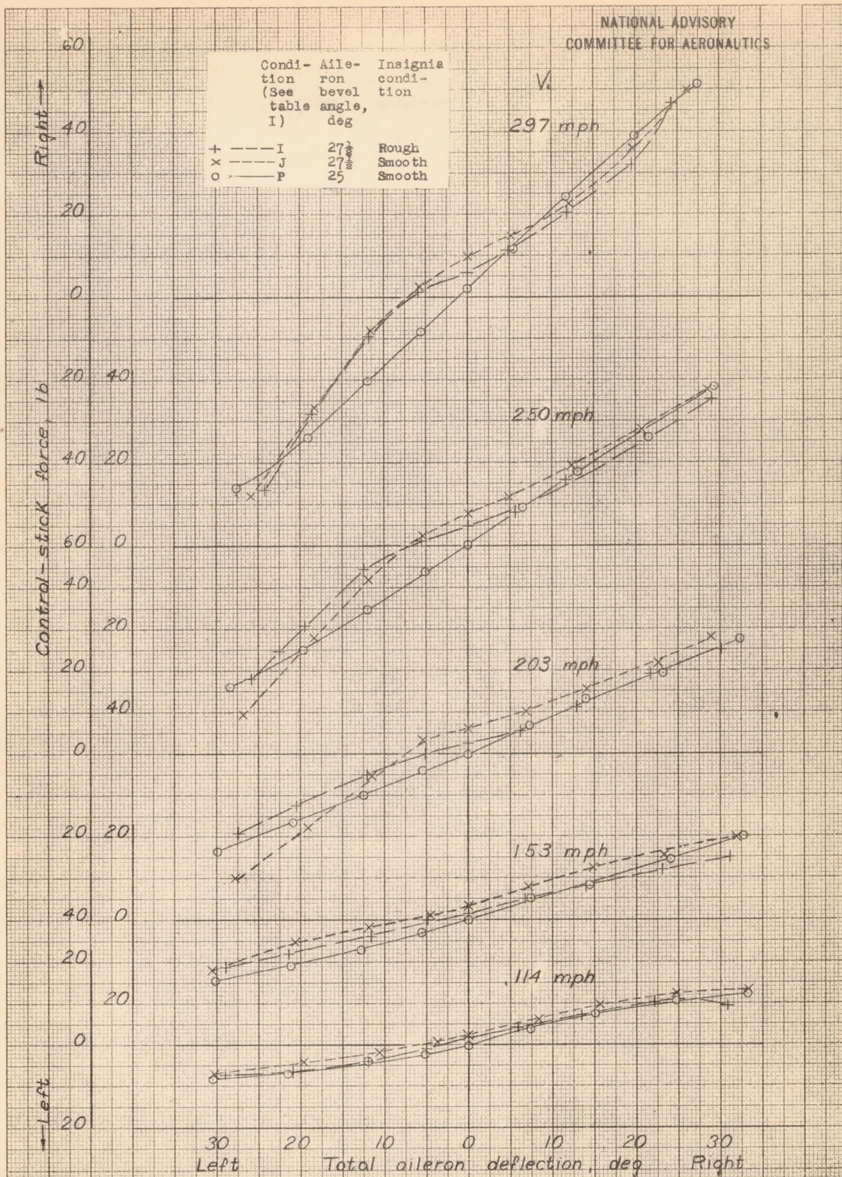
Figure 28—Effect of wing insignia on stick-force characteristics of beveled trailing-edge ailerons North American XP-51 airplane
