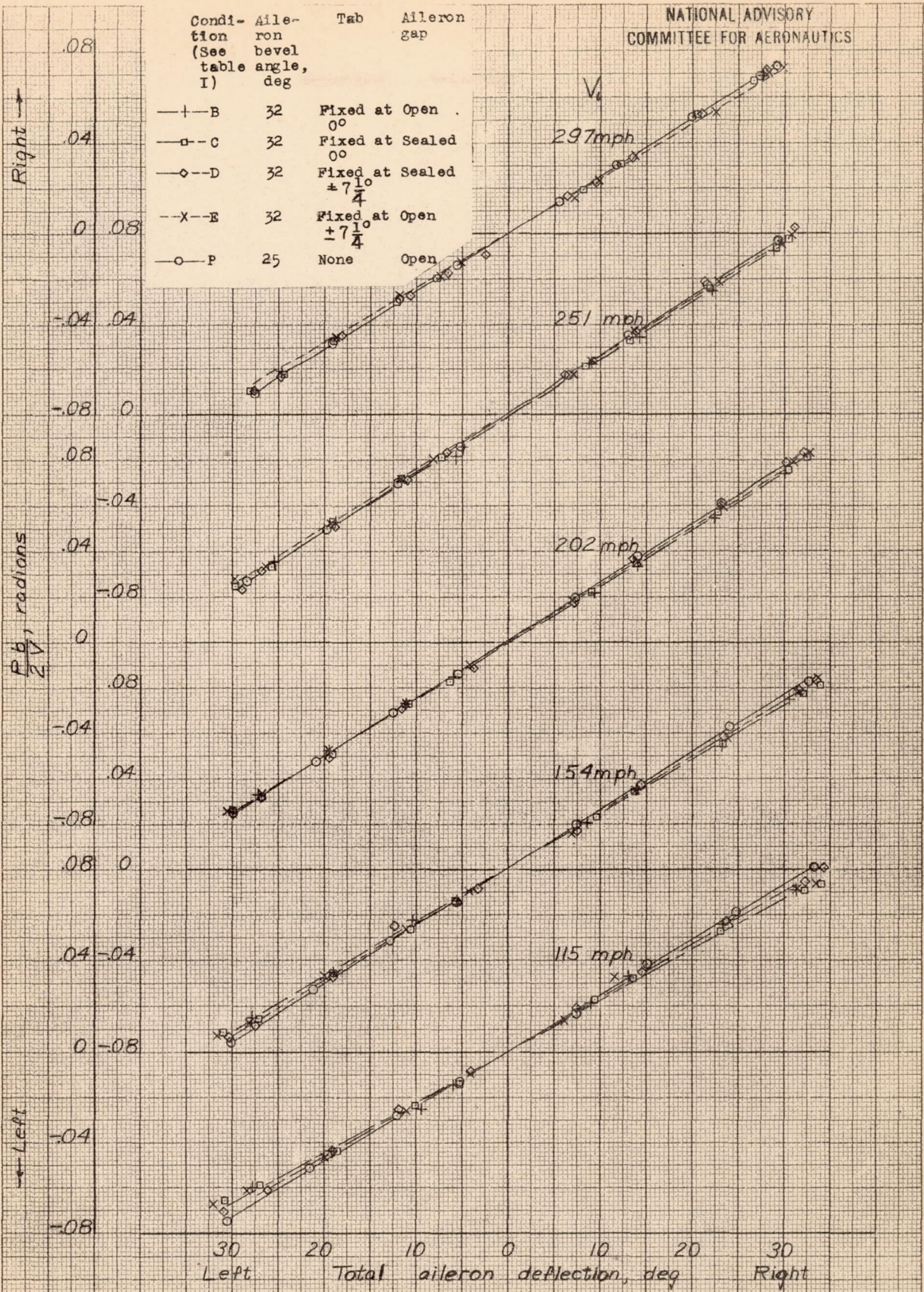
Figure 13. Effectiveness characteristics of beveled trailing-edge ailerons with sealed aileron gaps. North American XP-51 airplane
