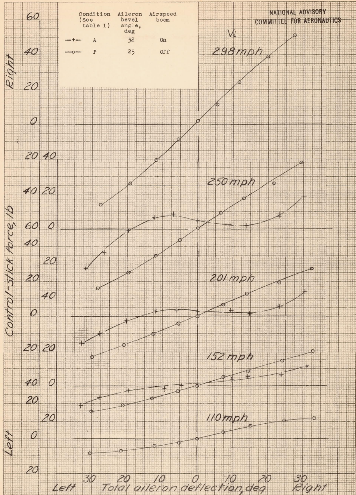
Figure 8.- Stick-force characteristics of 32°-bevel-angle ailerons. North American XP-51 airplane.
