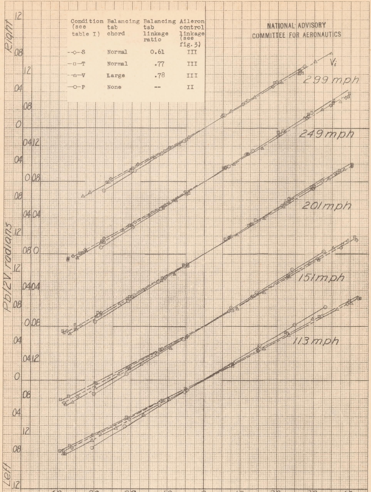
Figure 16- Effect of balancing tab linkage ratio and chord on aileron effectiveness. North American XP-51 airplane.
