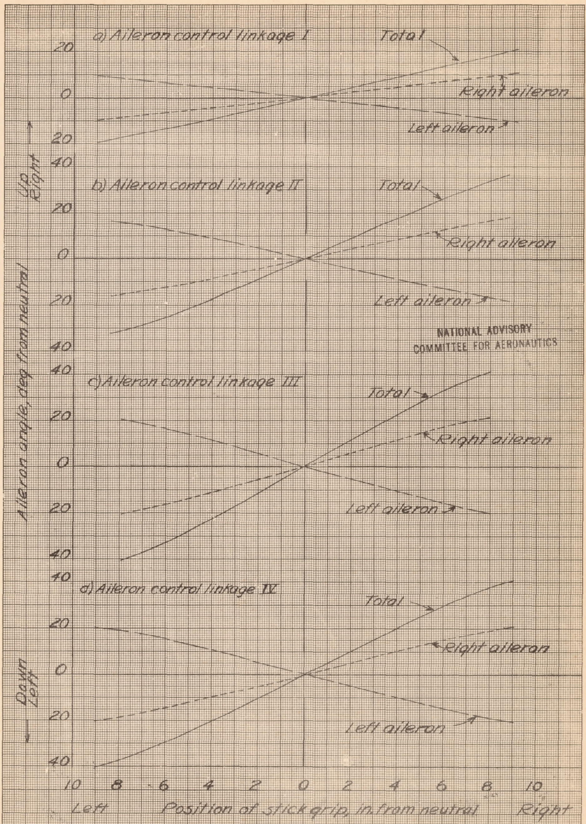
Figure 3. Relations between position of ailerons and position of stick grip under no load. North American XP-51 airplane.
