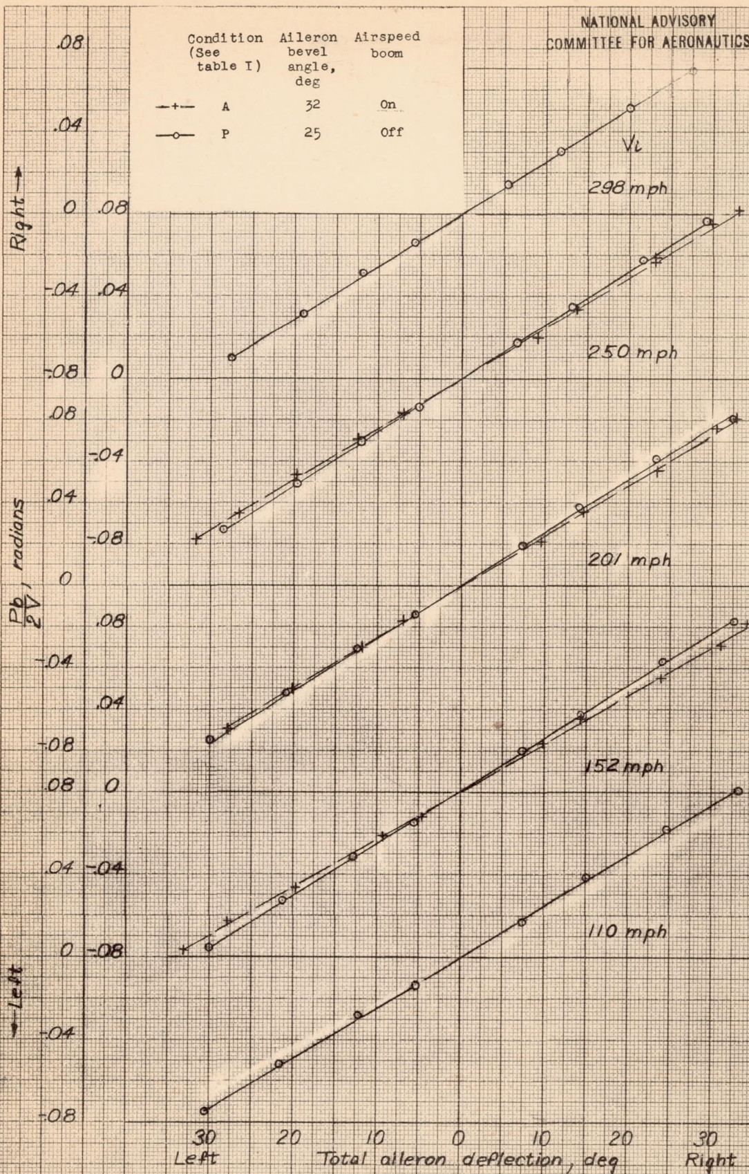
Figure 9.- Effectiveness characteristics of 32°-bevel-angle ailerons. North American XP-51 airplane.
