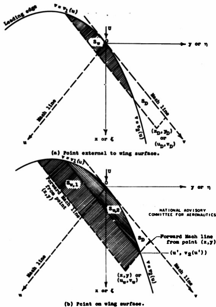
Figure 1.- Regions of integration for calculating velocity potential on surface of variably swept wing at supersonic speeds.
