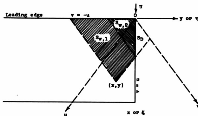
Figure 2.- Integration regions for calculating velocity potential on surface of thin flat plate wing at supersonic speeds.
