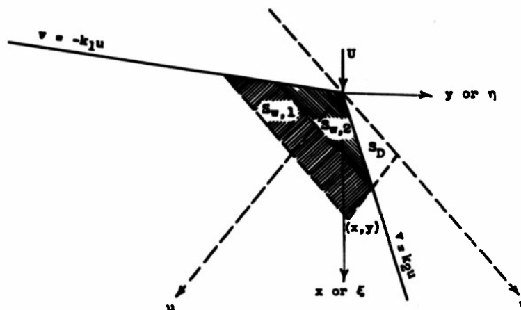
Figure 3.- Regions of integration for calculating velocity potential on surface of finite thickness, discontinuously swept wing at supersonic speeds.
