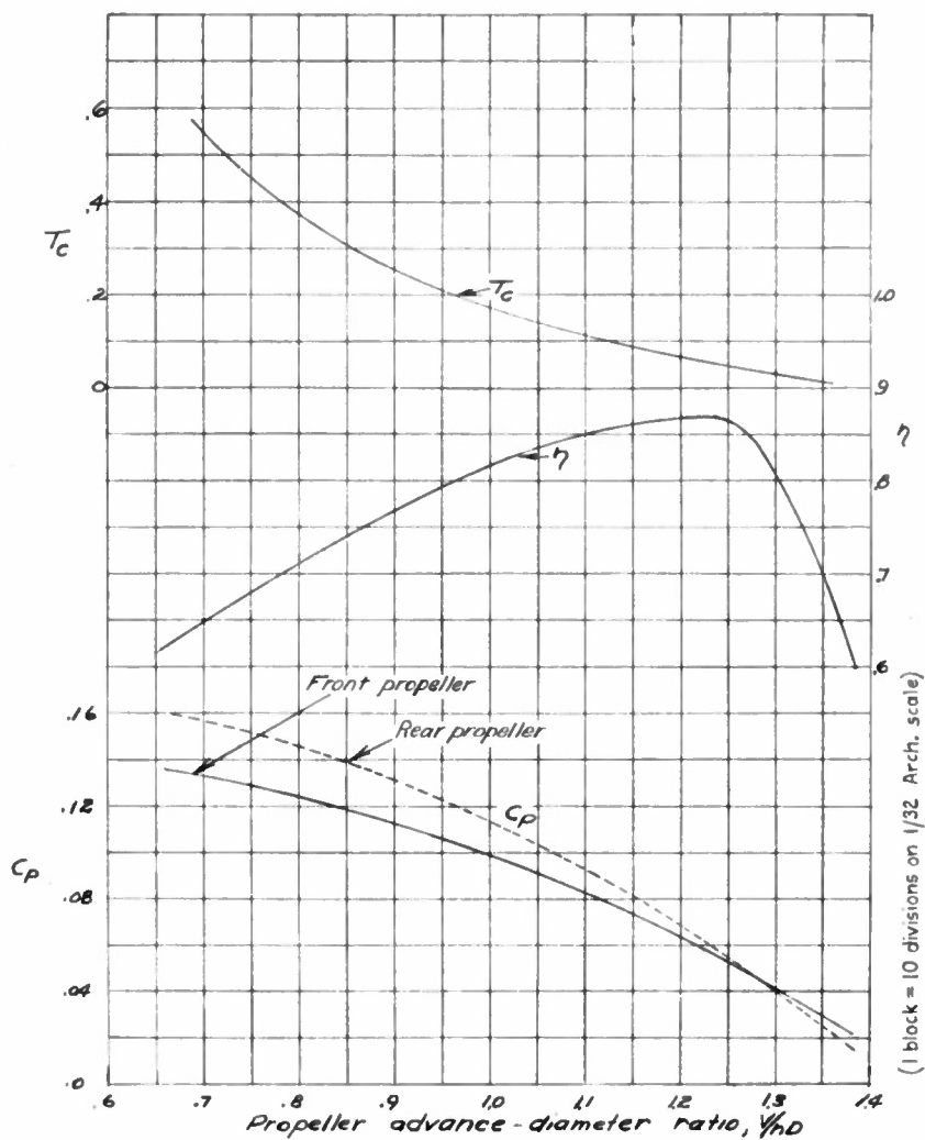
Figure 4.-Propeller characteristics as determined from tests of complete model in the NACA full-scale tunnel. Six-blade dual-rotating propeller; propeller diameter 10 feet; \beta_1 28.0^\circ ; \beta_2 27.7^\circ .
