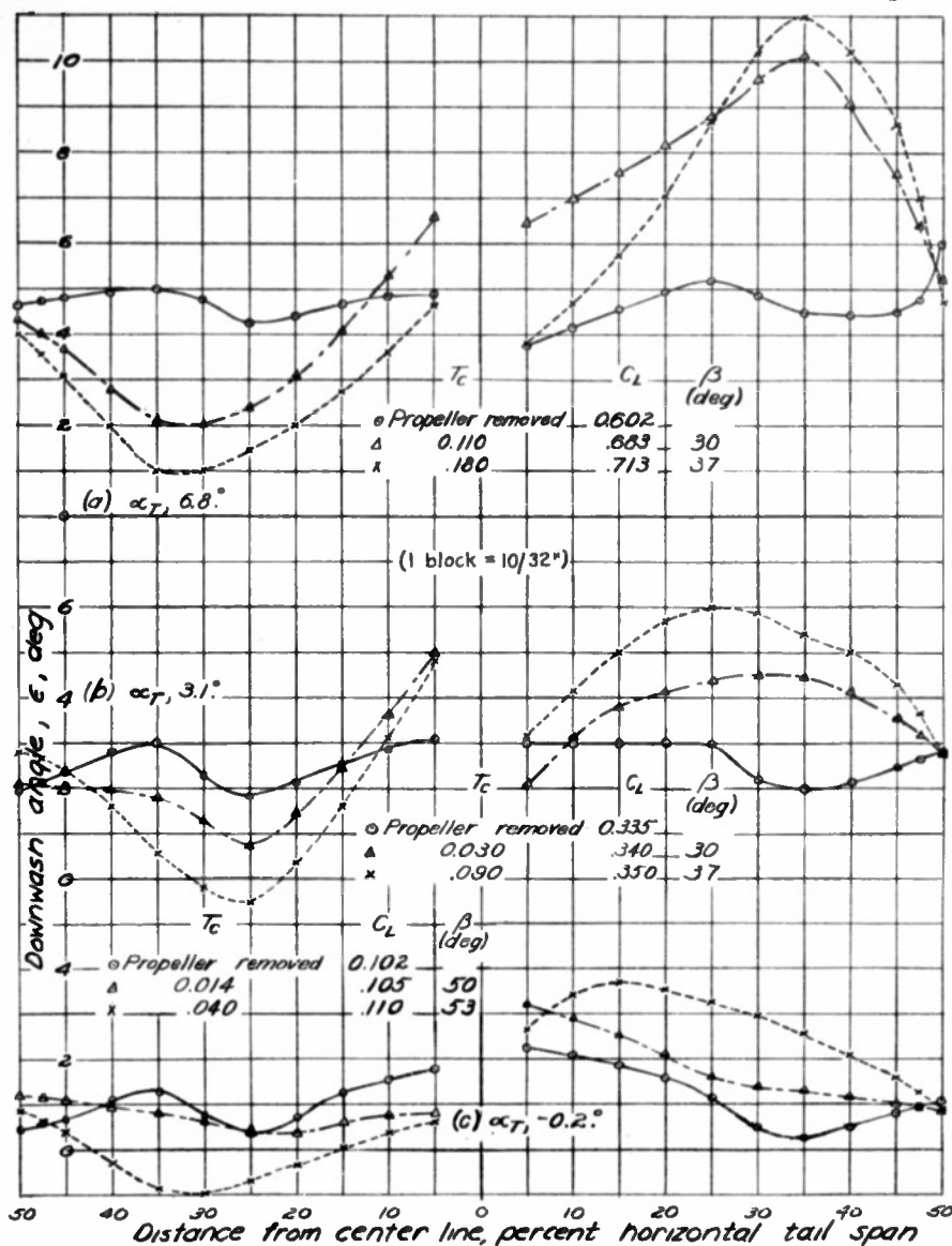
Figure 9.- Variation of downwash angle across the horizontal tail span of model equipped with single-rotating propeller. Values from reference 1. Flaps retracted.
