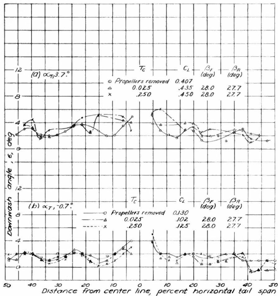
Figure 11.- Variation of downwash angle across the horizontal tail span of model equipped with dual-rotating propellers. Flaps retracted.
