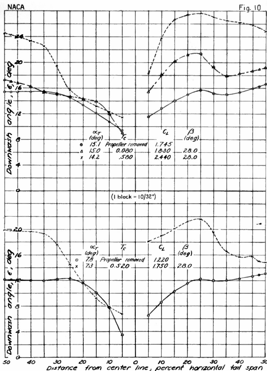
Figure 10.- Variation of downwash angle across the horizontal tail span of model equipped with single-rotating propeller. Values from reference 1. Flaps deflected 40.
