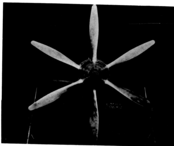
Figure 3.- Propeller installation on model
