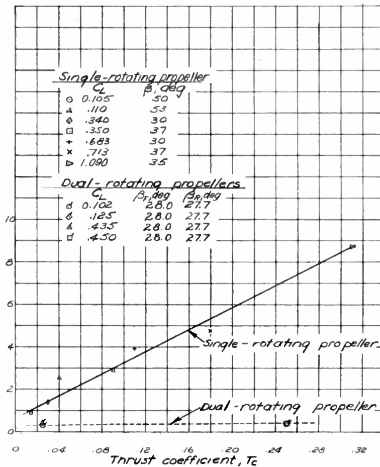
Figure 13.- Comparison of downwash differences across semispans of the horizontal tail surfaces of the model with single-rotating propeller and model with dual-rotating propellers. Flaps retracted.
