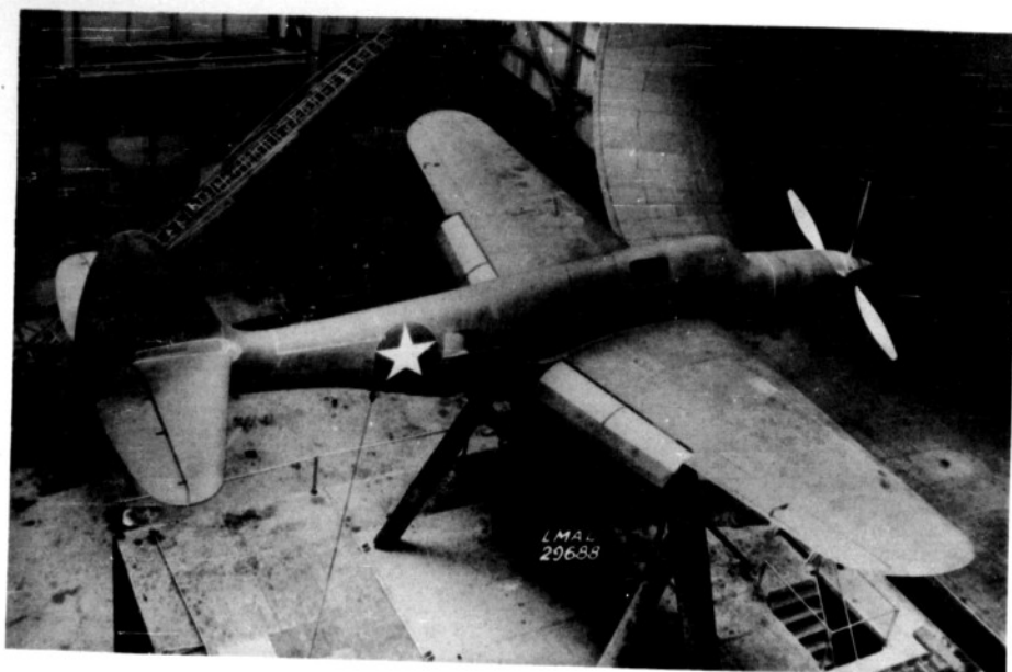
Figure 1.- Model mounted in the NACA full-scale tunnel.
