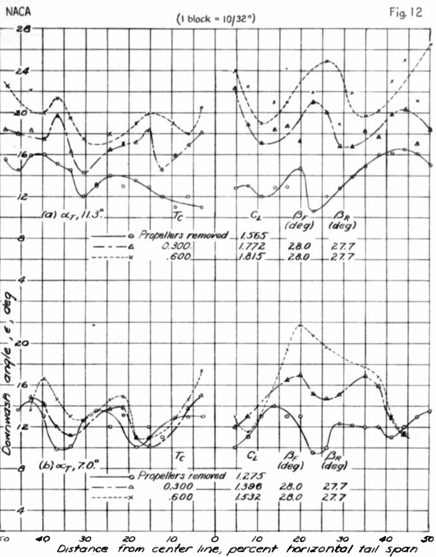
Figure 12-Variation of downwash angle across the horizontal tail span of model equipped with dual-rotating propellers. Flaps deflected 40^\circ .
