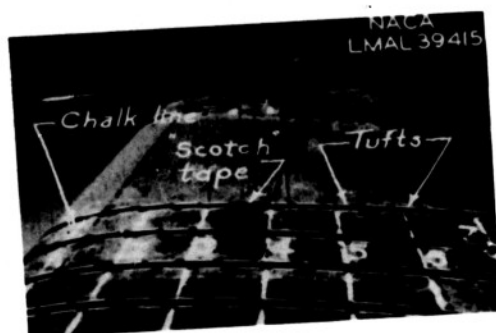
Figure 3.- Test panel on right wing of Republic P-47D airplane, showing rows of tufts at 39.5, 43.5, 48, and 52.5 percent semispan. Numbers identify spanwise lines at intervals of 10 percent chord.
