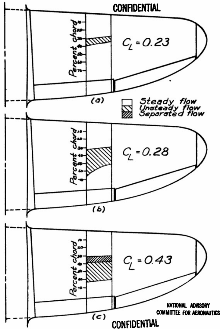
Figure 6.- Flow conditions at test section for an airplane Mach number of 0.71.
