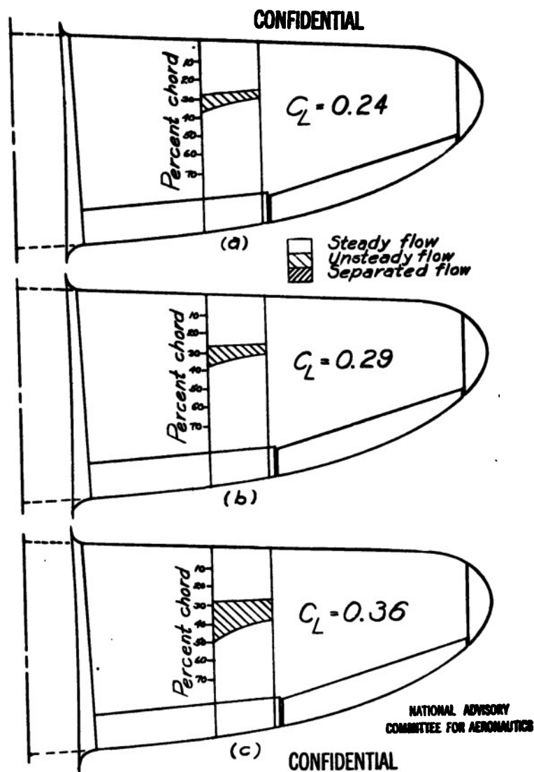
Figure 5.- Flow conditions at test section for an airplane Mach number of 0.69.
