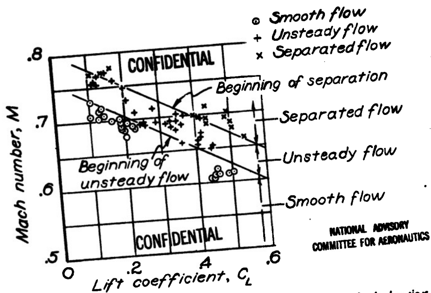
Figure 9.- Flow conditions indicated by tuft behavior.
