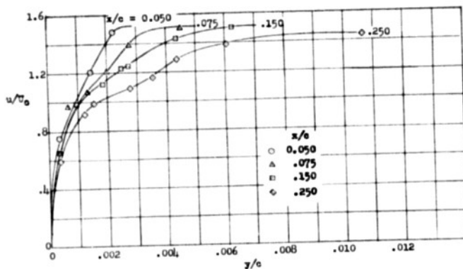
Figure 1. - Boundary-layer velocity profiles in the region forward of the 55-percent-chord station. Airfoil section, NACA 65(216)-222 (approx.); \alpha, 8.1^\circ .
