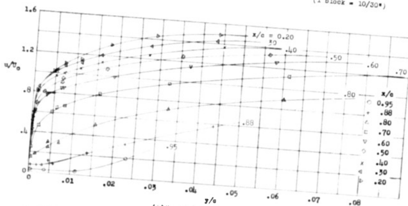
Figure 7. - Boundary-layer velocity profiles in the region from the 20-percent-chord to the 95-percent-chord stations. Nose-opening airfoil shape 15; \alpha , 9.1°.
