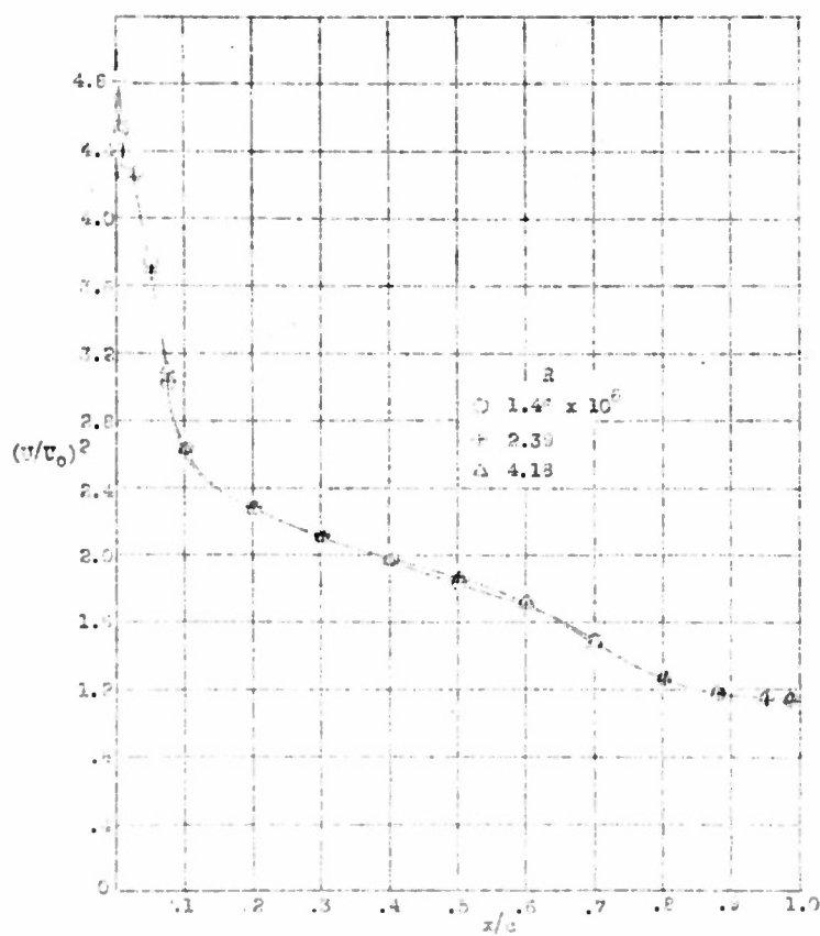
Figure 8.- Upper-surface pressure distributions for several Reynolds numbers. Nose-opening airfoil shape 17:0, 0.19
