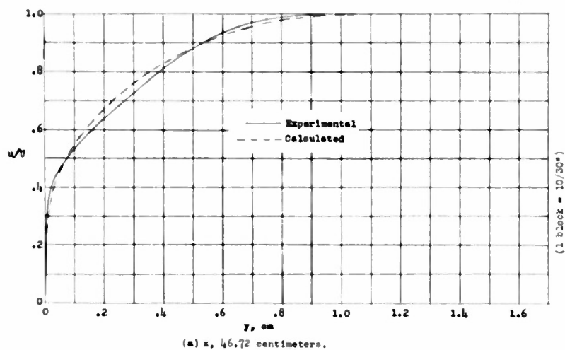
Figure 16. - Comparison of experimental and calculated velocity profiles. (Data from reference 7, run 2.)
