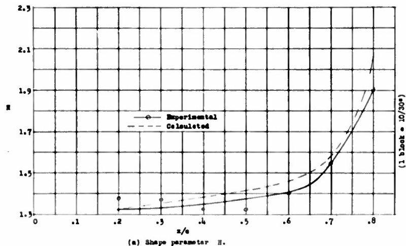
Figure 20. - Variation of experimental and calculated values of shape parameter, H and momentum thickness \theta/c with x/c . NACA airfoil shape 15; R, 4.18 \times 10^6 ; \alpha, 9.1^\circ .
