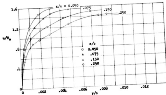
Figure 3. - Boundary-layer velocity profiles in the region forward of the 35-percent-chord station. Airfoil section, NACA 65(216)-222 (approx.); \alpha, 10.1^\circ .
