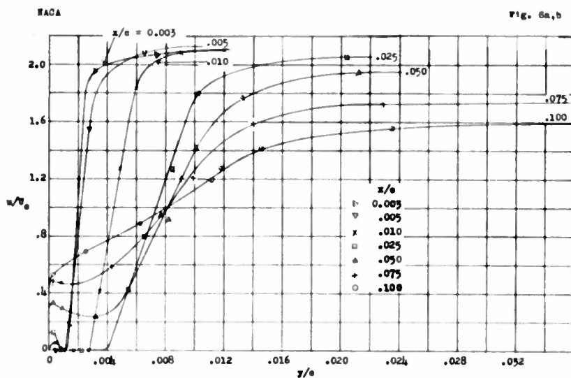
Figure 6. - Boundary-layer velocity profiles in the region forward of the 10-percent-chord station. Nose-opening airfoil shape 13; \alpha, 9.1^\circ .
