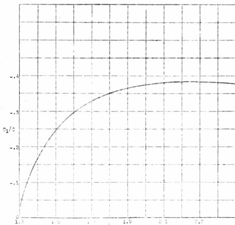
Figure 25.- Approximate determining rate of pressure recovery for pressure distribution designed to hold a constant R .
