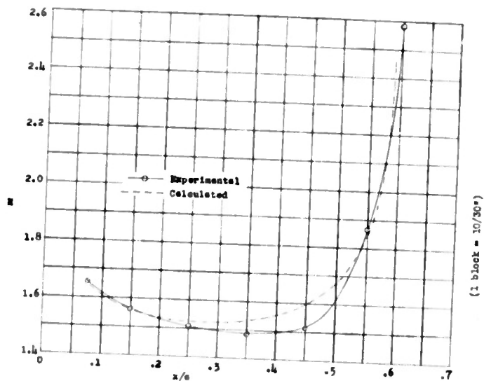
Figure 23. - Variation of experimental and calculated values of shape parameter H and momentum thickness \theta/c with x/c . Airfoil section, NACA 65(216)-222 (approx.); R , 2.67 \times 10^6 ; \alpha , 0.10^\circ .
