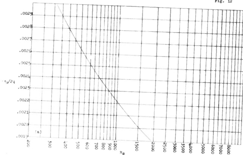
Figure 12. - Variation of v/2q with Re (reference 14).
