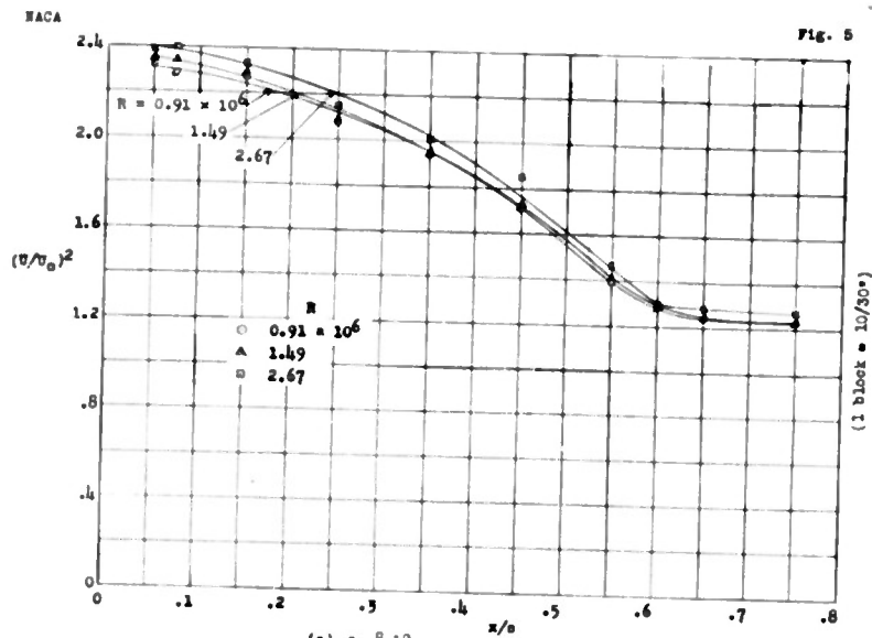
Figure 5. - Upper-surface pressure distributions for several Reynolds numbers. Airfoil section, NACA 65(216)-222 (approx.).
