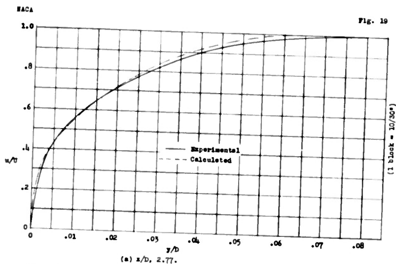
Figure 19. - Comparison of experimental and calculated velocity profiles for the elliptic cylinder. R , based on minor axis, 118,000. (Data from reference 11.)
