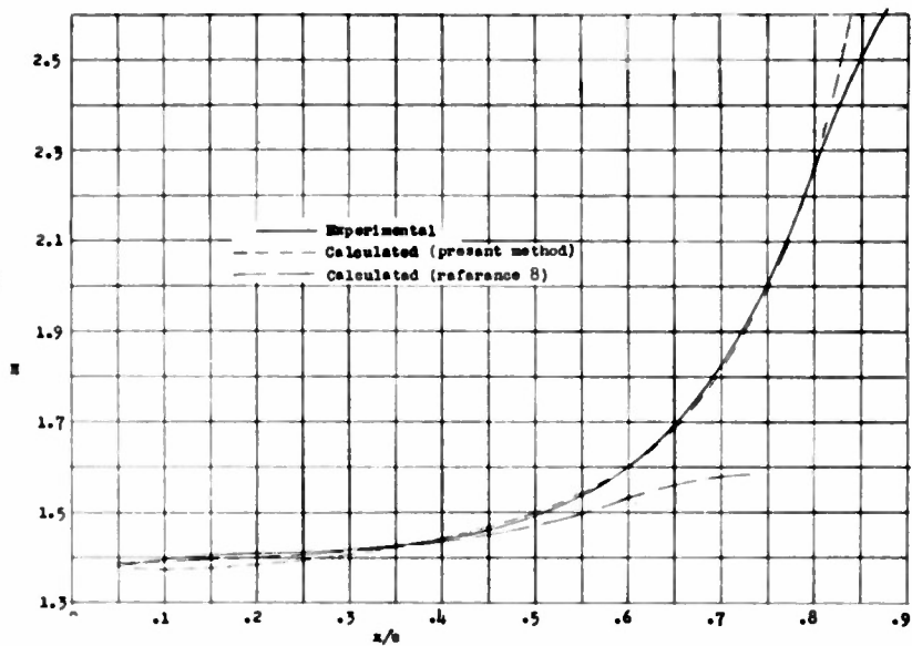
Figure 17. - Variation of experimental and calculated values of shape parameter H and momentum thickness \theta/c with x/c for symmetrical airfoil. R, 3.8 \times 10^6 ; \alpha, 9^\circ . (Data from reference 8.)
