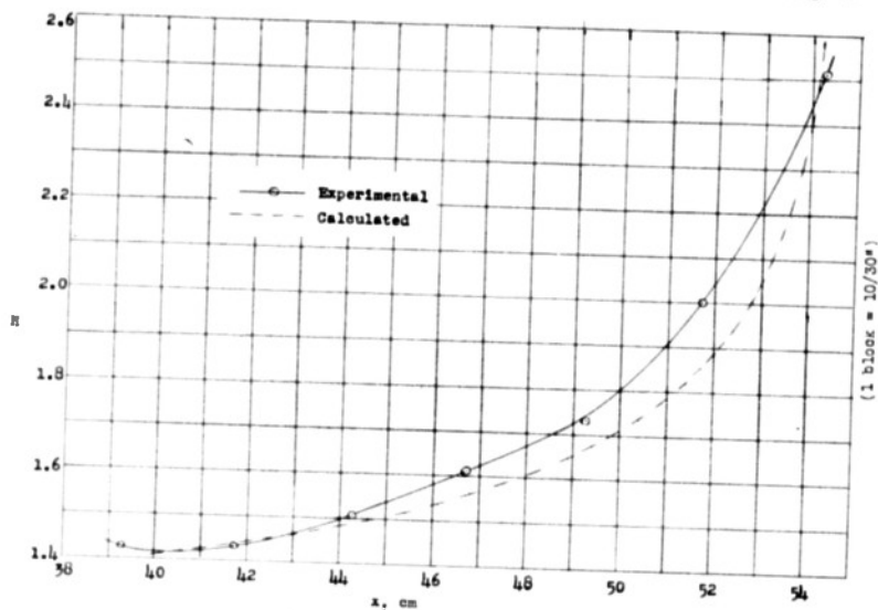
Figure 15. - Variation of experimental and calculated values of shape parameter H and momentum thickness \theta with x for flow in a channel. (Data from reference 7, run 2.)
