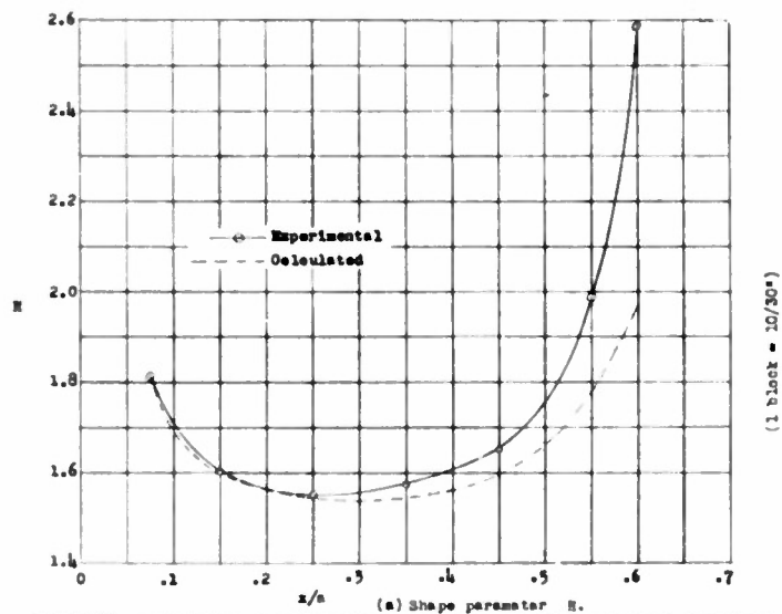
Figure 22. - Variation of experimental and calculated values of shape parameter H and momentum thickness \theta/c with x/c . Airfoil section, NACA 65(216)-222 (approx.); H , 0.92 \pm 10\% ; \alpha , 6.1^\circ .
