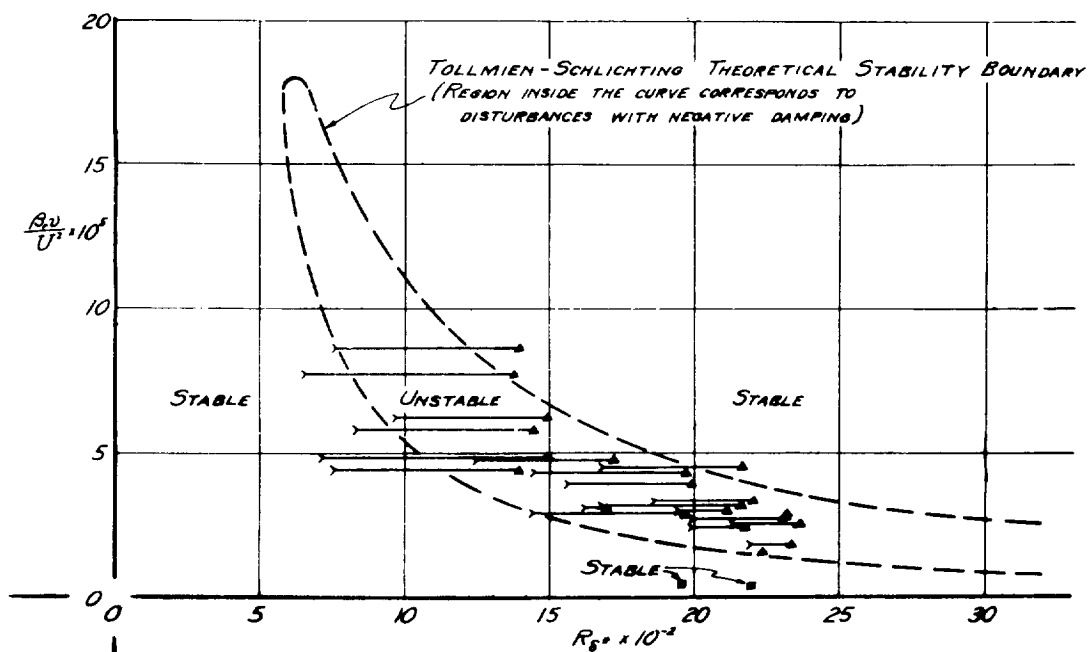
Figure 17.- Frequencies of the boundary layer oscillations excited by the wire lattice compared with the theoretical instability limit. The horizontal lines denote the path of the amplified waves from the lattice to the beginning of transition.
