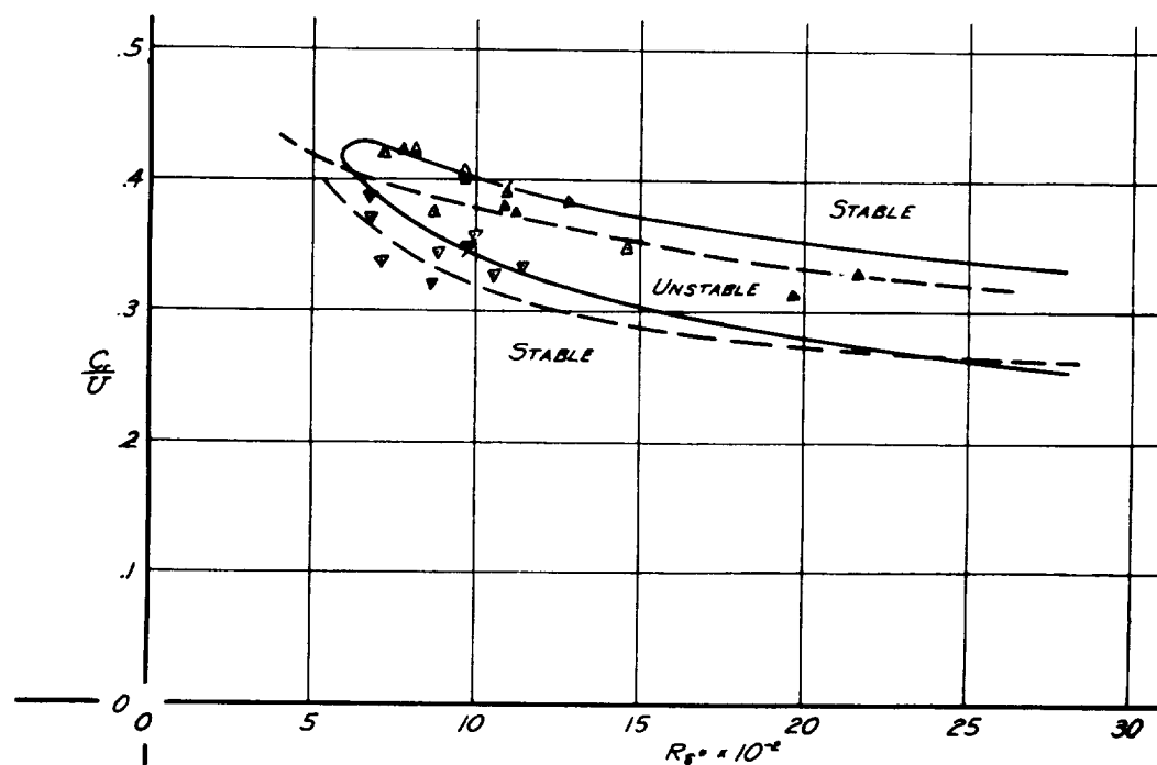
Figure 22.- The experimental stability limit of the laminar boundary layer oscillation on the convex side of the r = 20' plate as compared with the theoretical stability limit. Phase velocity diagram.
