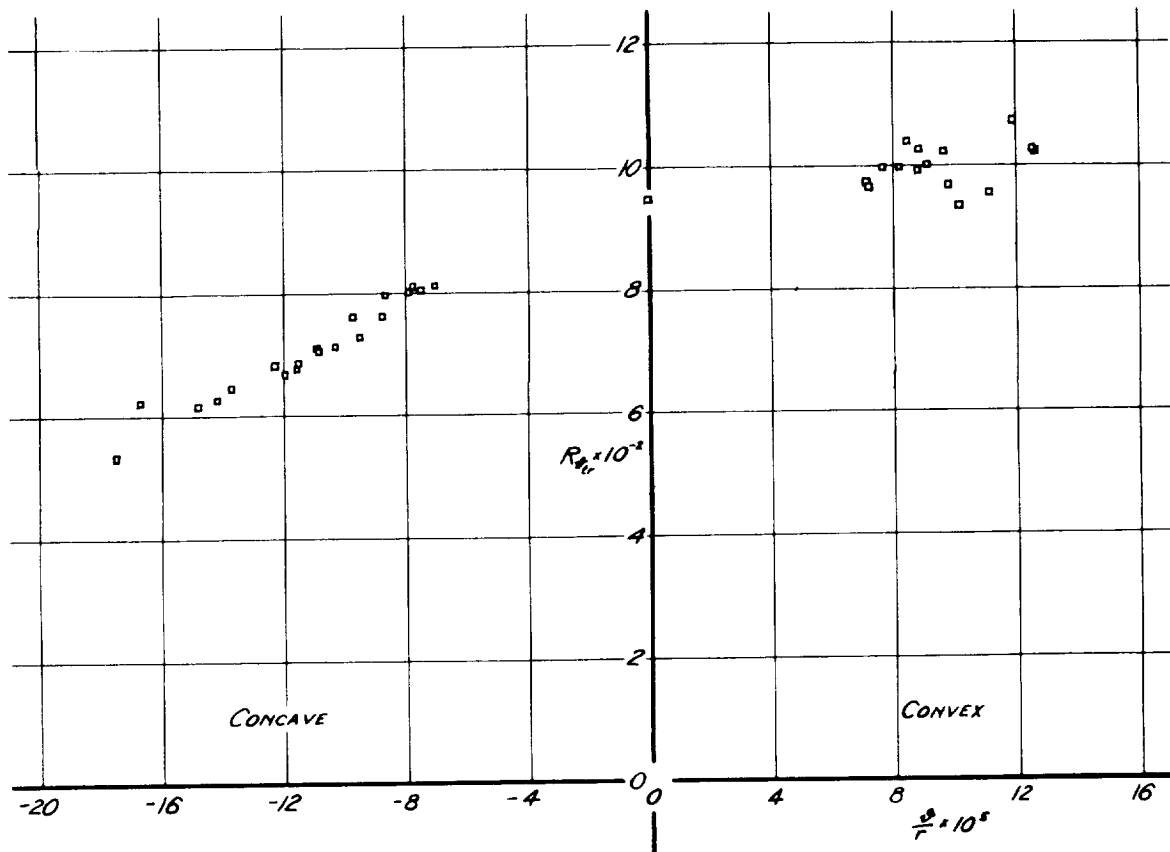
Figure 11.- Effect of curvature on the Reynolds number of transition. Results of measurements on the flat plate and r = 20' plate are shown.
