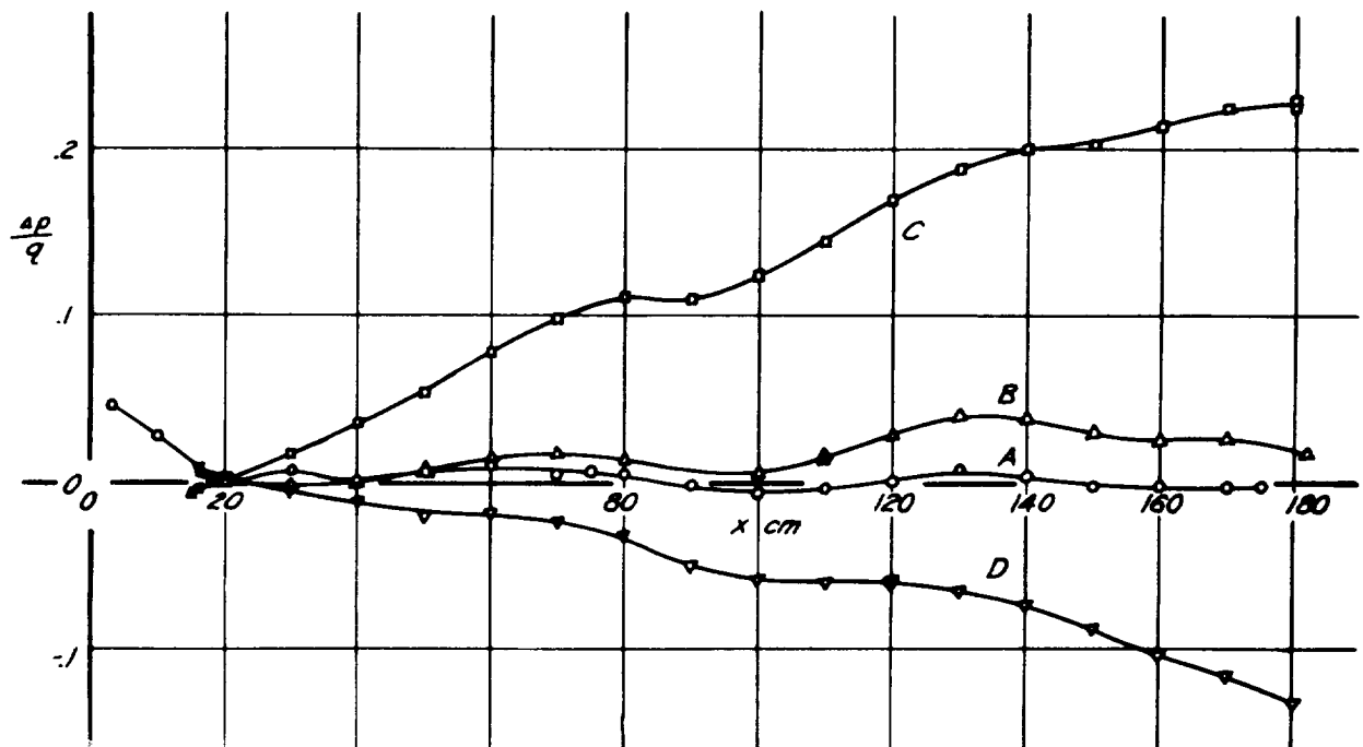
Figure 31.- Pressure gradients for which transition was investigated along the convex side of the r = 20' plate.
