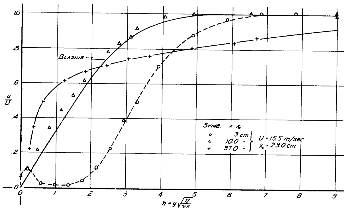
Figure 28.- Velocity profiles downstream from a single roughness element situated at a distance x_0 from the leading edge. Transition occurs after the boundary layer has become reattached to the wall.
