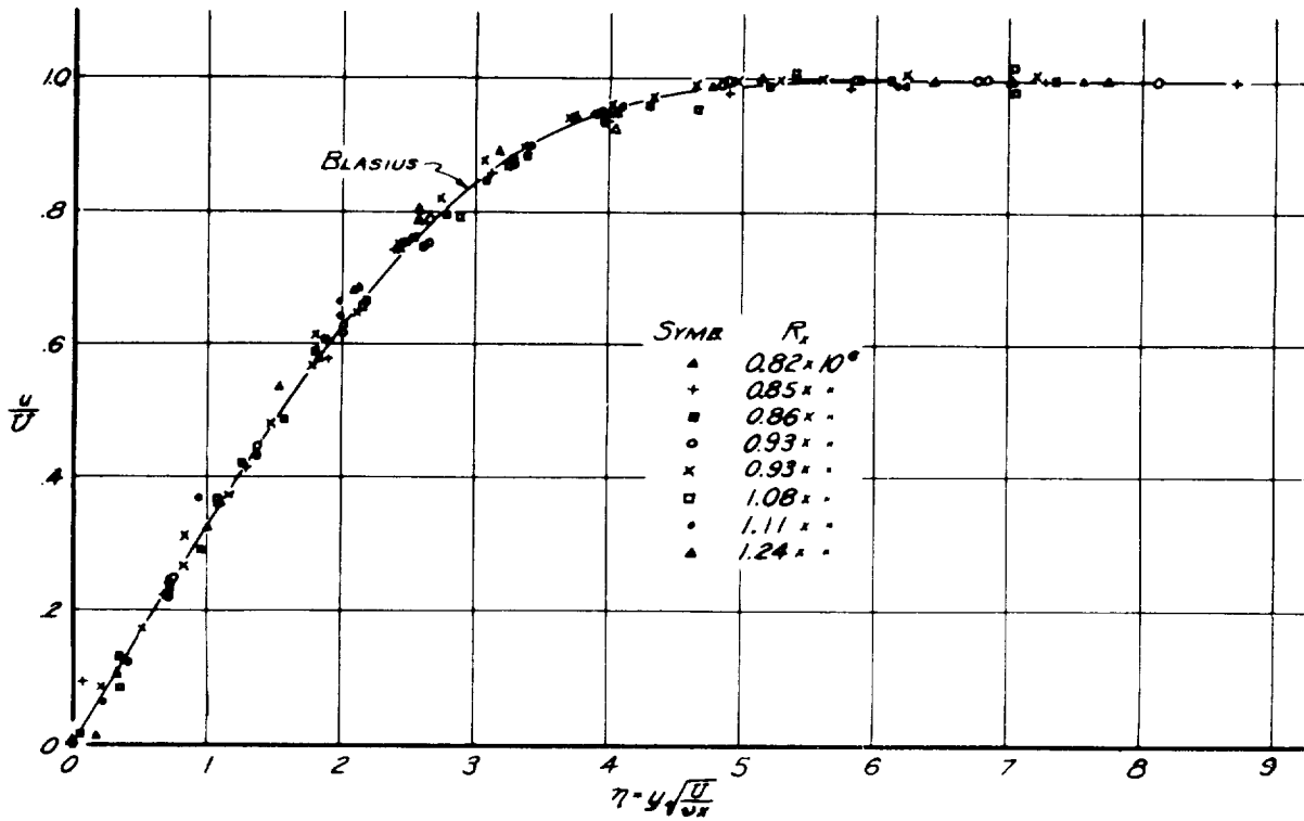
Figure 6.-Velocity distribution in the laminar boundary layer of the flat plate.
