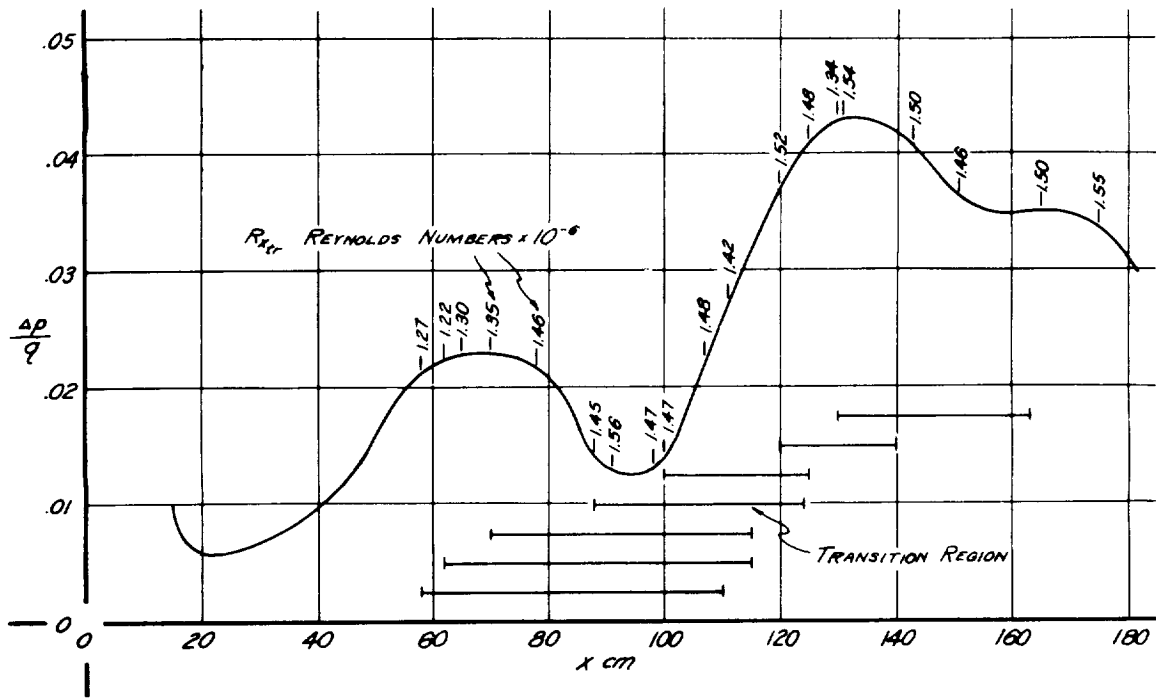
Figure 32.- Reynolds numbers of transition with pressure gradient B. Note change in scale as compared with Fig. 31.
