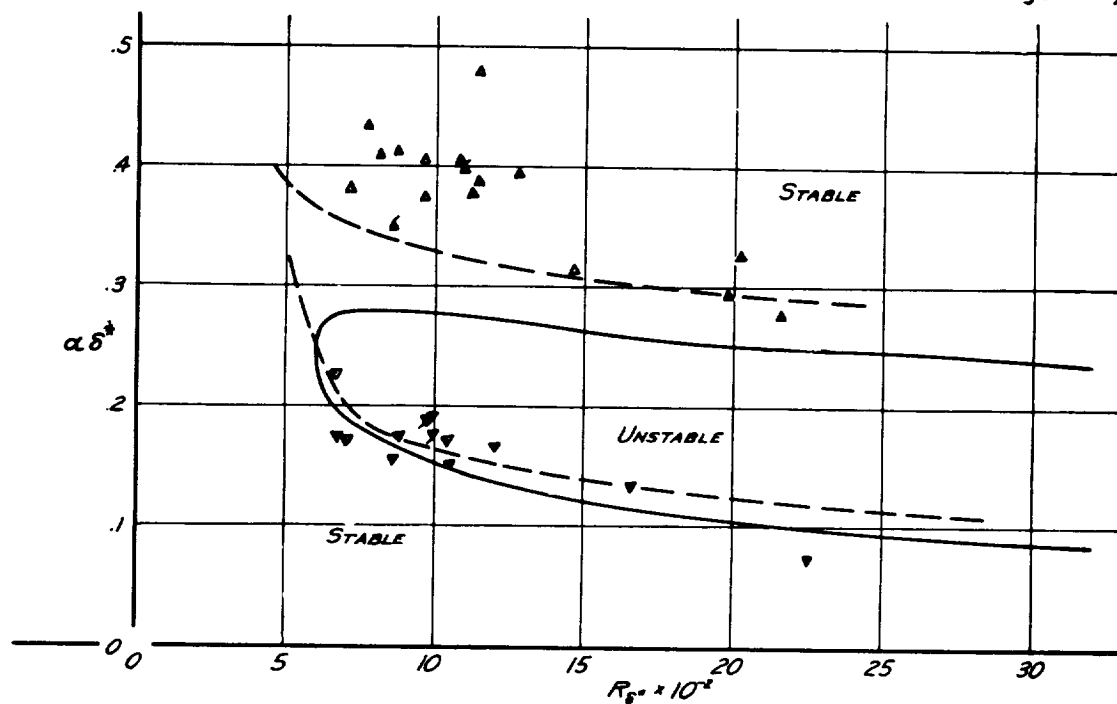
Figure 21.- The experimental stability limit of the laminar boundary layer oscillation on the convex side of the r = 20' plate as compared with the theoretical stability limit. Wave length diagram.
