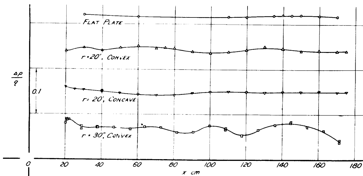
Figure 5.- Pressure distributions along the test plates for "zero" gradient.
