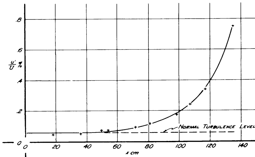
Figure 12.- Increase of turbulence level along convex side of r = 30'' plate due to the spread of turbulence from the opposite wall.
