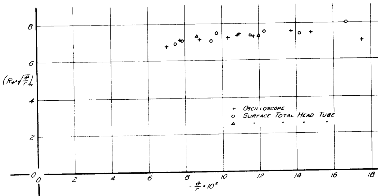
Figure 26.- The critical parameter (Re \sqrt{\frac{\gamma}{r}}) at the transition point as function of \frac{\gamma}{r} for the concave side of the r = 20 " plate.
