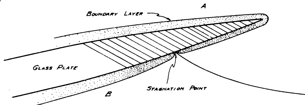
Figure 36.- Schematic diagram showing the angle of attack effect.
