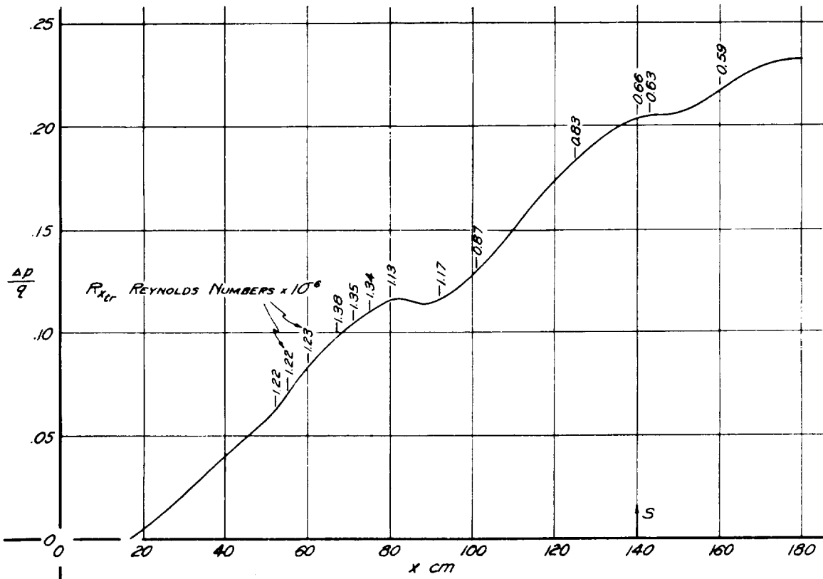
Figure 33.- Reynolds number of transition with pressure gradient C. Note change in scale as compared with Fig. 31. S denoted the computed separation point.
