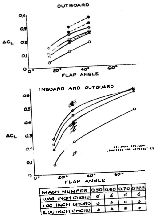
FIGURE 13.-EFFECT OF OUTBOARD AND INBOARD-OUTBOARD FLAPS AT 33% CHORD ON LIFT COEFFICIENT FOR \alpha = 1^\circ .
