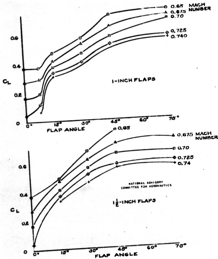
FIGURE 2.-EFFECT OF FLAP ANGLE ON THE C_L AT BALANCE, ELEVATOR AND STABILIZER AT 0°, FLAPS INBOARD AT 33% CHORD.
