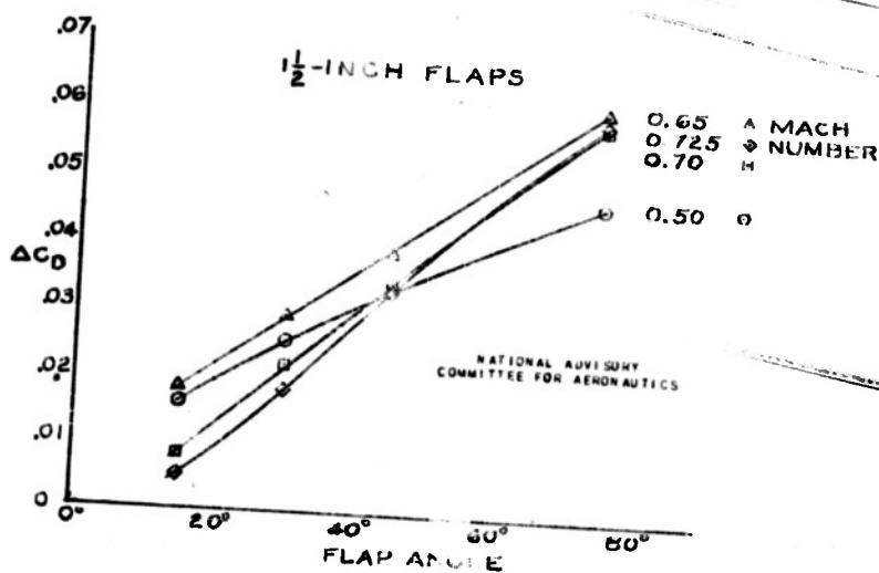
FIGURE 4.-EFFECT OF INBOARD FLAPS AT 33% CHORD ON DRAG COEFFICIENT FOR C_L=0.15 .
