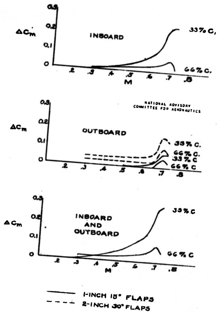
FIGURE 5.-EFFECT OF CHORD POSITION OF FLAPS ON MOMENT COEFFICIENT.
