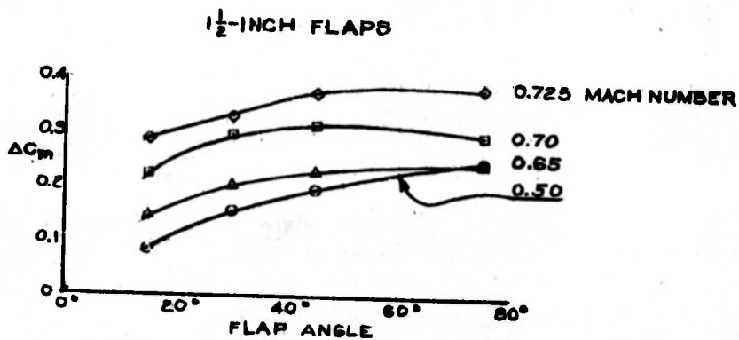
FIGURE 8 - EFFECT OF INBOARD FLAPS AT 39% CHORD ON MOMENT COEFFICIENT FOR C_L = 0.15 .
