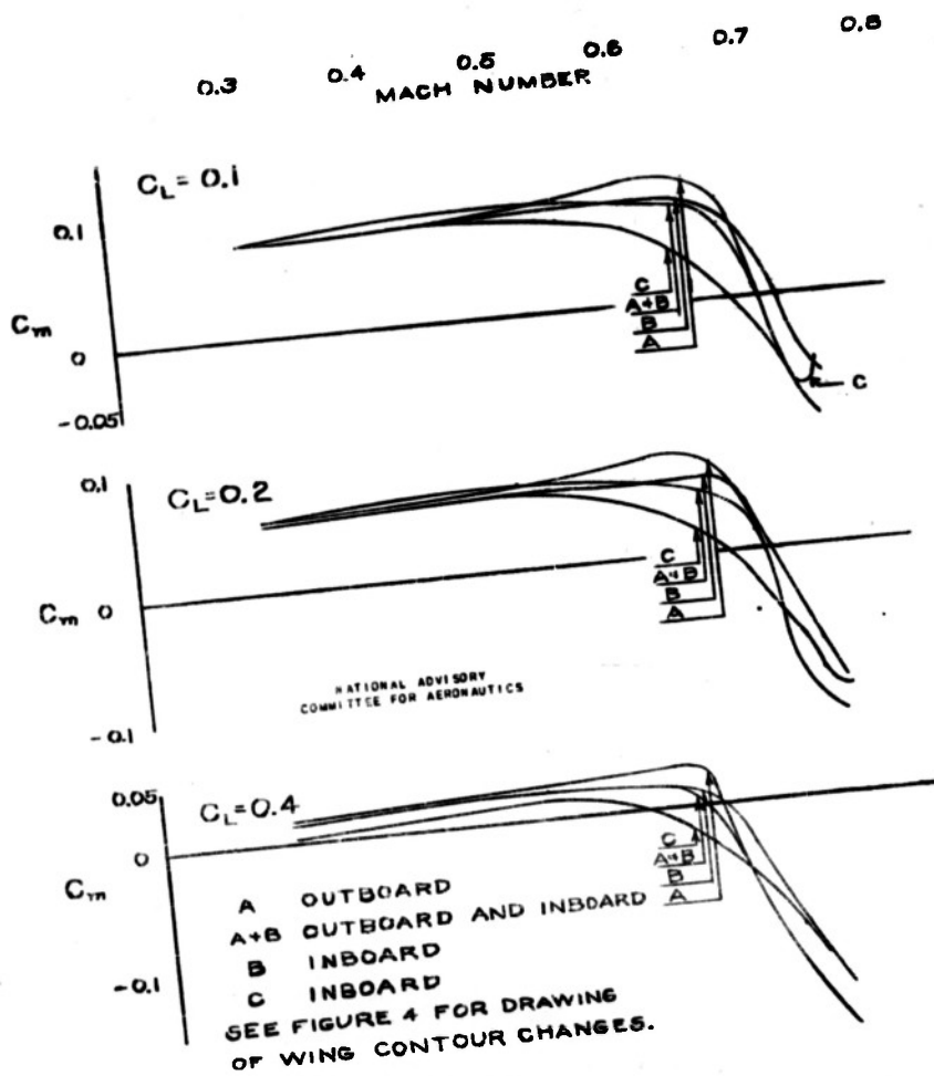
FIGURE 16.-EFFECT OF CHANGING UPPER SURFACE WING CONTOURS ON MOMENT COEFFICIENT.
