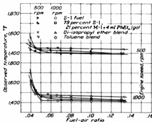
FIGURE 14.—Ignition of four 100-octane fuels. Compression ratio, 7.0; engine-coolant temperature, 250° F; ignition by heated roll.
