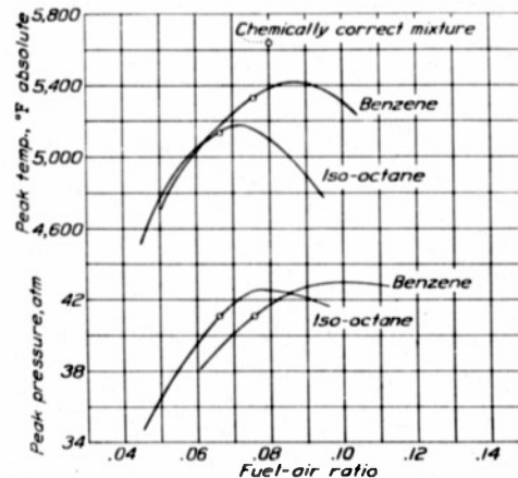
FIGURE 20.—Effect of fuel-air ratio on estimated peak temperatures and peak pressures. Compression ratio, 5; initial temperature, 112° F; initial pressure, 1.0 atmosphere. Data from reference 15.
