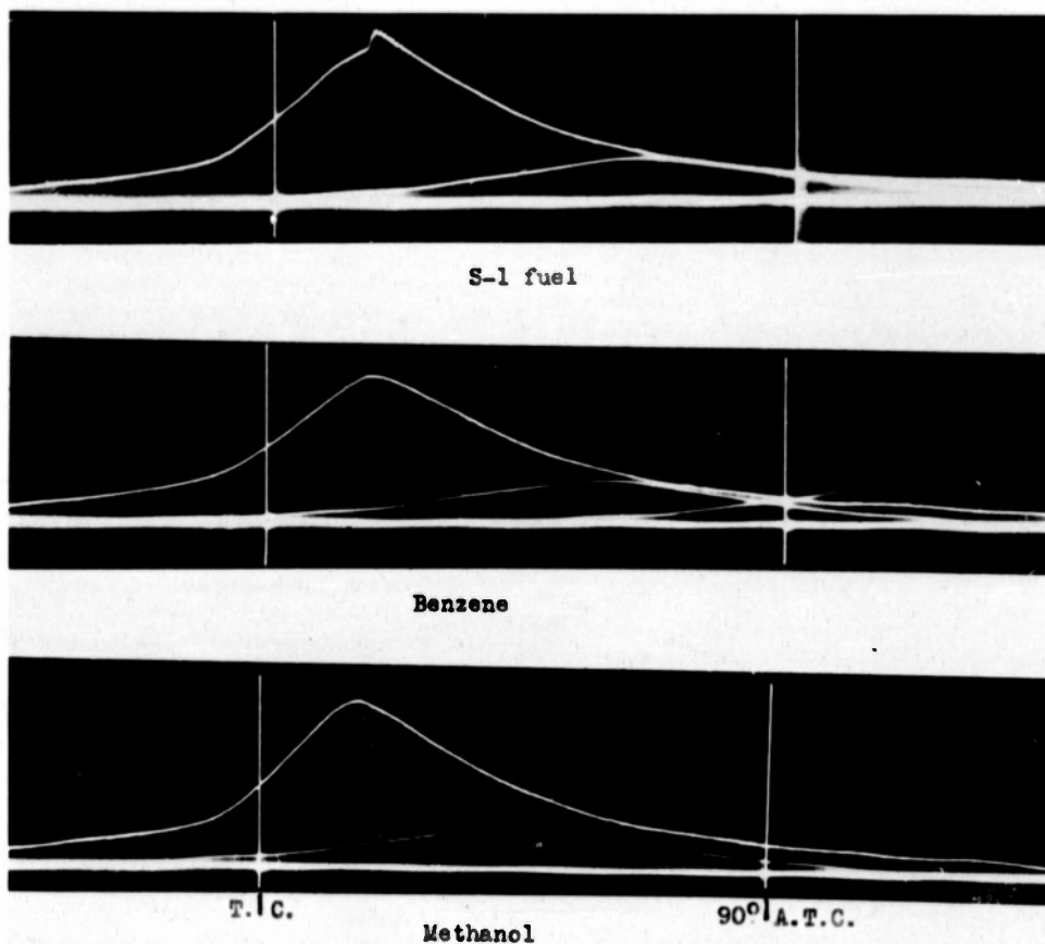
FIGURE 6.—Indicator cards for three fuels. Compression ratio, 7.0; engine-coolant temperature, 310° F; engine speed, 500 rpm; spark advance, 30°; one spark plug. Mixture ratio for complete combustion.
