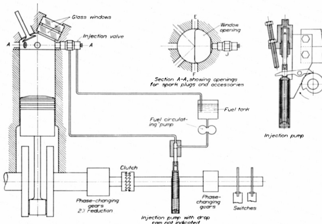
FIGURE 1.—Diagram of combustion apparatus.
