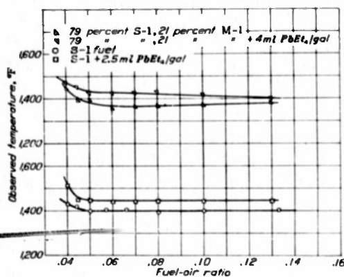
FIGURE 13.—Ignition of two fuels with and without addition of tetraethyl lead. Compression ratio, 7.0; engine-coolant temperature, 250° F; engine speed, 500 rpm; ignition by heated roll.
