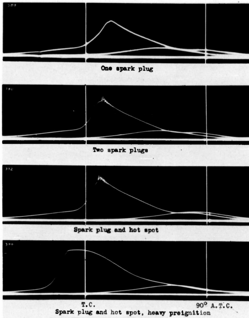
FIGURE 6.—Knock induced by hot spot and by use of two spark plugs. Compression ratio, 7.0; engine coolant temperature, 250° F; engine speed, 500 rpm; spark advances, 10°; fuel, 85 percent 8-1, 15 percent M-1.
