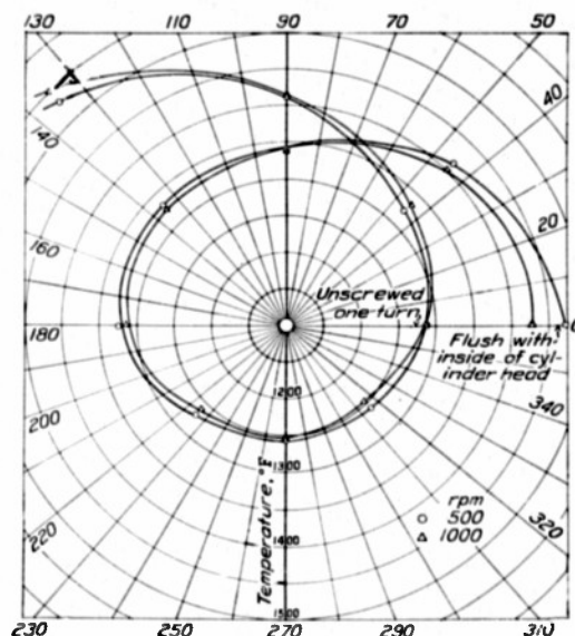
FIGURE 2.—Ignition points of benzene for different heated-coil positions. Compression ratio, 7.0; engine-coolant temperature, 250° F; thread pitch of fitting, 1.5 millimeters.
