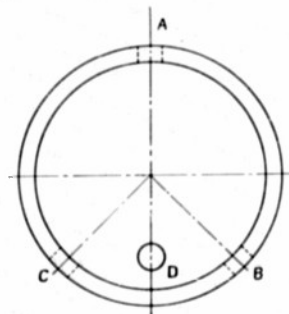
FIGURE 2.—Location of spark-plug holes in C. F. R. engine.
