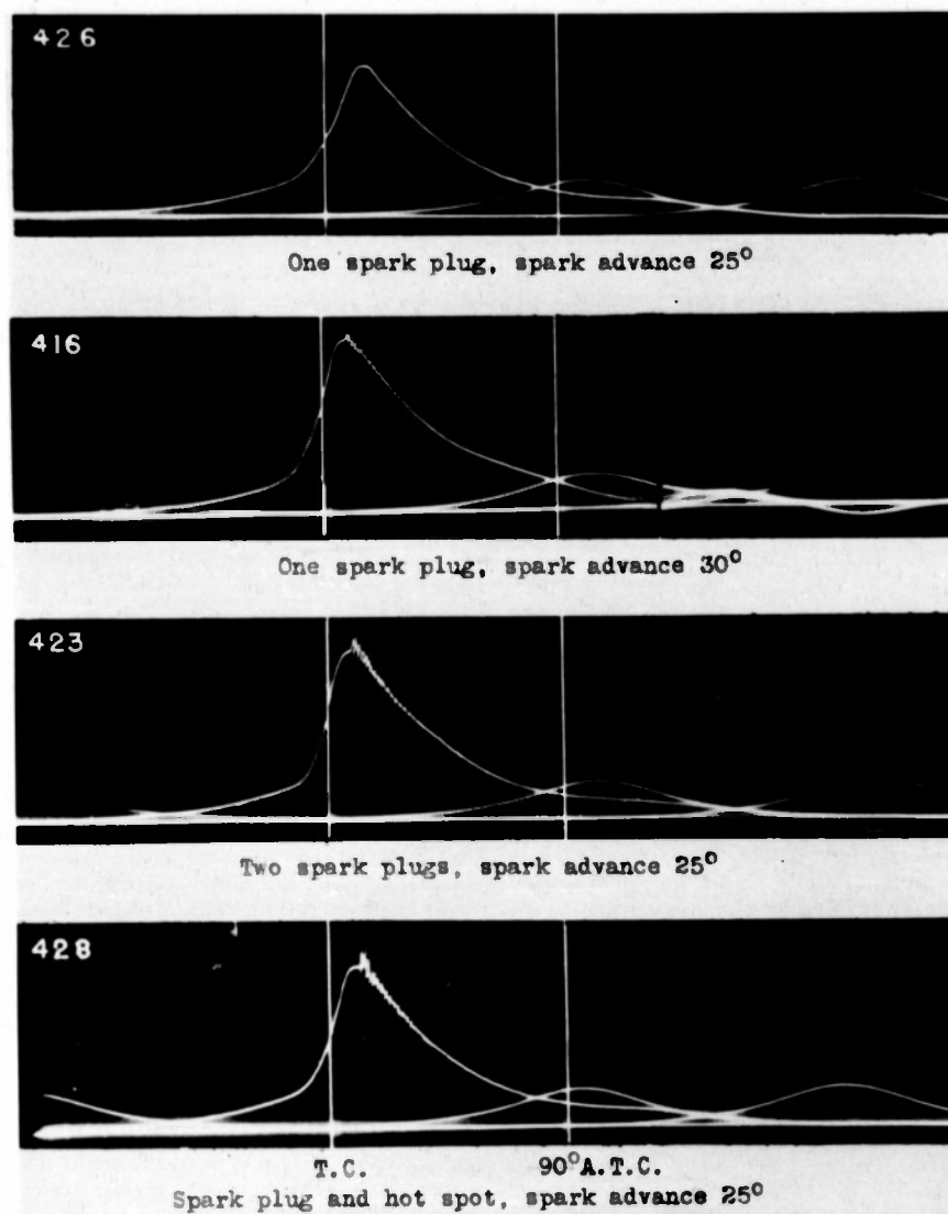
FIGURE 7.—Knock induced by hot spot, by use of two spark plugs, or by advancing the spark. Compression ratio, 7.0; engine-coolant temperature, 250^\circ F; engine speed, 1,000 rpm; fuel, 85 percent S-1, 15 percent M-1.
