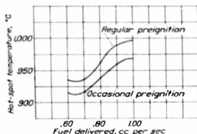
FIGURE 16.—Effect of mixture strength. Coolant-outlet temperature, 60° C; engine speed, 1,250 rpm. Data from reference 5.
