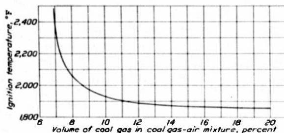
FIGURE 17.—Ignition of coal gas-air mixtures by hot moving pellet. Platinum pellet, 2 millimeters in diameter; velocity, 21 meters per second. Chemically correct mixture, 21 percent. Data from reference 10.
