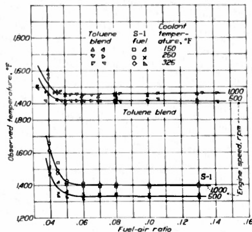
FIGURE 11.—Effect of engine-coolant temperature on ignition of toluene blend and S-1 fuel. Compression ratio, 9.5; ignition by heated coil.
