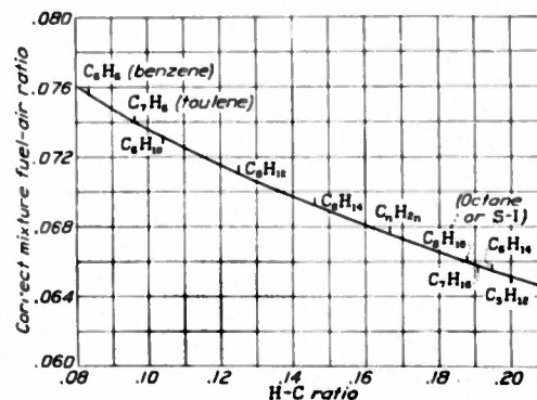
FIGURE 15.—Fuel-air ratios for complete combustion of several hydrocarbons.
