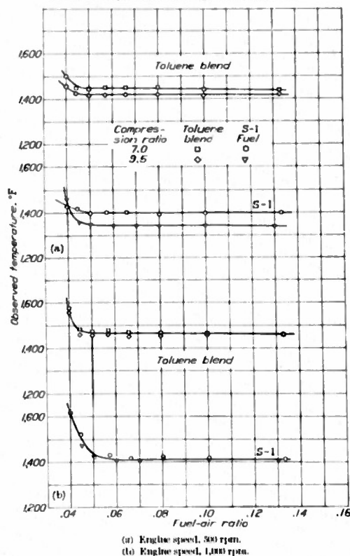
FIGURE 12.—Effect of compression ratio on ignition of toluene blend and S-1 fuel. Engine-coolant temperature, 250° F; ignition by heated coil.
