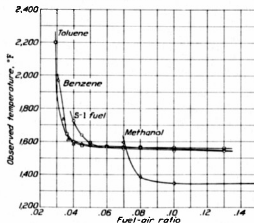
FIGURE 18.—Ignition of four fuels. Compression ratio, 7.0; engine-coolant temperature, 250° F; engine speed, 500 rpm; ignition by hot wire.
