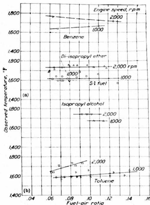
(a) S-1 fuel, benzene, and di-isopropyl ether. (b) Toluene and isopropyl alcohol. FIGURE 19.—Ignition of various fuels in C. F. R. engine.
