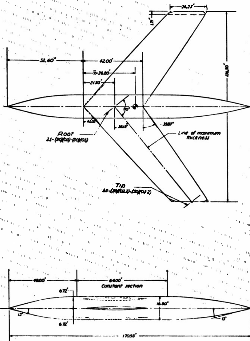
Figure 1.-Sketch of wing and fuselage. Wing area, 4728 sq.in.; mean aerodynamic chord, 35.31 in.; aspect ratio, 3.94.
