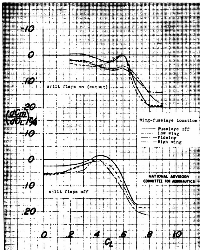
Figure 17.- Variation of (dC_m/dC_L)\epsilon/l with lift coefficient for a 42^\circ swept-back wing for several wing-fuselage arrangements. R = 8.2 \times 10^6 .
