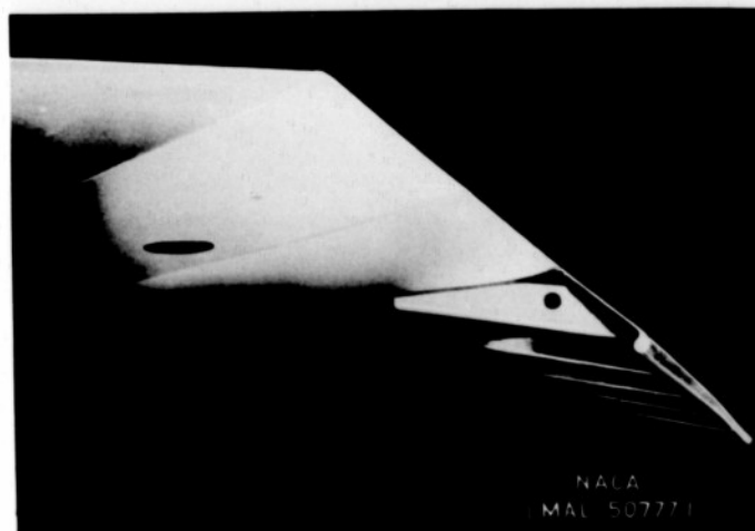
(a) Flat leading-edge flap.
