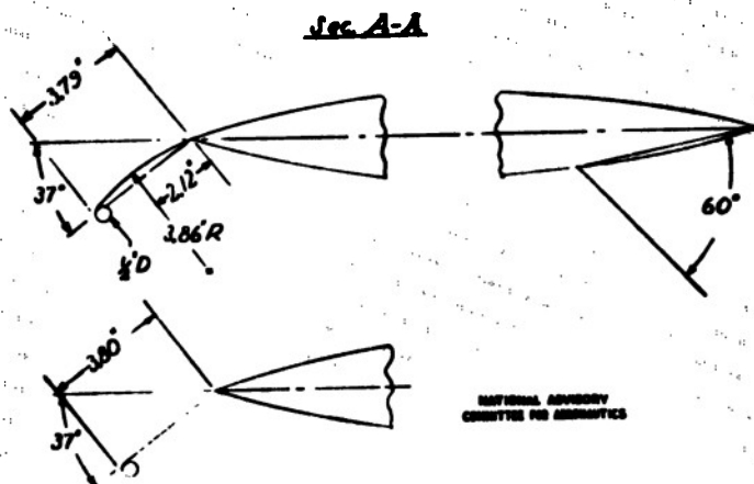
Figure 3 - Schematic drawing of high lift devices for 42° swept-back wing.
