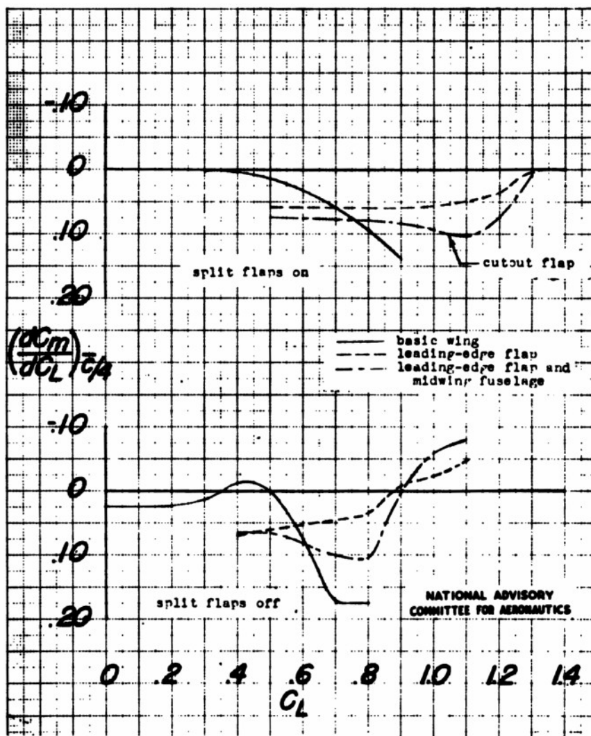
Figure 16.- Variation of (dC_m/dC_L)\pi/l with lift coefficient for a 42^\circ sweptback wing with and without a flat leading-edge flap. R = 5.32 \times 10^6 .
