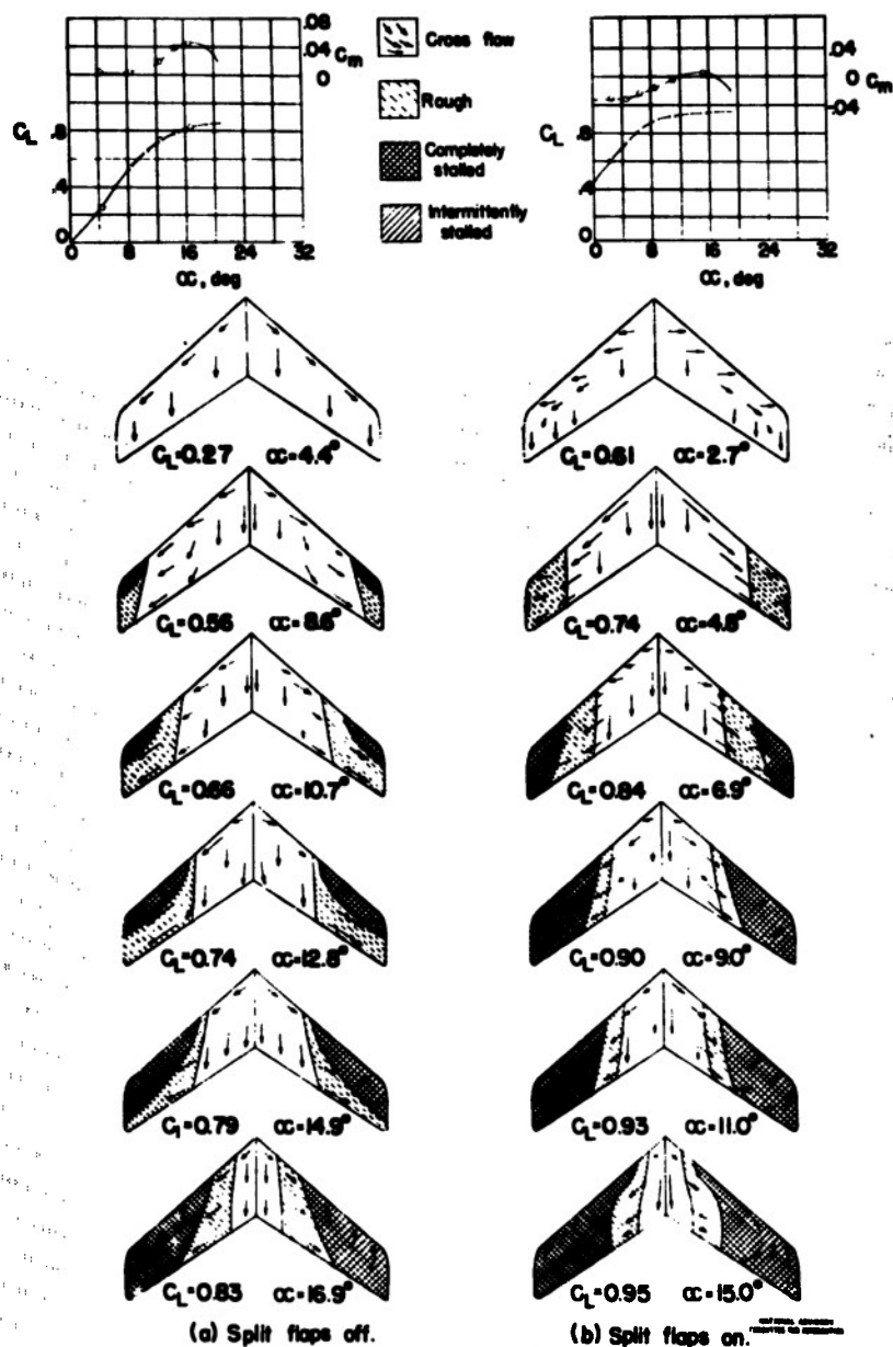
Figure 5.-Stalling characteristics of a 42° sweptback wing. R = 8.20 \times 10^6 .
