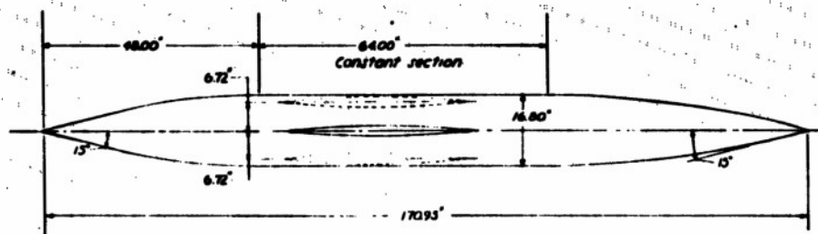
Figure 1-Sketch of wing and fuselage. Wing area, 4728 sq.in.; mean aerodynamic chord, 35.31 in.; aspect ratio, 3.94.
