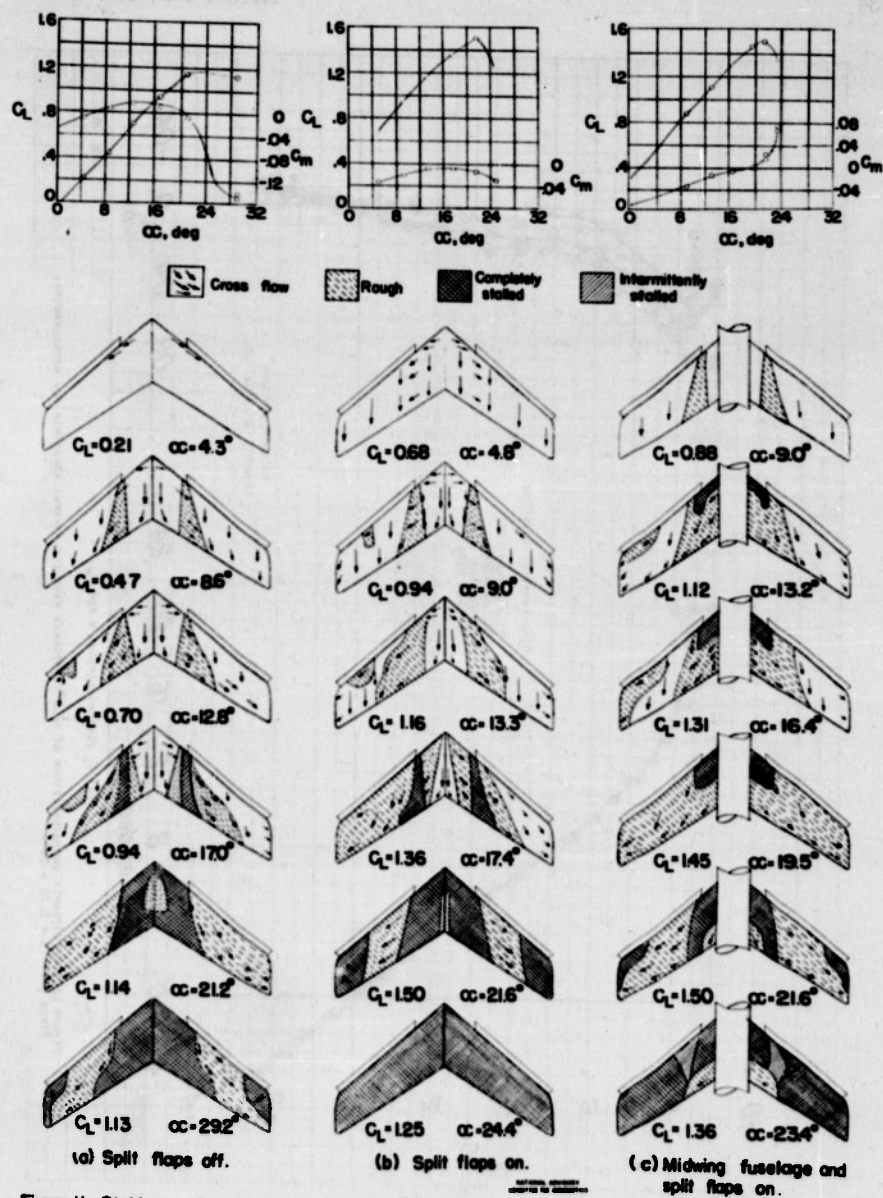
Figure 11.-Stalling characteristics of a 42° sweptback wing with a flat leading-edge flap R=5.32 \times 10^\circ .
